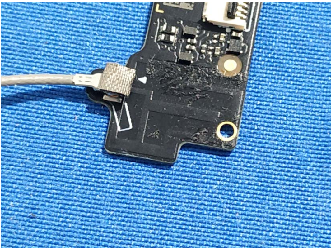
GFSK Antenna-Chain 1
