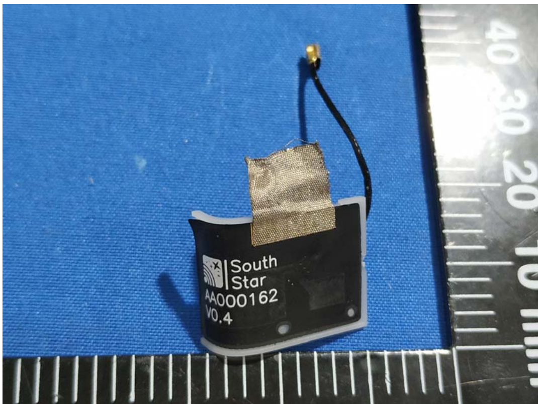
Wi-Fi&BLE Antenna-Chain 1
