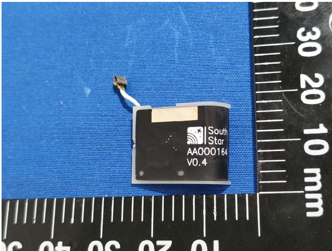
GFSK Antenna-Chain 1
