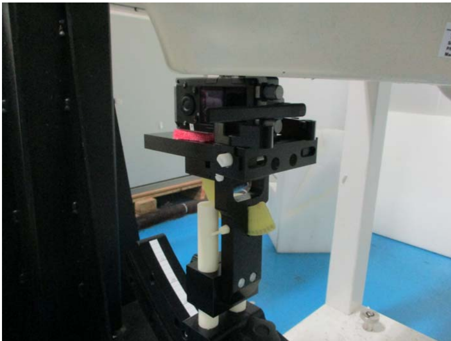
Test Position_Left Antenna Fold (0mm)
