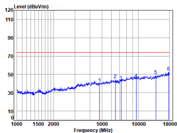
BLE_1M_TX_CH_00_Vertical-Peak
