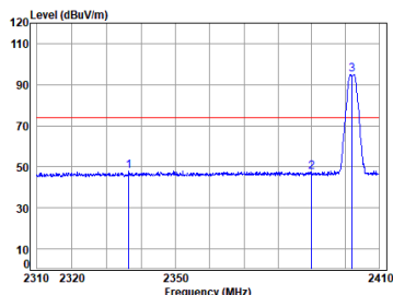
BLE_2M_TX_CH_00_Horizontal-Peak
