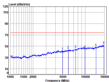
BLE_1M_TX_CH_39_Vertical-Peak
