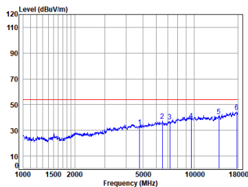
BLE_1M_TX_CH_00_Vertical-Avg
