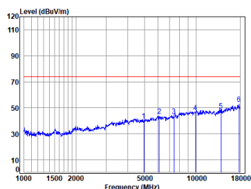
BLE_1M_TX_CH_39_Horizontal-Peak
