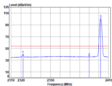
BLE_1M_TX_CH_00_Vertical-Avg
