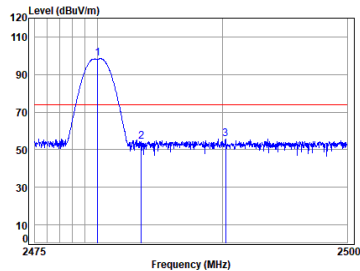
BLE_1M_TX_CH_39_Vertical-Peak
