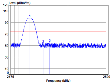
BLE_1M_TX_CH_39_Horizontal-Peak
