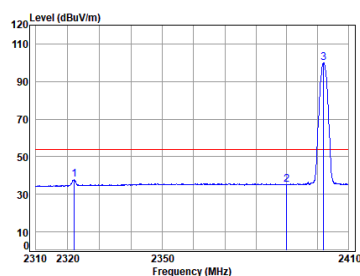
BLE_1M_TX_CH_00_Horizontal-Avg
