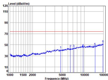
BLE_2M_TX_CH_00_Vertical-Peak
