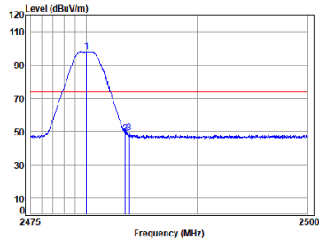
BLE_2M_TX_CH_39_Horizontal-Peak
