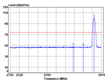
BLE_1M_TX_CH_00_Horizontal-Peak
