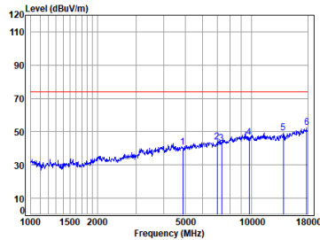
BLE_2M_TX_CH_19_Horizontal-Peak
