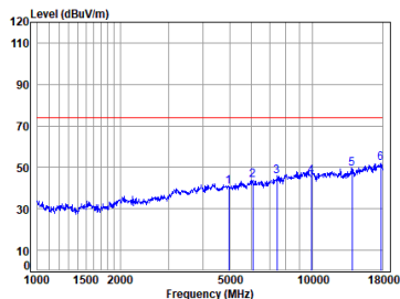
BLE_2M_TX_CH_39_Vertical-Peak
