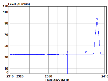
BLE_2M_TX_CH_00_Horizontal-Avg
