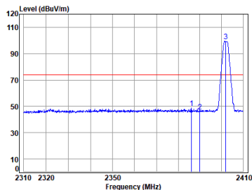
BLE_2M_TX_CH_00_Vertical-Peak
