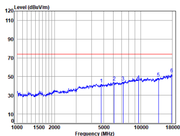
BLE_1M_TX_CH_00_Horizontal-Peak
