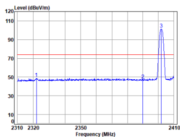
BLE_1M_TX_CH_00_Vertical-Peak
