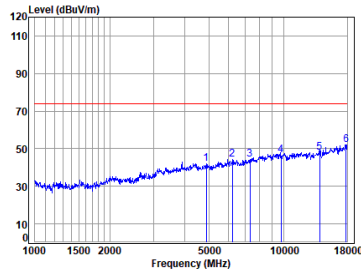
BLE_1M_TX_CH_19_Horizontal-Peak
