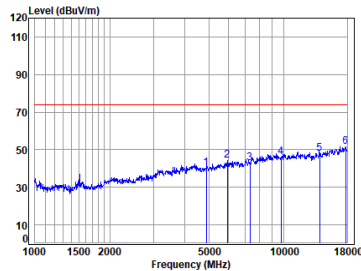
BLE_2M_TX_CH_19_Vertical-Peak
