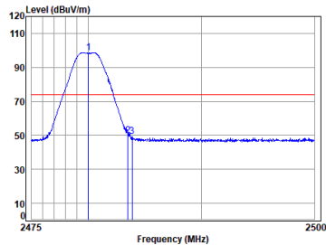
BLE_2M_TX_CH_39_Vertical-Peak
