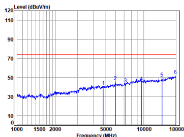
BLE_2M_TX_CH_00_Horizontal-Peak
