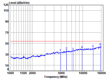
BLE_1M_TX_CH_19_Horizontal-Avg
