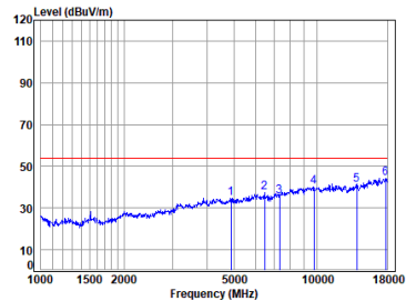
BLE_1M_TX_CH_19_Vertical-Avg
