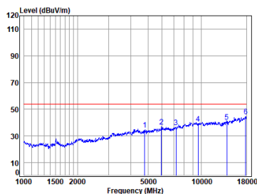
BLE_1M_TX_CH_00_Horizontal-Avg
