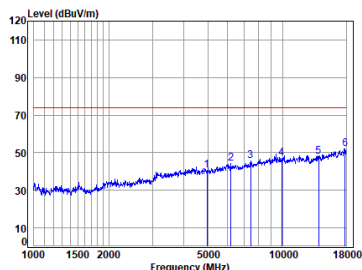
BLE_2M_TX_CH_39_Horizontal-Peak
