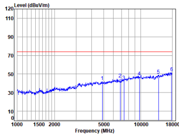
BLE_1M_TX_CH_19_Vertical-Peak
