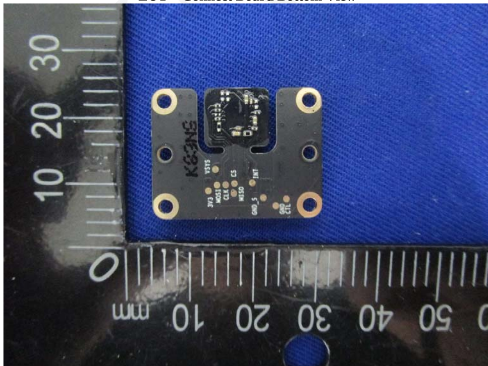
EUT – Connect Board Bottom View
