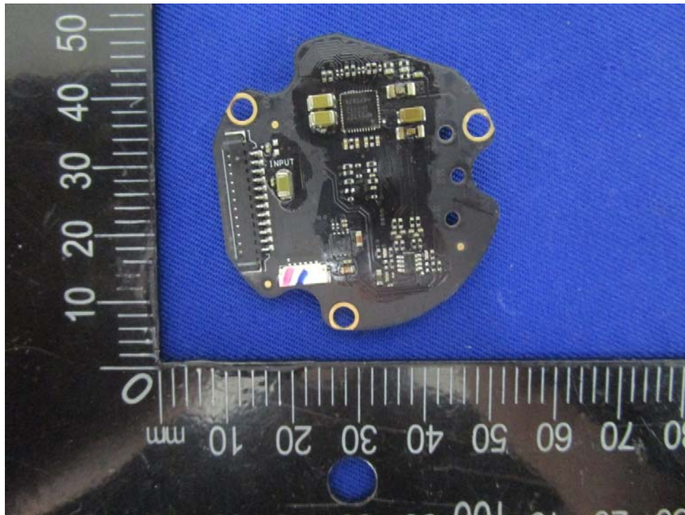
EUT – Motor Control Board Bottom View
