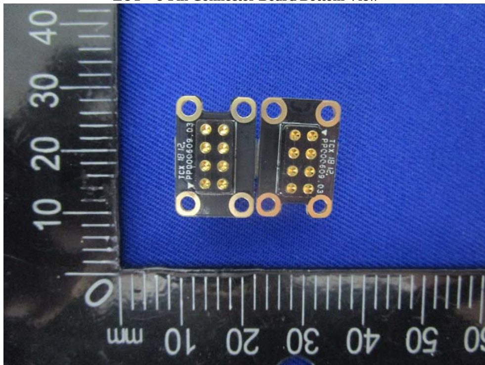
EUT – 8-Pin Connector Board Bottom View
