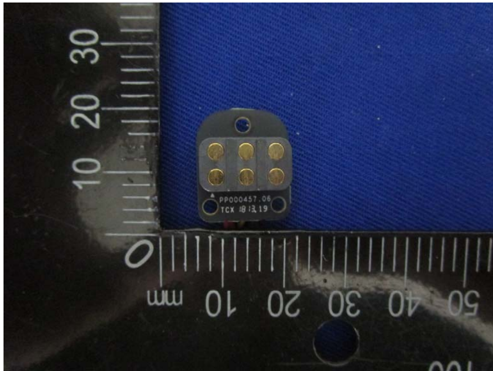
EUT – Contact Board View
