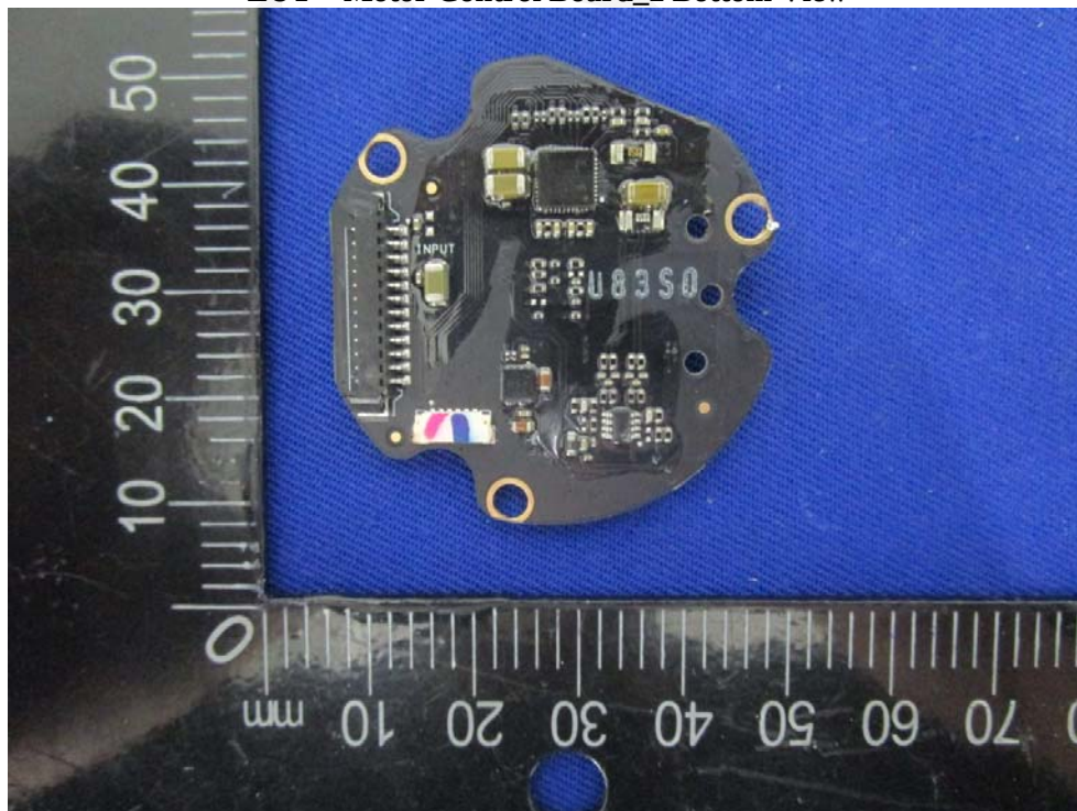
EUT – Motor Control Board_2 Bottom View
