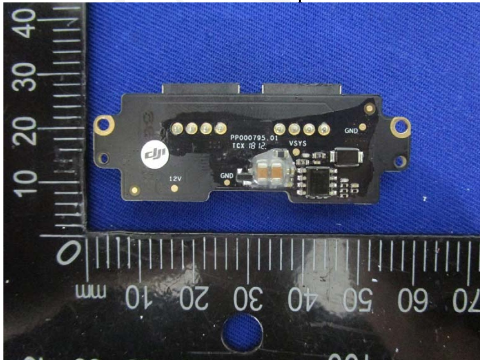
EUT – Connect Board Top View
