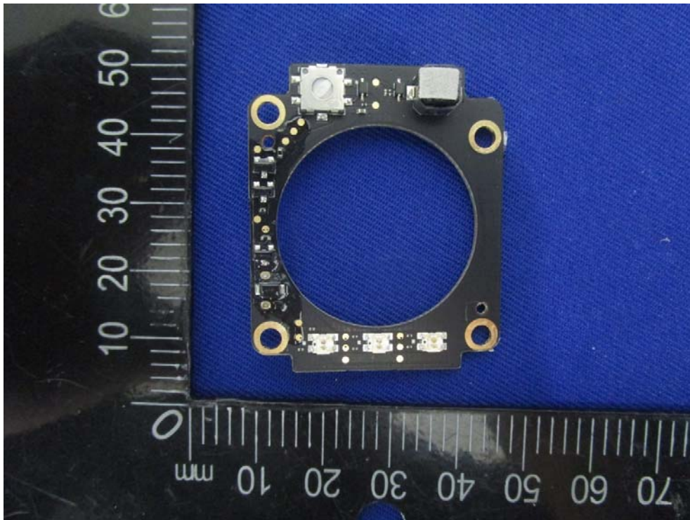
EUT – Button Control Board Bottom View
