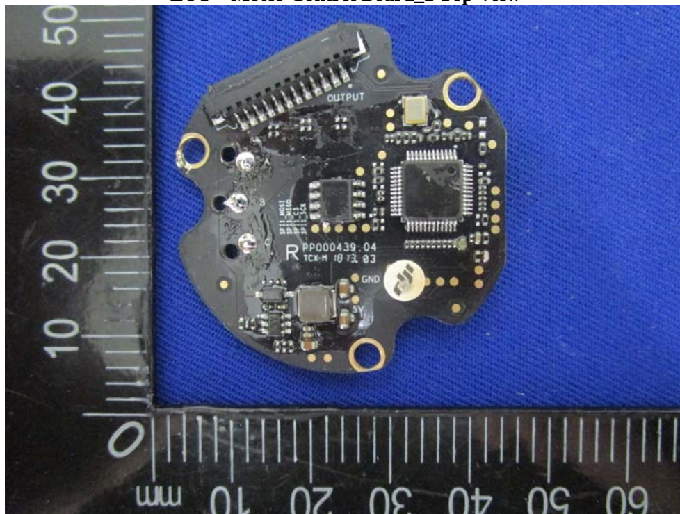
EUT – Motor Control Board_2 Top View
