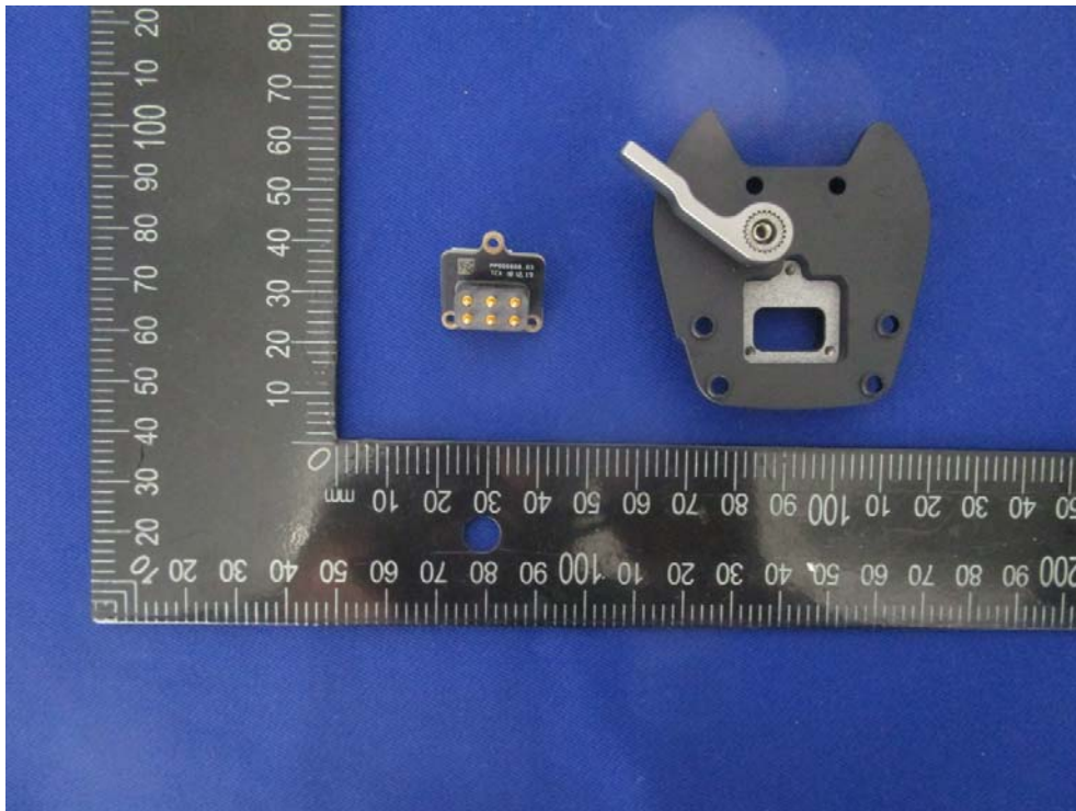
EUT – Uncover3 View
