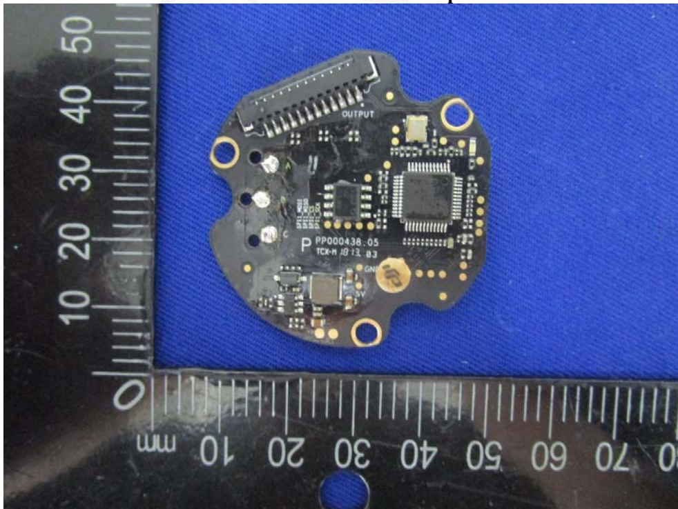
EUT – Motor Control Board Top View
