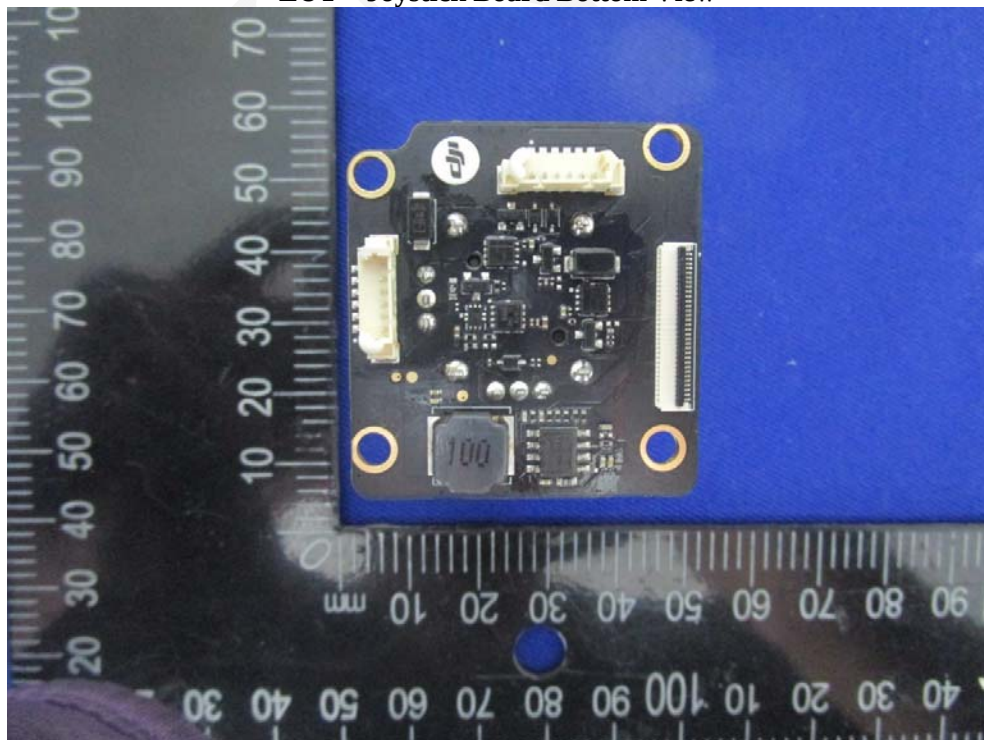
EUT – Joystick Board Bottom View
