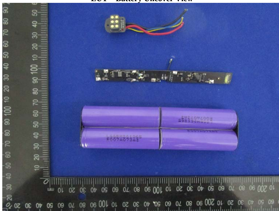
EUT – Battery Uncover View
