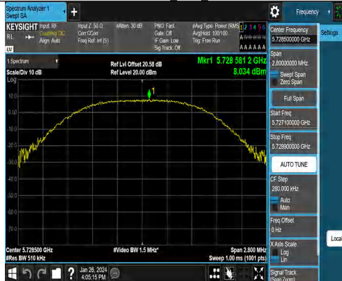
1.4M MIMO Ant3 5728.5
