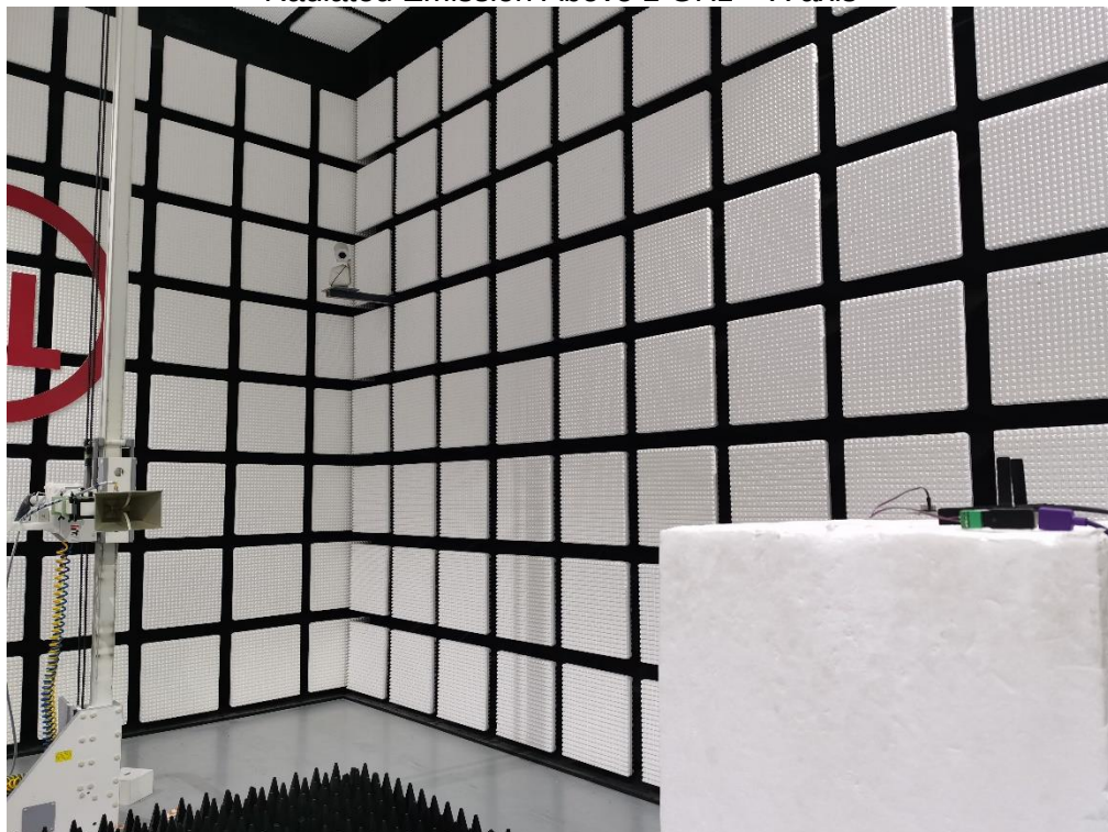
Radiated Emission Above 1 GHz – X axis
