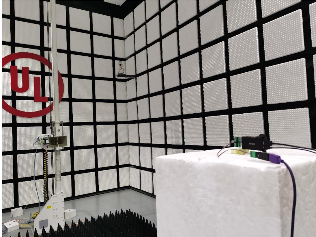
Radiated Emission Above 1 GHz – Y axis
