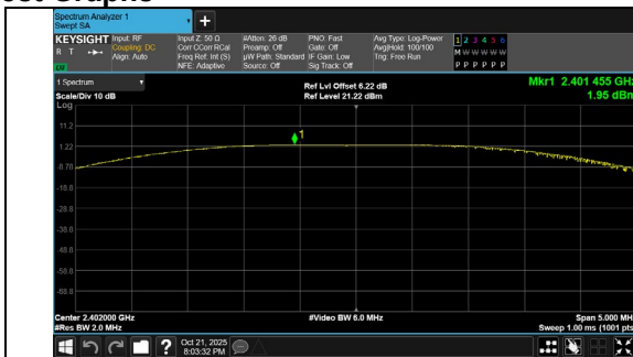
Peak Output Power BLE 2M_Channel 0
