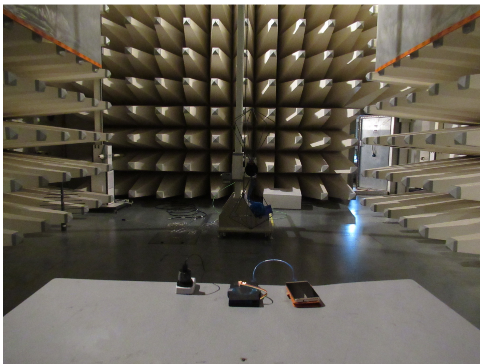
Set-up for Radiated Emission (Charging + Discharging mode)
