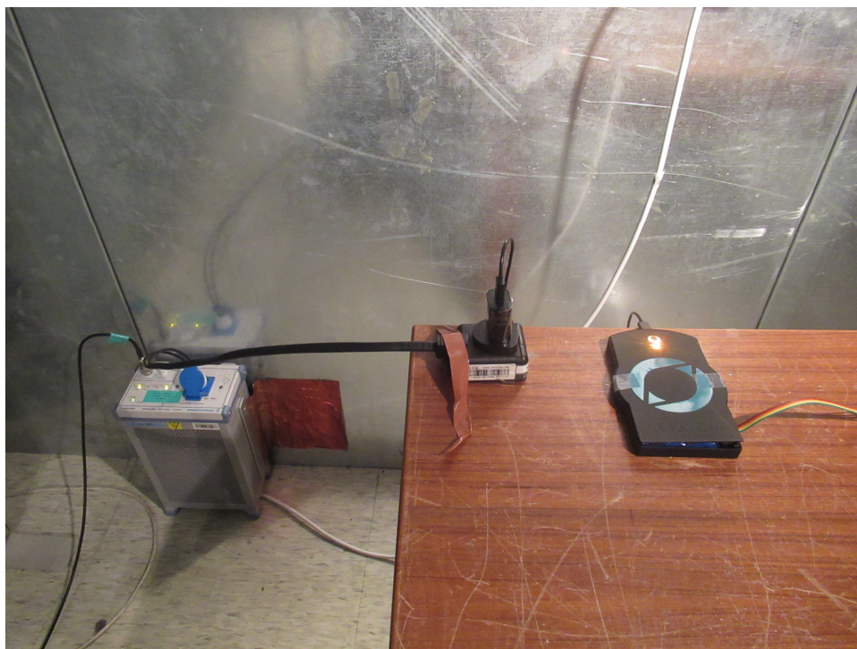
Set-up for AC Mains Conducted Emission (Charging mode + TX mode)
