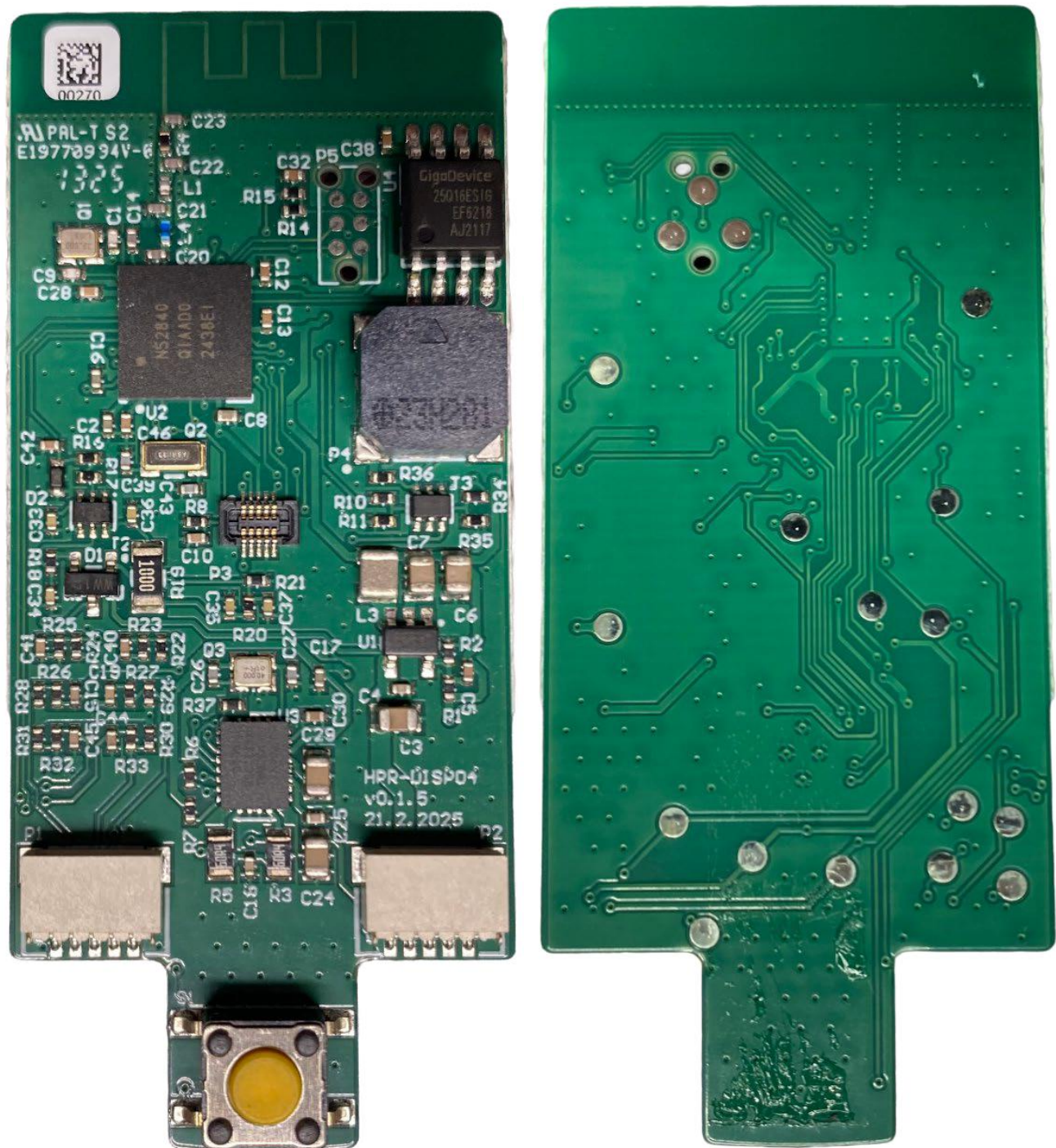
Internal photos - PCB
