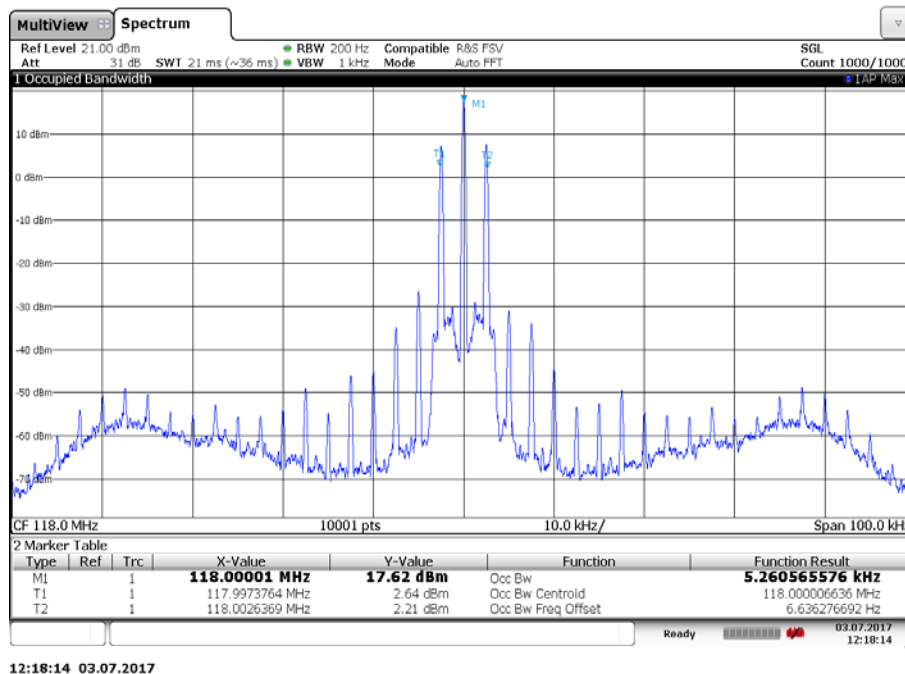
Plot 1: 8.33 kHz channel bandwidth, 118.000 MHz
