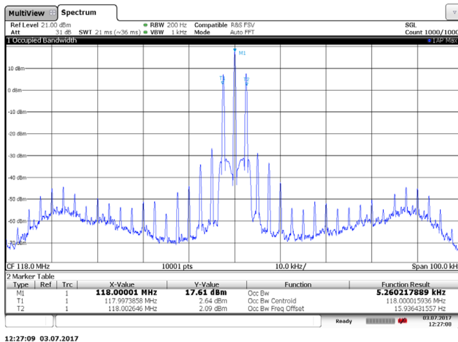
Plot 2: 25 kHz channel bandwidth, 118.000 MHz
