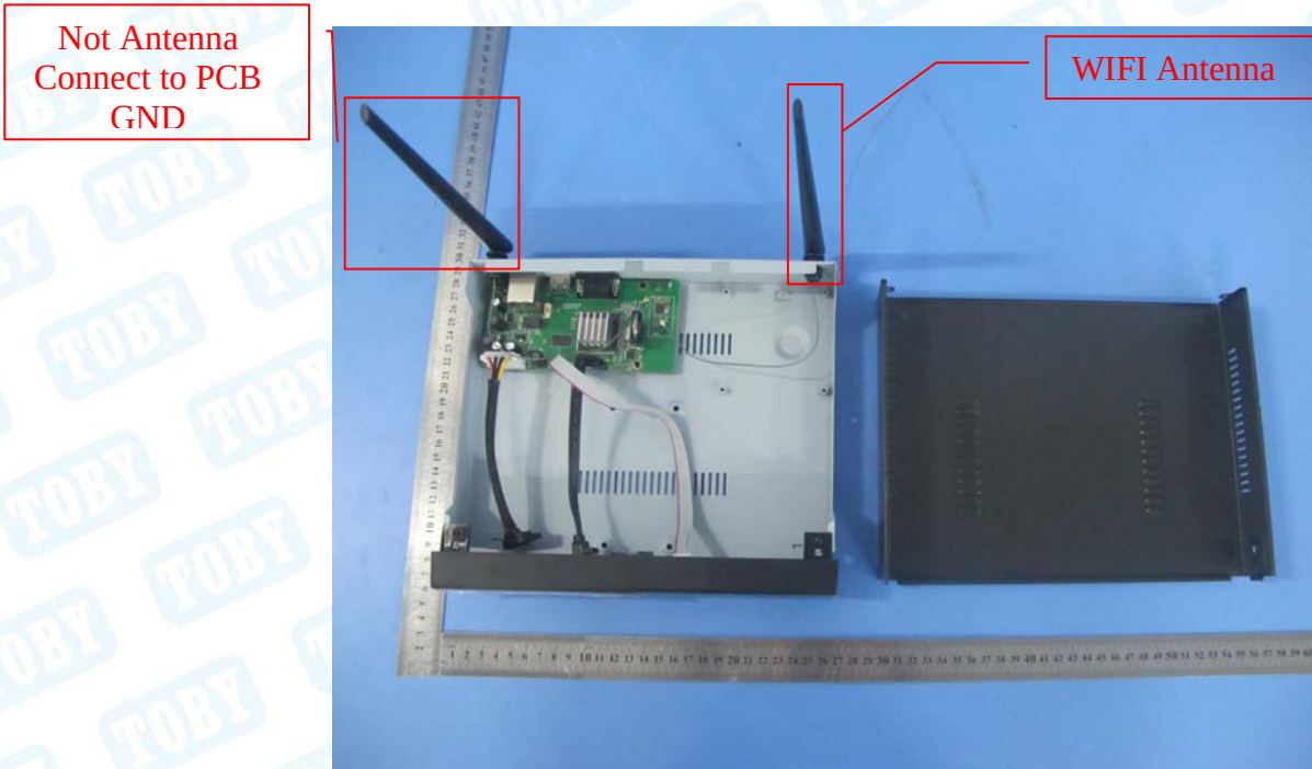
Photo 8 Internal of EUT
