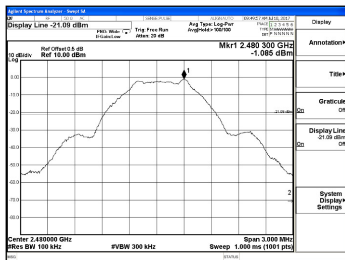
Channel 39 / 2480 MHz
