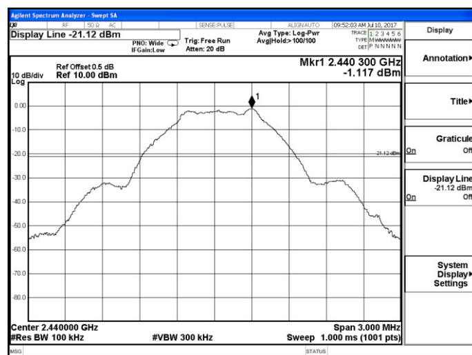
Channel 19 / 2440 MHz
