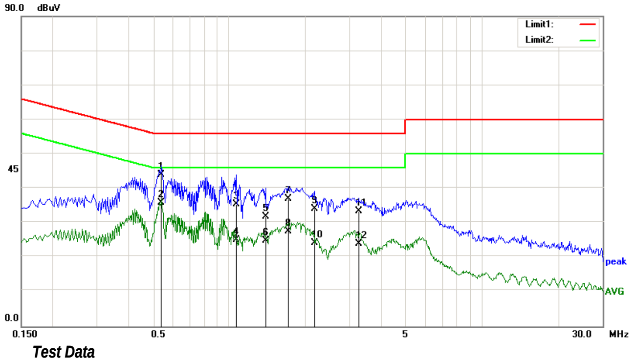
Phase Neutral Plot at 230Vac, 50Hz
