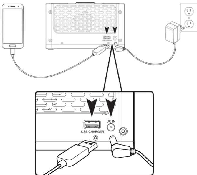
Power ports on the back of the clock
