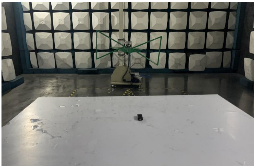
Radiated Emissions below 1GHz
