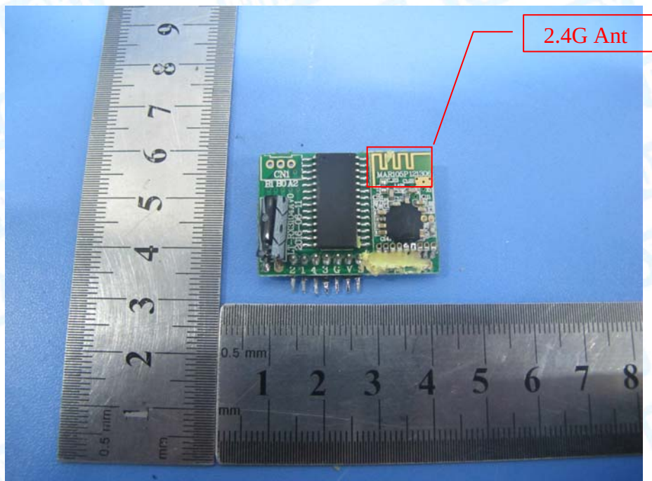
Photo 15 Appearance of PCB
