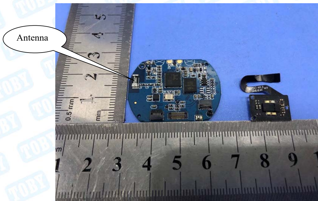
Photo 6 Appearance of PCB
