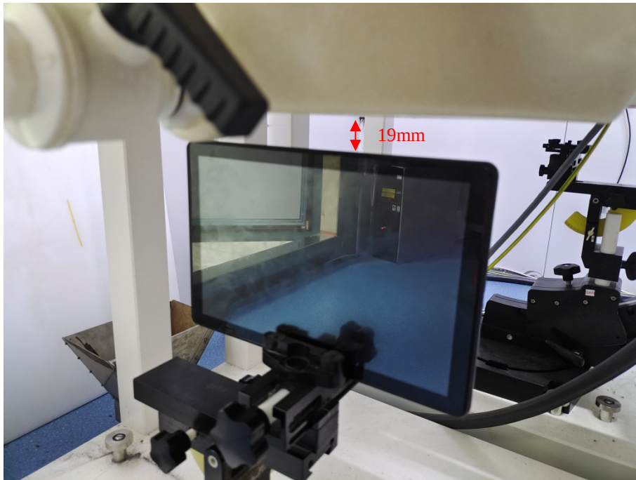
Body Bottom Setup Photo (19mm)
