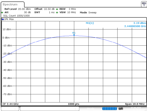
BLE_1M_Middle_Channel
