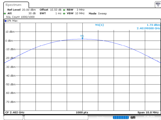
BLE_1M_Low_Channel
