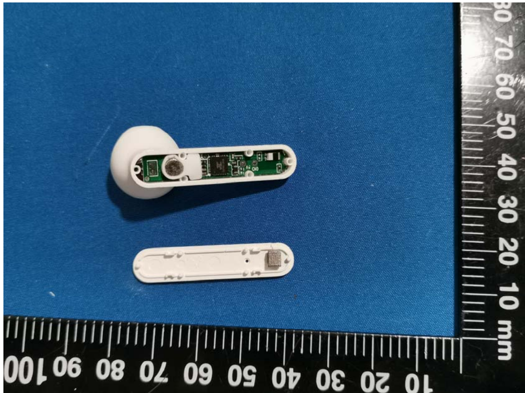
Right Unit
