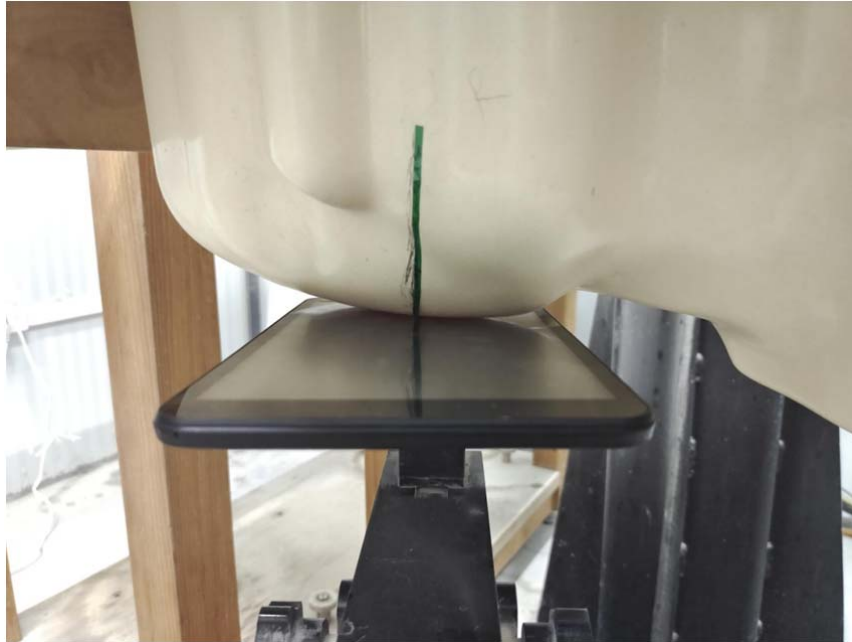
Head Right Cheek Setup Photo
