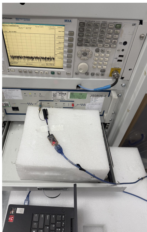
Fig. 3 Conducted Measurement
