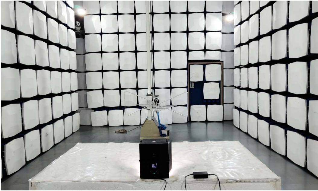
Radiated Emission Test Setup:
