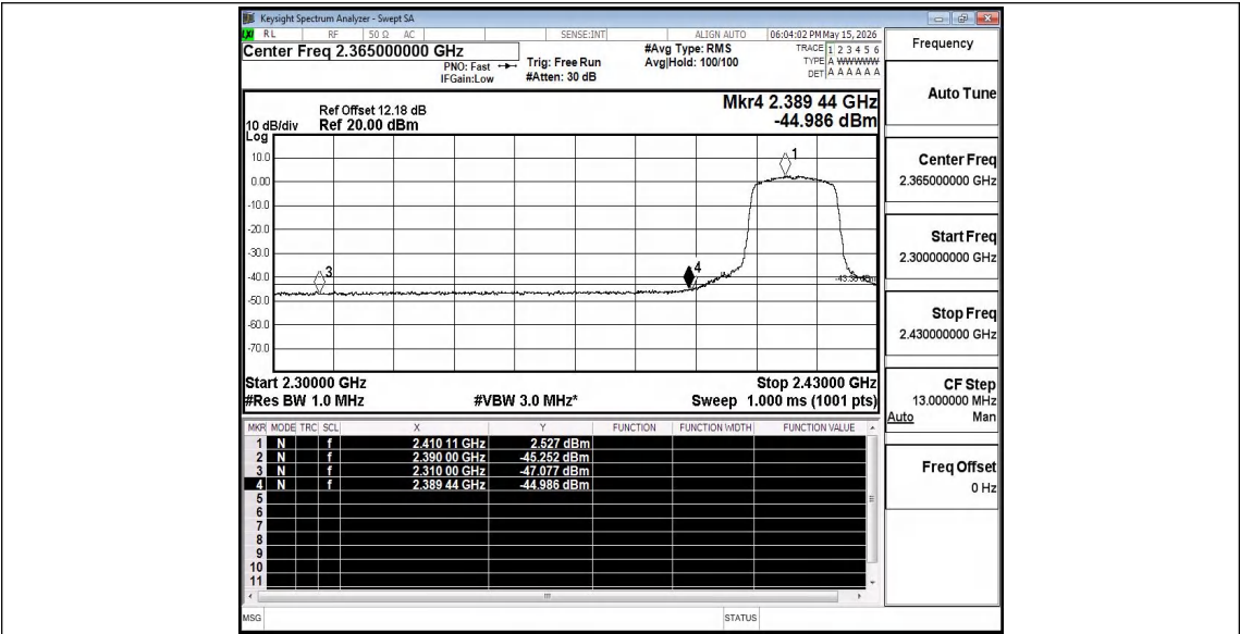
11N20SISO_Ant1_Low_2412_Peak
