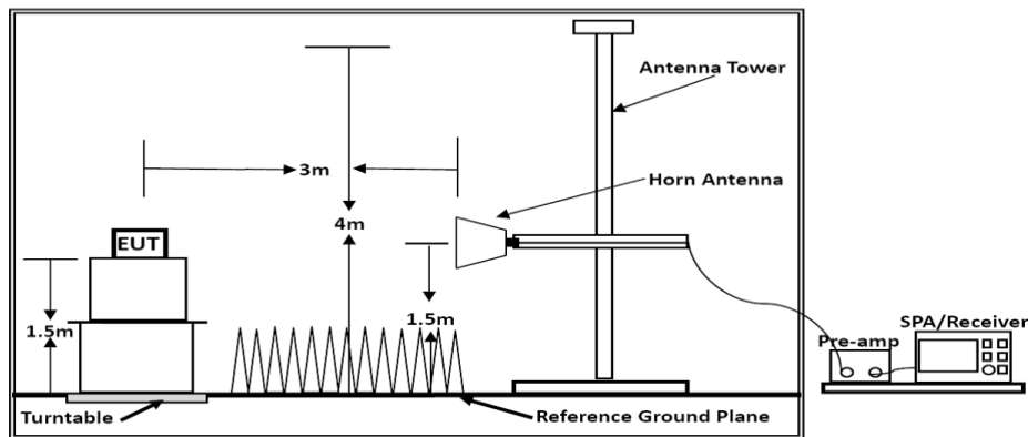
Above 1GHz
