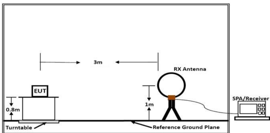
Below 30MHz
