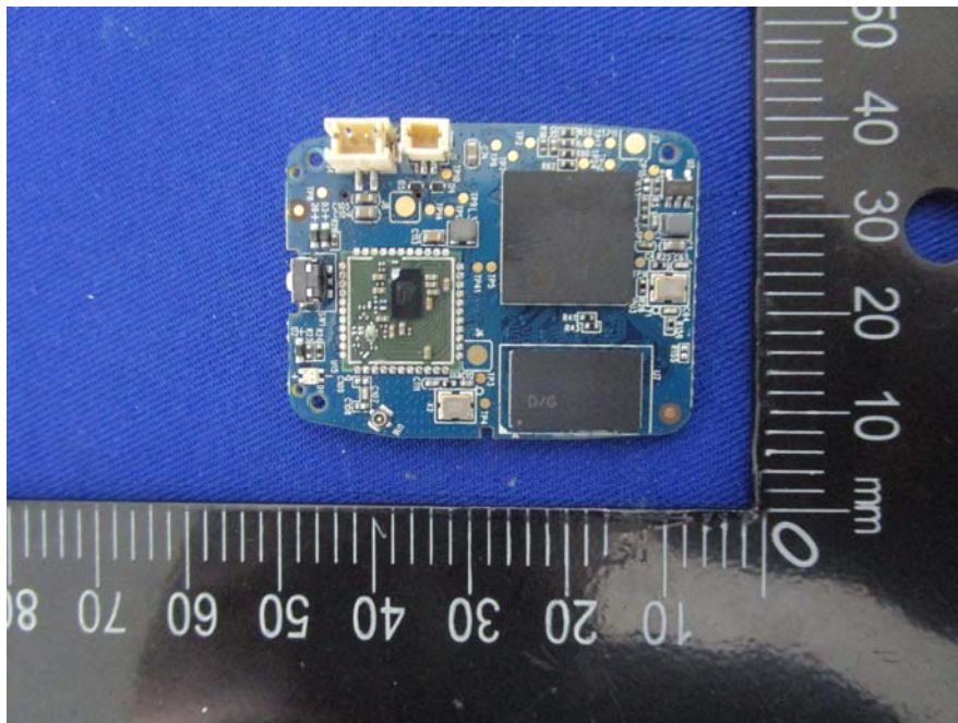
EUT – Board 2 Top Uncover 2 View
