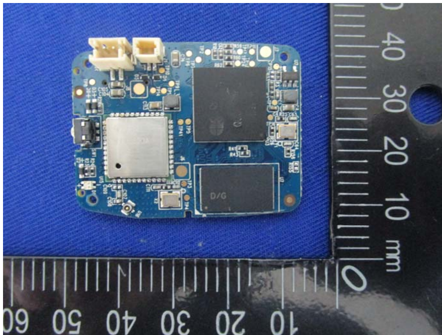
EUT – Board 2 Top Uncover 1 View
