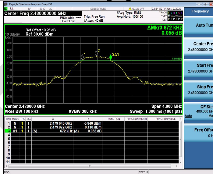
GFSK/1M_Ant1_2480
