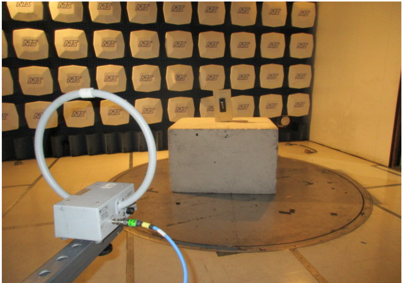
Radiated Measurements Setup 0.009-30MHz
