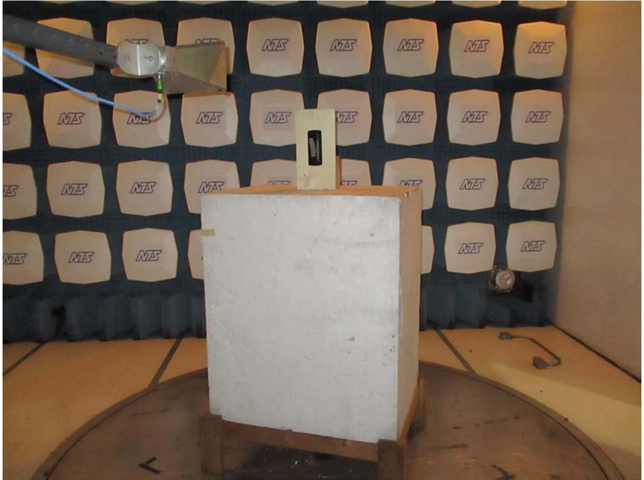
Radiated Measurements Setup 10-18GHz
