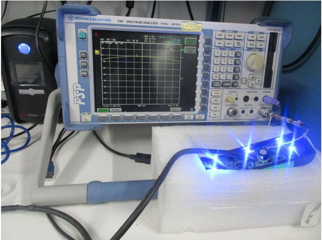
Figure 6: RF Conducted Emissions (BLE only)
