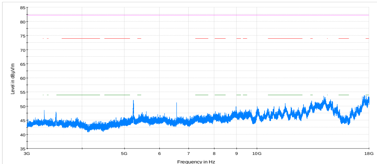
Figure 8.1-33: Radiated emissions within 3–18 GHz, Wi-Fi high channel, LTE B5 high channel, peak measurement
