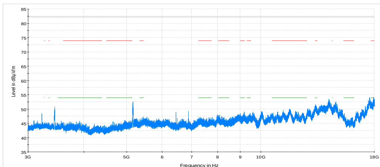
Figure 8.1-19: Radiated emissions within 3–18 GHz, Wi-Fi low channel, LTE B5 low channel, peak measurement
