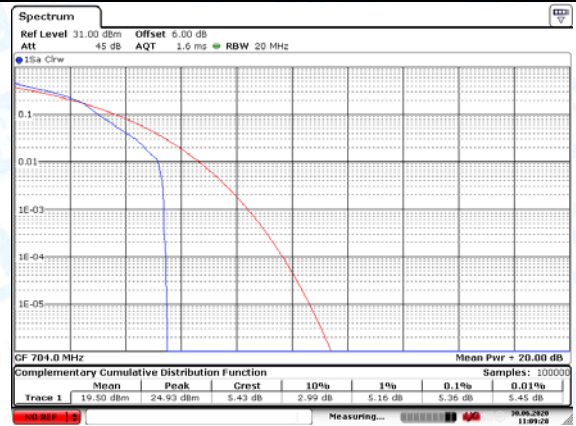
LTE Band 12 10MHz (Low Channel)-16QAM
