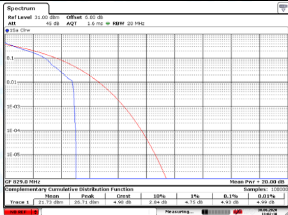
LTE Band 5 10MHz (Low Channel)-QPSK
