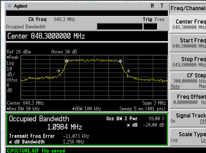
LTE BAND 26 (1.4MHz QPSK-High CH)
