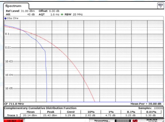
LTE Band 12 10MHz (High Channel)-16QAM
