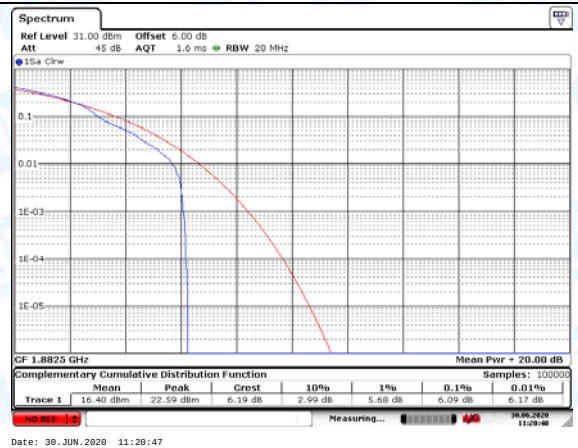
LTE Band 25 20MHz (Middle Channel)-16QAM
