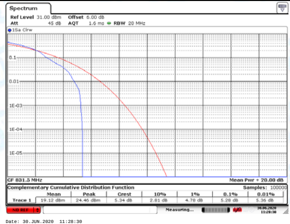
LTE Band 26 15MHz (Middle Channel)-16QAM
