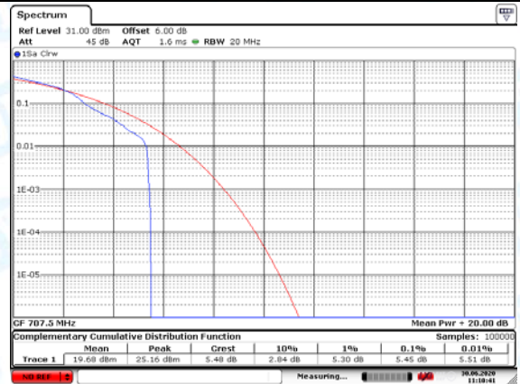
LTE Band 12 10MHz (Middle Channel)-16QAM
