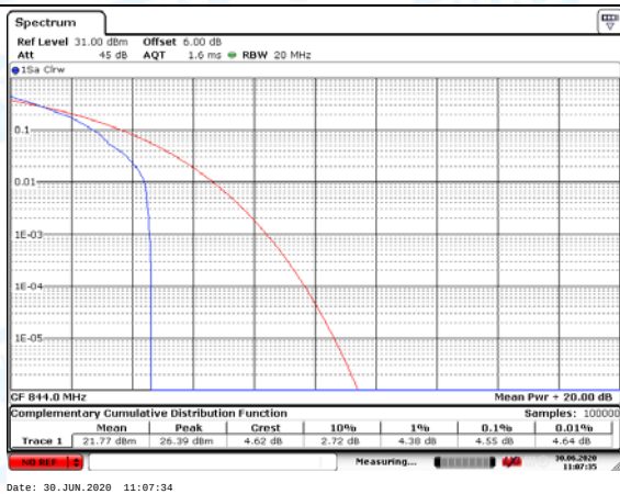
LTE Band 5 10MHz (High Channel)-QPSK
