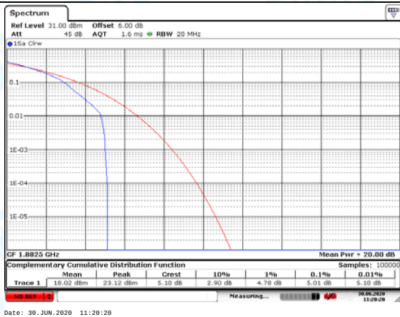
LTE Band 25 20MHz (Middle Channel)-QPSK
