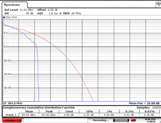
LTE Band 12 10MHz (Low Channel)-QPSK
