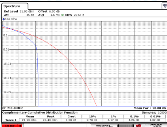
LTE Band 12 10MHz (High Channel)-QPSK
