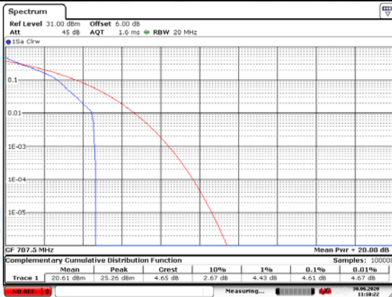
LTE Band 12 10MHz (Middle Channel)-QPSK
