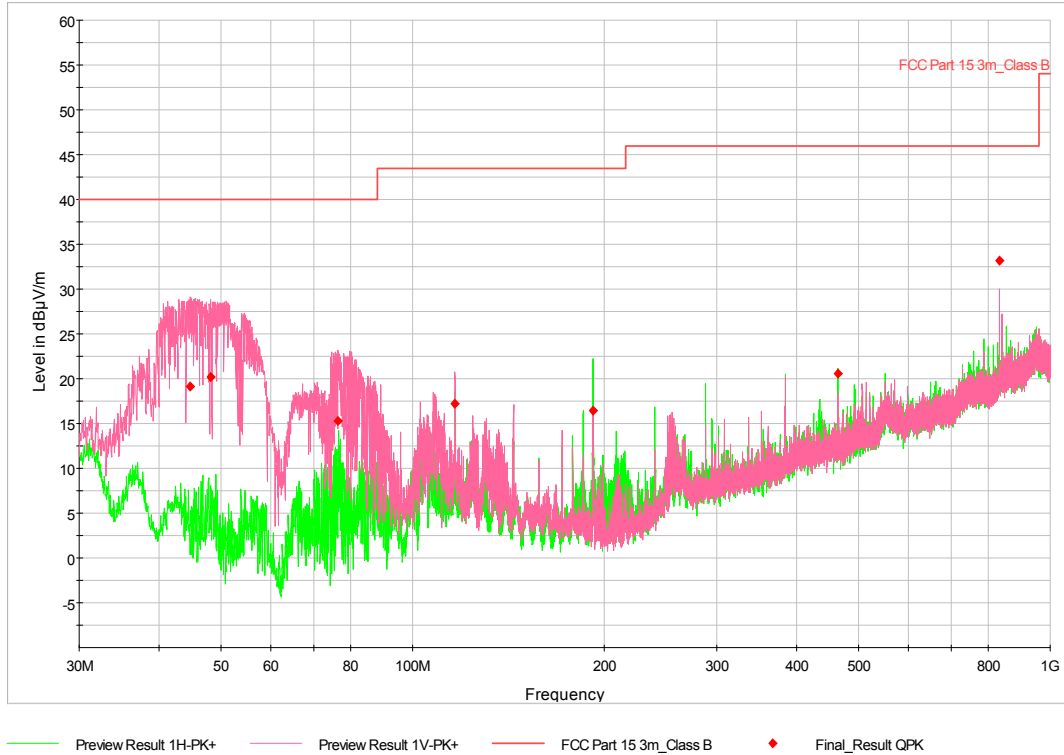
Figure 7-32: Radiated Emissions - 30 MHz to 1 GHz (§ 15.205, 15.209) – Configuration 5
