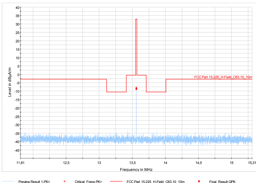
Figure 7-27: Radiated Emissions – 11.810 MHz to 15.310 MHz (§ 15.225a-c) – Configuration 3; Horizontal Polarization
