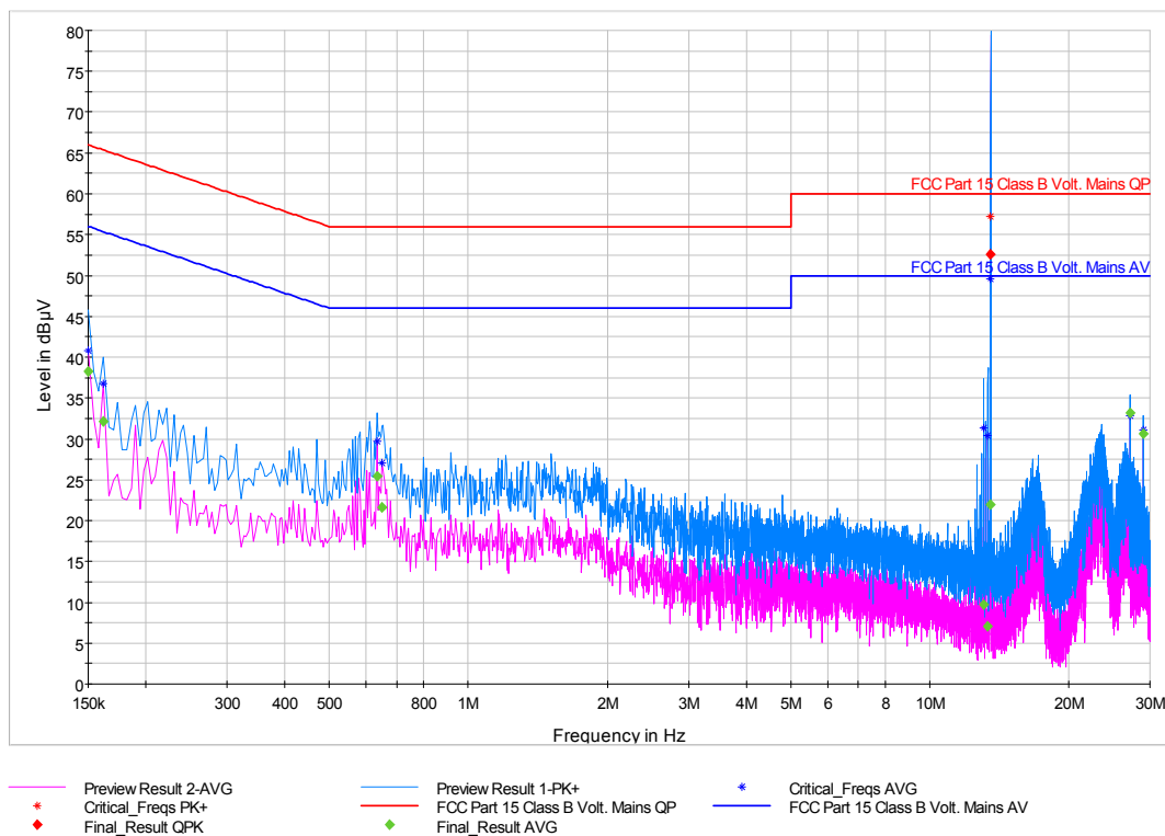
Figure 7-8: Conducted Emissions (150 kHz – 30 MHz), Phase Line – Configuration 12, Top antenna (120 V / 60 Hz)
