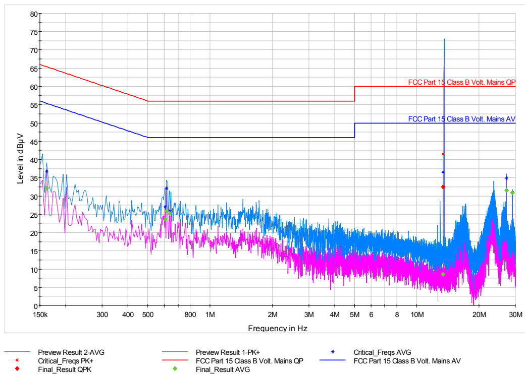
Figure 7-2: Conducted Emissions (150 kHz – 30 MHz), Phase Line – Configuration 11 (120 V / 60 Hz)
