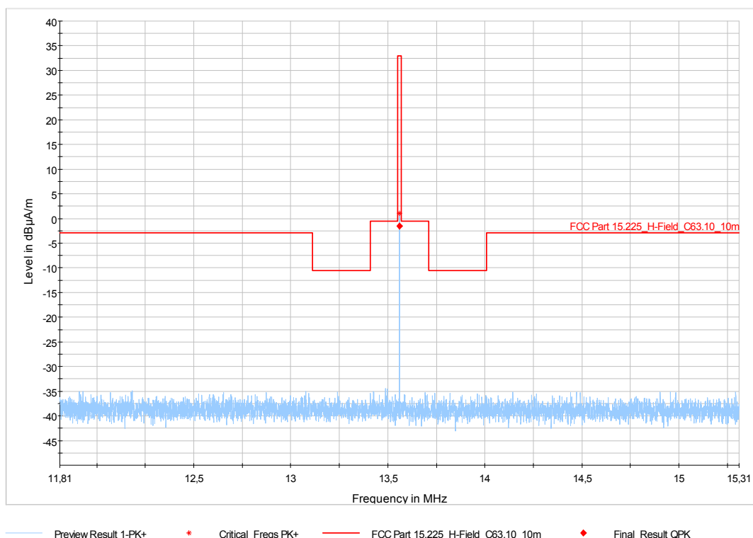
Figure 7-28: Radiated Emissions – 11.810 MHz to 15.310 MHz (§ 15.225a-c) – Configuration 4; Vertical Polarization
