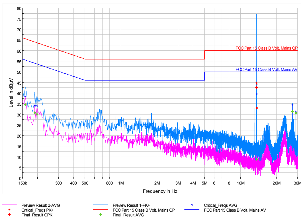
Figure 7-10: Conducted Emissions (150 kHz – 30 MHz), Phase Line – Configuration 11 (240 V / 60 Hz)
