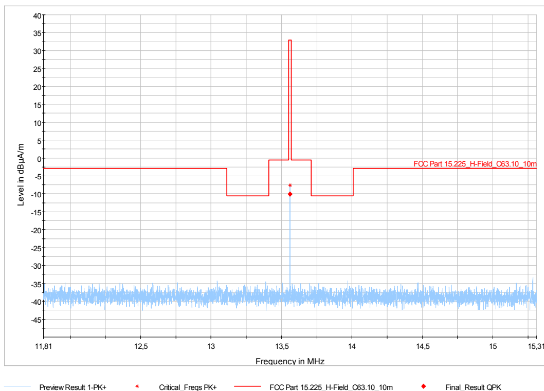
Figure 7-25: Radiated Emissions – 11.810 MHz to 15.310 MHz (§ 15.225a-c) – Configuration 2; Horizontal Polarization
