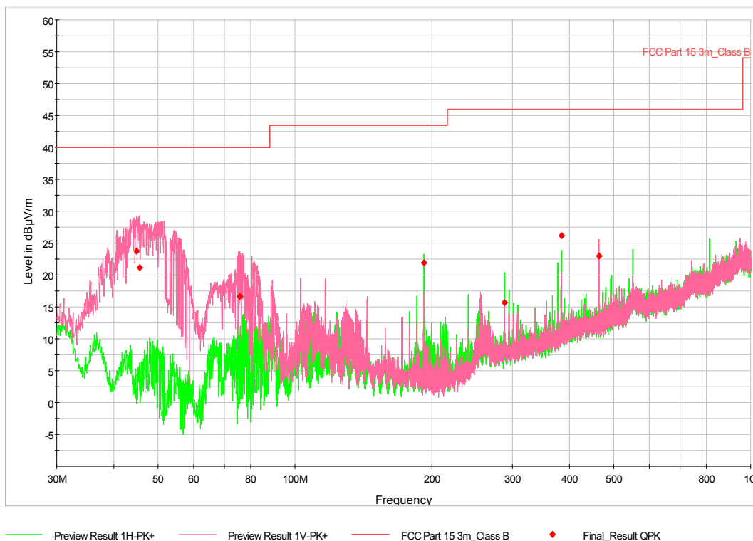
Figure 7-36: Radiated Emissions - 30 MHz to 1 GHz (§ 15.205, 15.209) – Configuration 8
