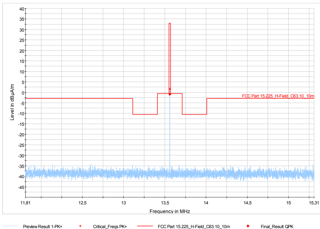
Figure 7-24: Radiated Emissions – 11.810 MHz to 15.310 MHz (§ 15.225a-c) – Configuration 2; Vertical Polarization
