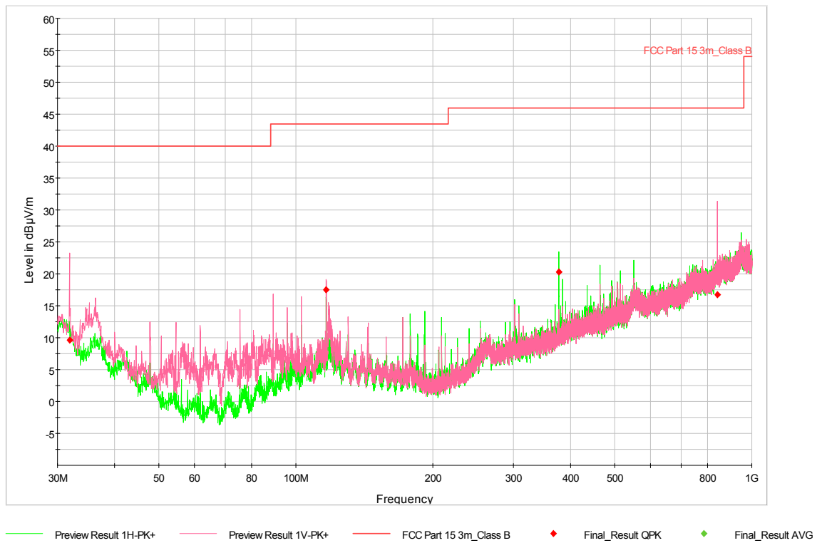
Figure 7-37: Radiated Emissions - 30 MHz to 1 GHz (§ 15.205, 15.209) – Configuration 10
