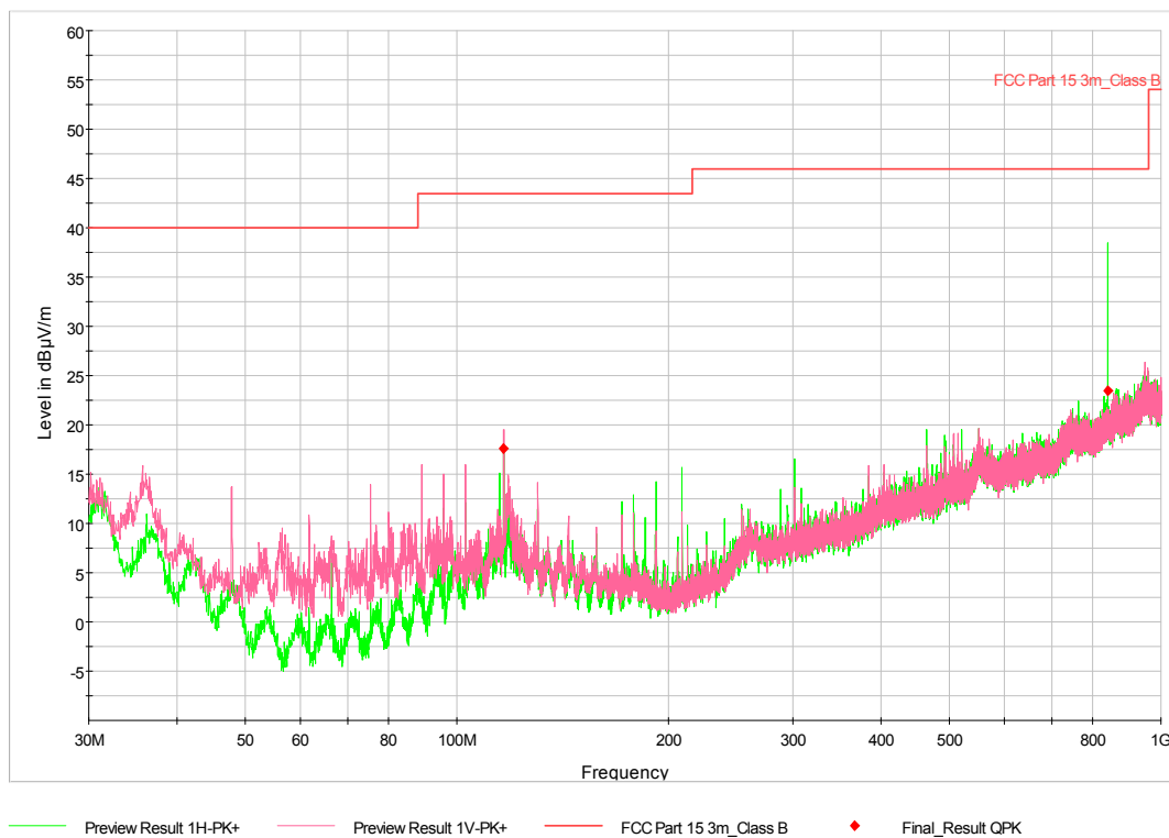
Figure 7-34: Radiated Emissions - 30 MHz to 1 GHz (§ 15.205, 15.209) – Configuration 9
