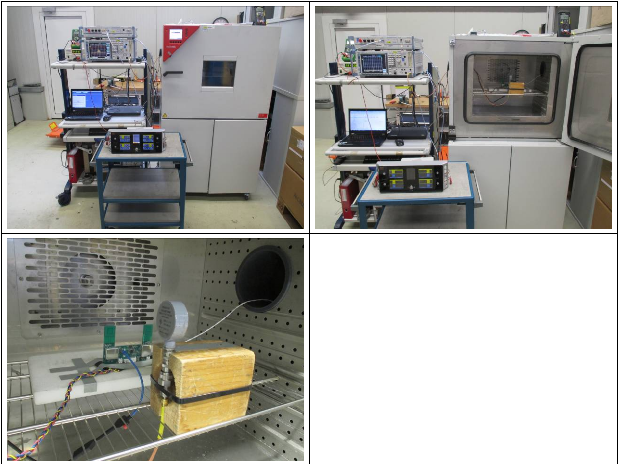
Figure 7-45: Test Setup – Frequency Stability with voltage or Temperature variation – Configurations 1 & 2
