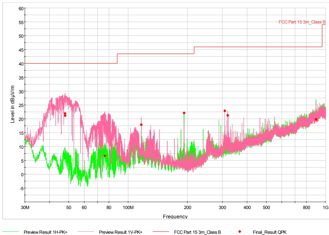
Figure 7-33: Radiated Emissions - 30 MHz to 1 GHz (§ 15.205, 15.209) – Configuration 6
