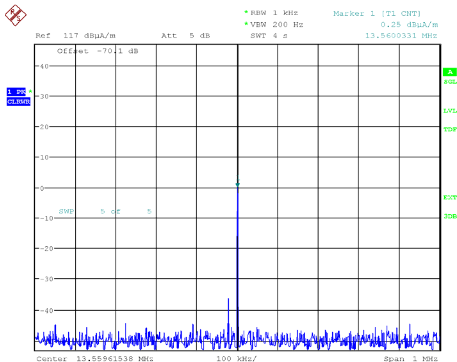
Figure 7-38: Frequency stability – 20 °C / 5 V at startup – Configuration 1
