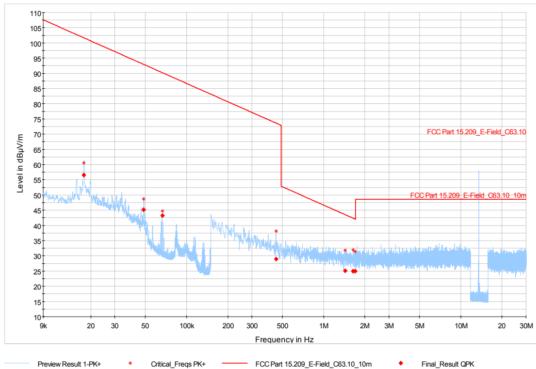
Figure 7-31: Radiated Emissions – 9 kHz to 30 MHz (§ 15.225d) – Configuration 5
