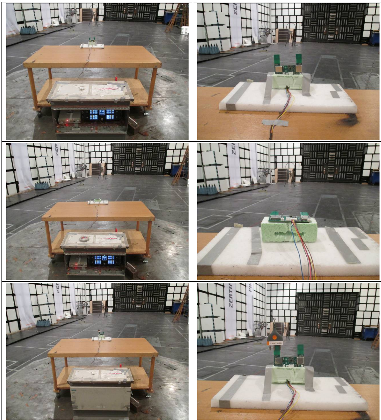
Figure 7-44: Test Setup Radiated Emission 9 kHz – 30 MHz – Configuration 1, 2, 3, 4, 5
