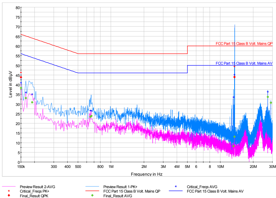
Figure 7-14: Conducted Emissions (150 kHz – 30 MHz), Phase Line – Configuration 12, Bottom antenna (240 V / 60 Hz)
