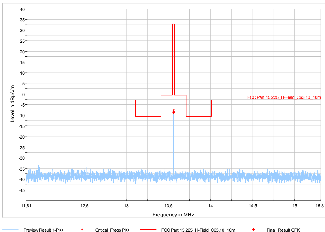
Figure 7-22: Radiated Emissions – 11.810 MHz to 15.310 MHz (§ 15.225a-c) – Configuration 1; Horizontal Polarization
