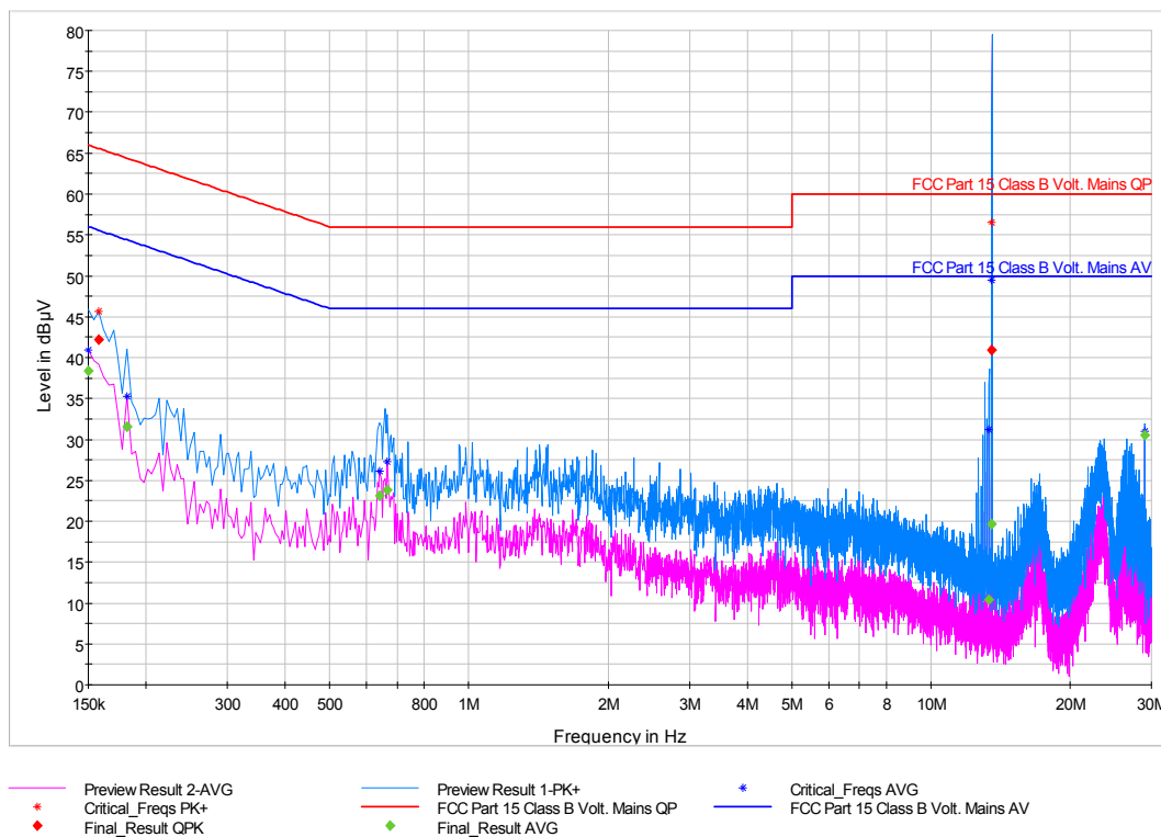
Figure 7-16: Conducted Emissions (150 kHz – 30 MHz), Phase Line – Configuration 12, Top antenna (240 V / 60 Hz)
