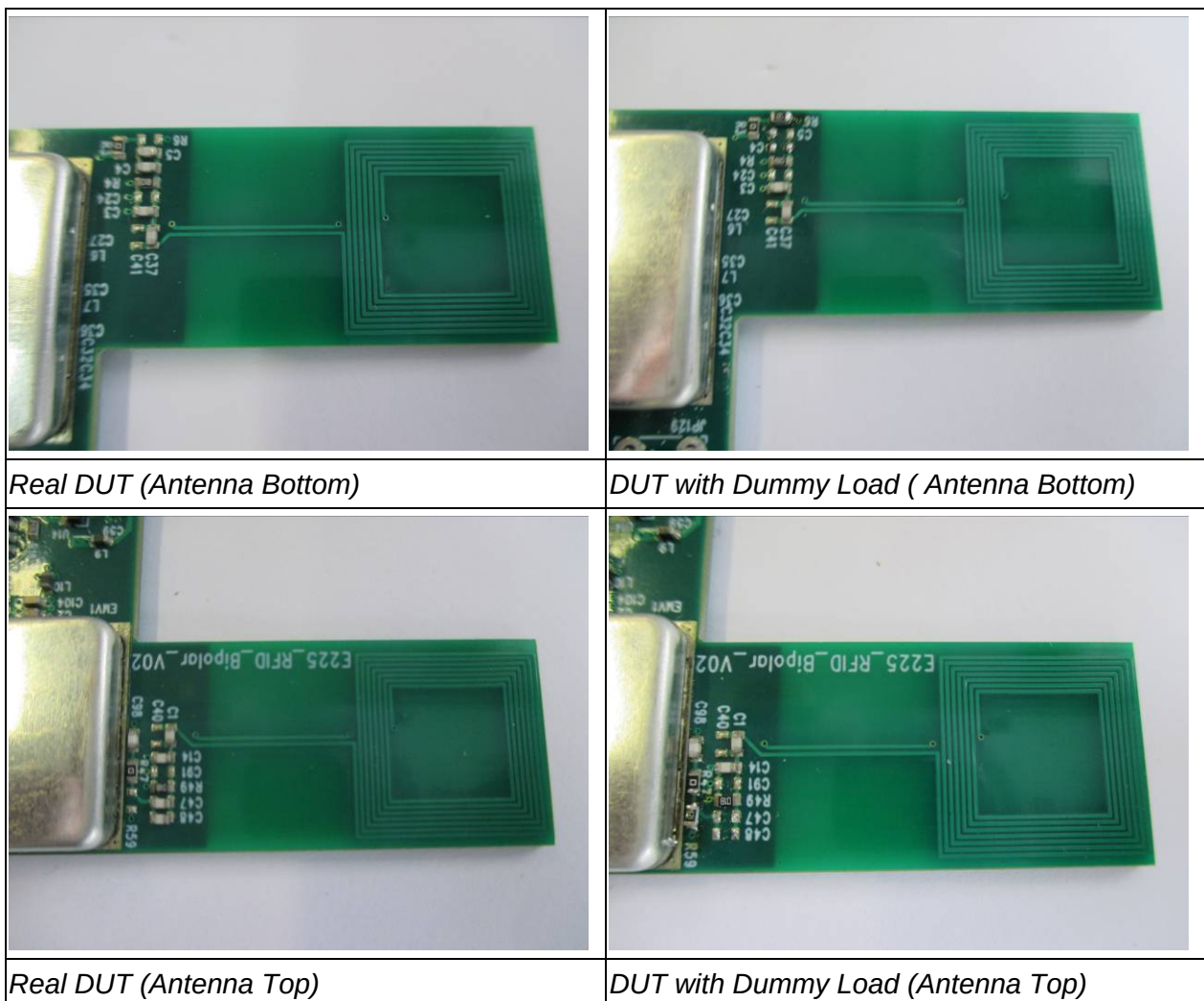
Figure 7-47: RFID Reader Bipolar - Differences between real Module and Dummy Load
