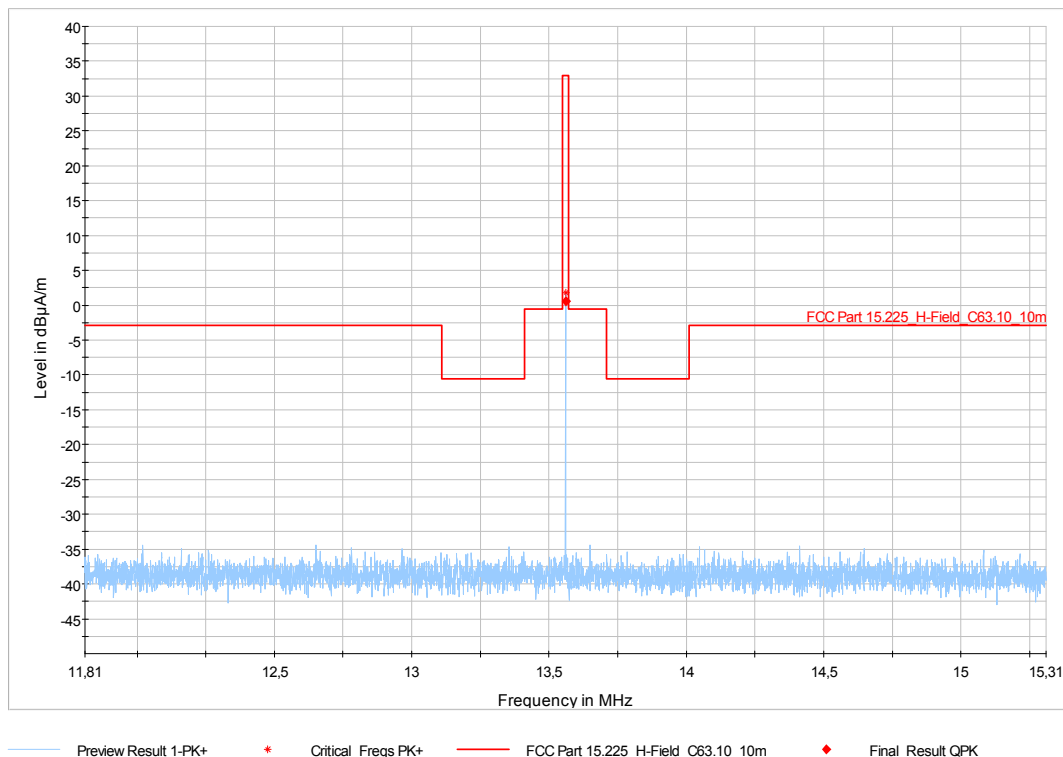
Figure 7-21: Radiated Emissions – 11.810 MHz to 15.310 MHz (§ 15.225a-c) – Configuration 1; Vertical Polarization
