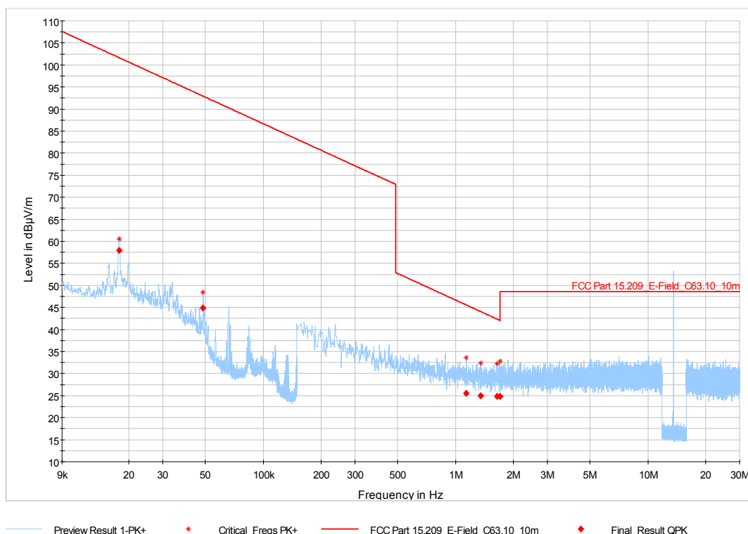
Figure 7-23: Radiated Emissions – 9 kHz to 30 MHz (§ 15.225d) – Configuration 1
