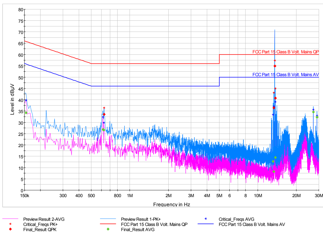
Figure 7-7: Conducted Emissions (150 kHz – 30 MHz), Neutral line – Configuration 12, Top antenna (120 V / 60 Hz))
