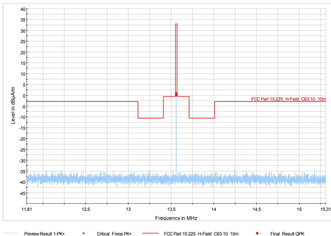
Figure 7-26: Radiated Emissions – 11.810 MHz to 15.310 MHz (§ 15.225a-c) – Configuration 3; Vertical Polarization
