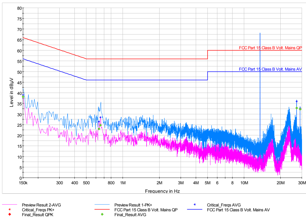
Figure 7-9: Conducted Emissions (150 kHz – 30 MHz), Neutral line – Configuration 11 (240 V / 60 Hz)
