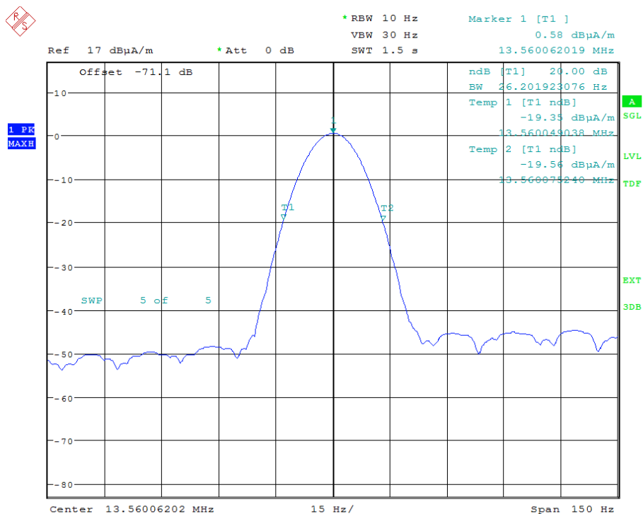
Figure 7-19: Occupied Bandwidth -20 dB (Carrier Frequency 13.56 MHz) – configuration 6
