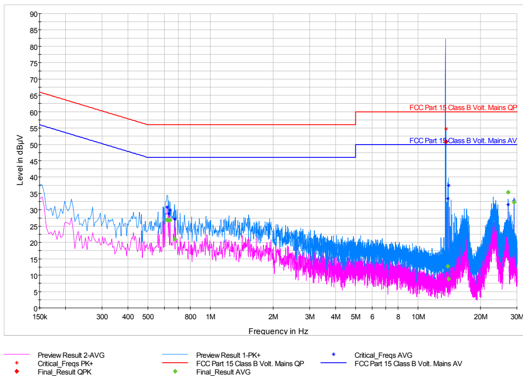
Figure 7-5: Conducted Emissions (150 kHz – 30 MHz), Neutral line – Configuration. 12, Bottom antenna (120 V / 60 Hz)
