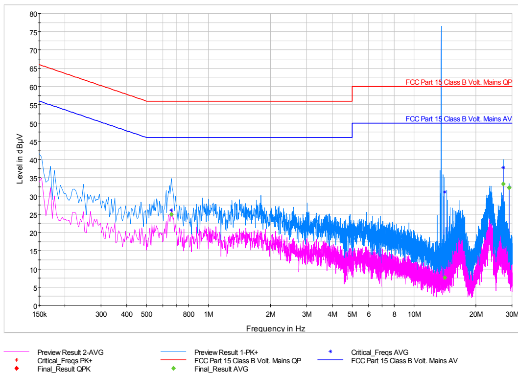
Figure 7-15: Conducted Emissions (150 kHz – 30 MHz), Neutral line – Configuration 12, Top antenna (240 V / 60 Hz)
