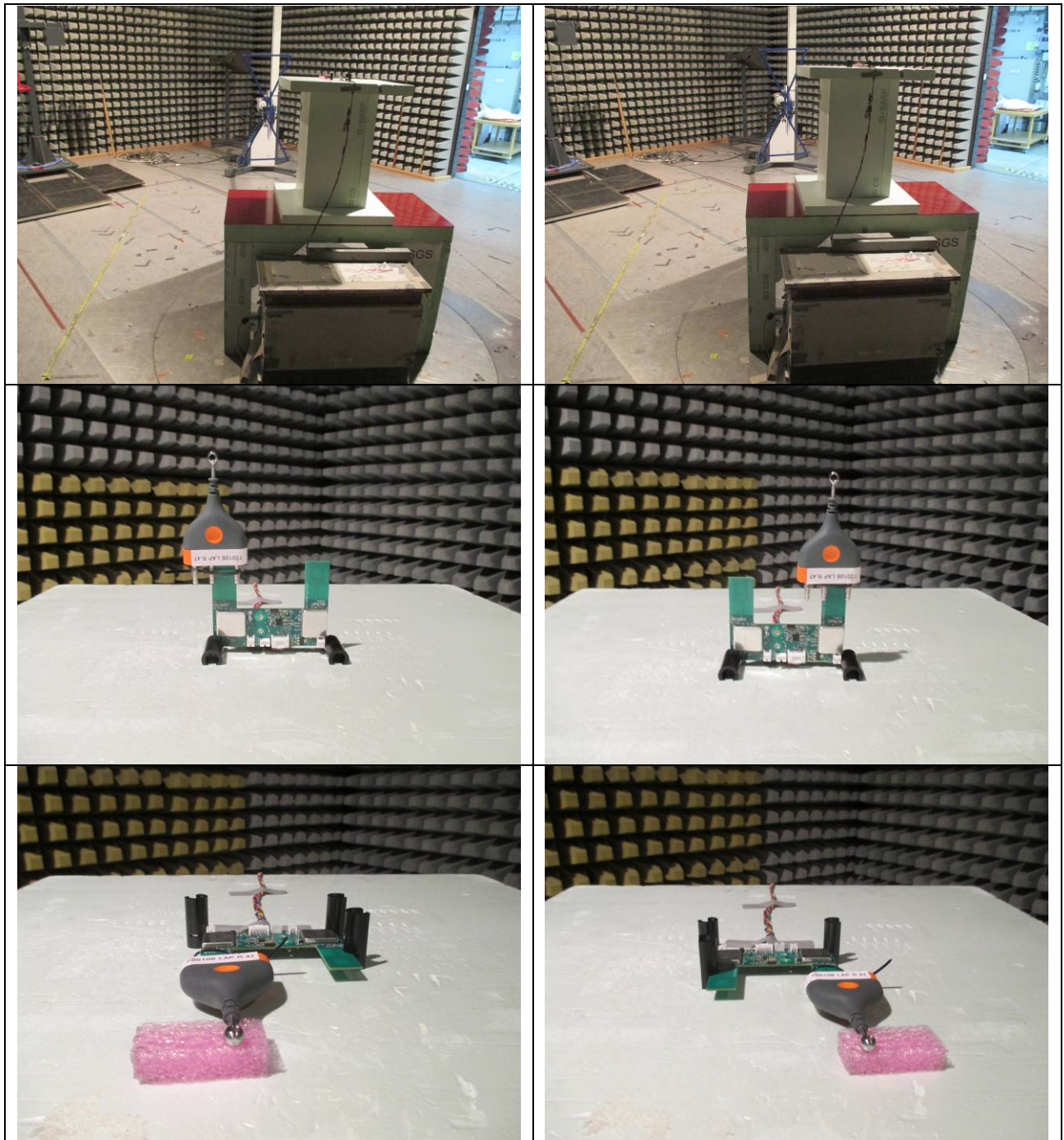
Figure 7-43: Test Setup Radiated Emission 30 MHz – 1 GHz – Configurations 5, 6, 7, 8
