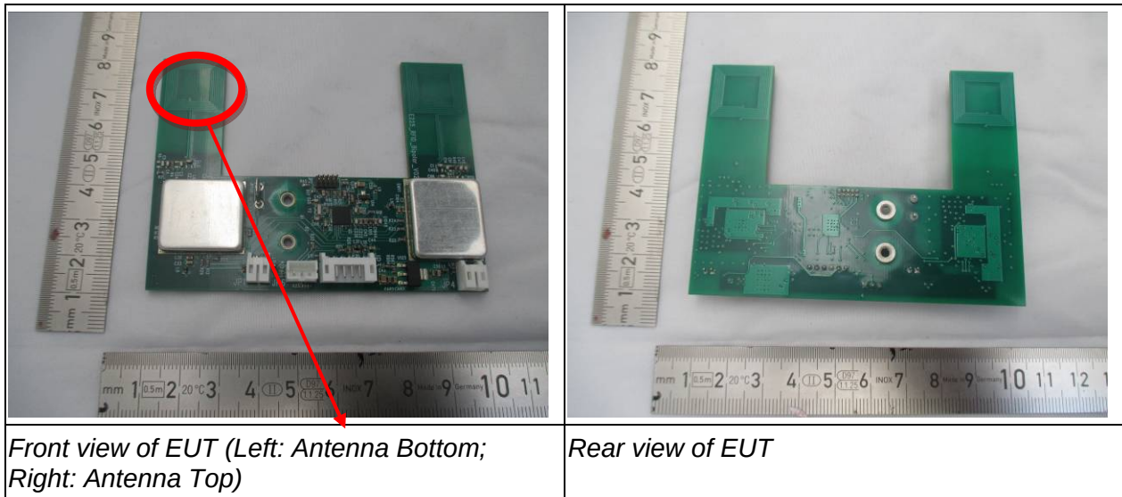
Figure 7-46: RFID Reader Bipolar
