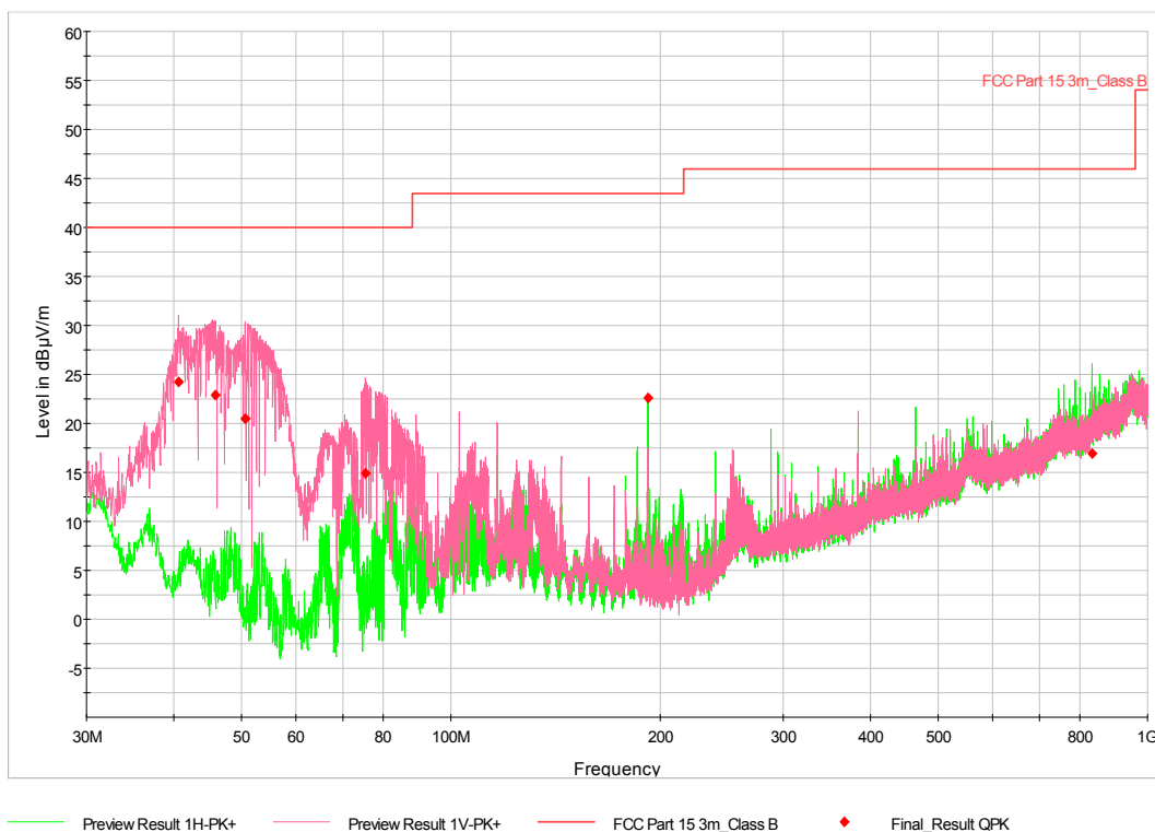
Figure 7-35: Radiated Emissions - 30 MHz to 1 GHz (§ 15.205, 15.209) – Configuration 7
