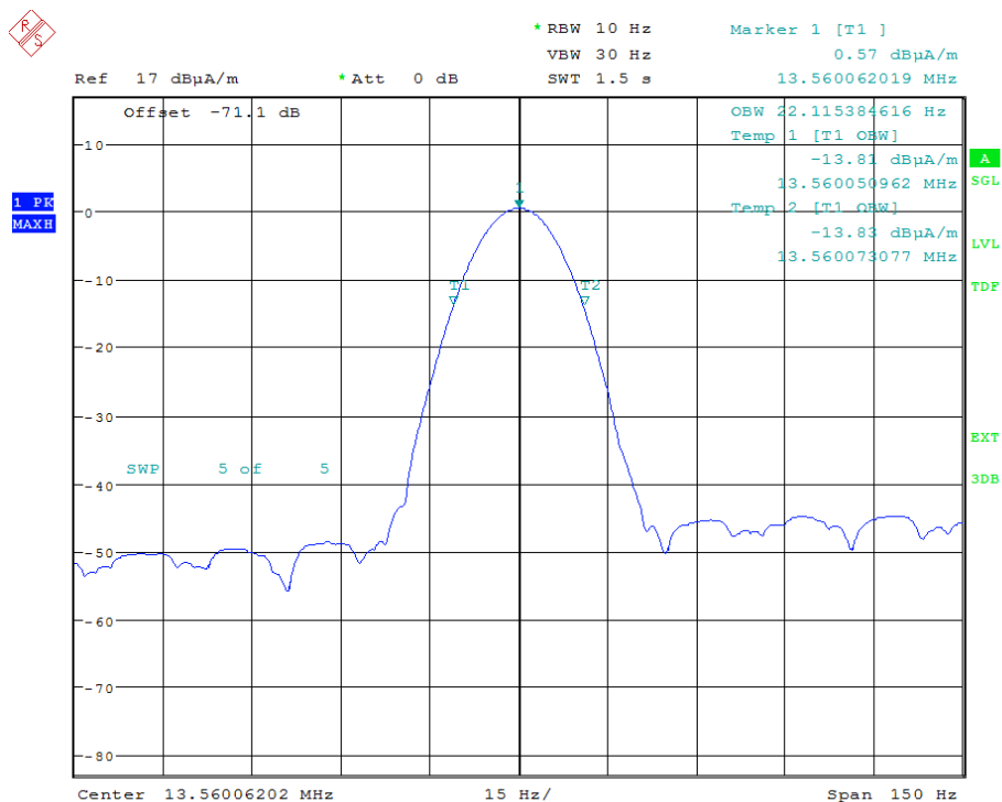
Figure 7-20: Occupied Bandwidth 99% (Carrier Frequency 13.56 MHz) – configuration 6
