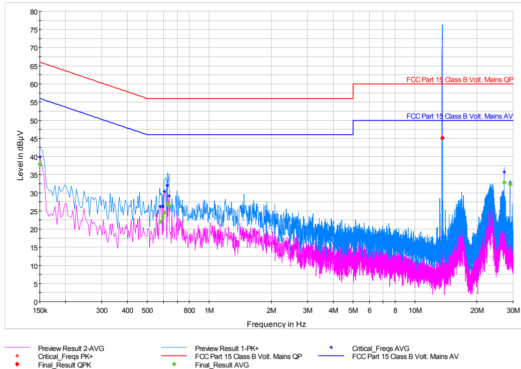
Figure 7-1: Conducted Emissions (150 kHz – 30 MHz), Neutral line – Configuration 11 (120 V / 60 Hz)
