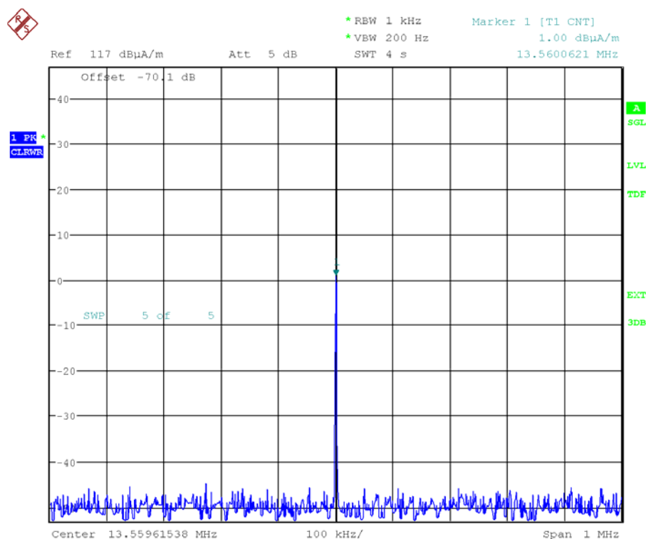
Figure 7-39: Frequency stability – 20 °C / 5 V at startup – Configuration 2
