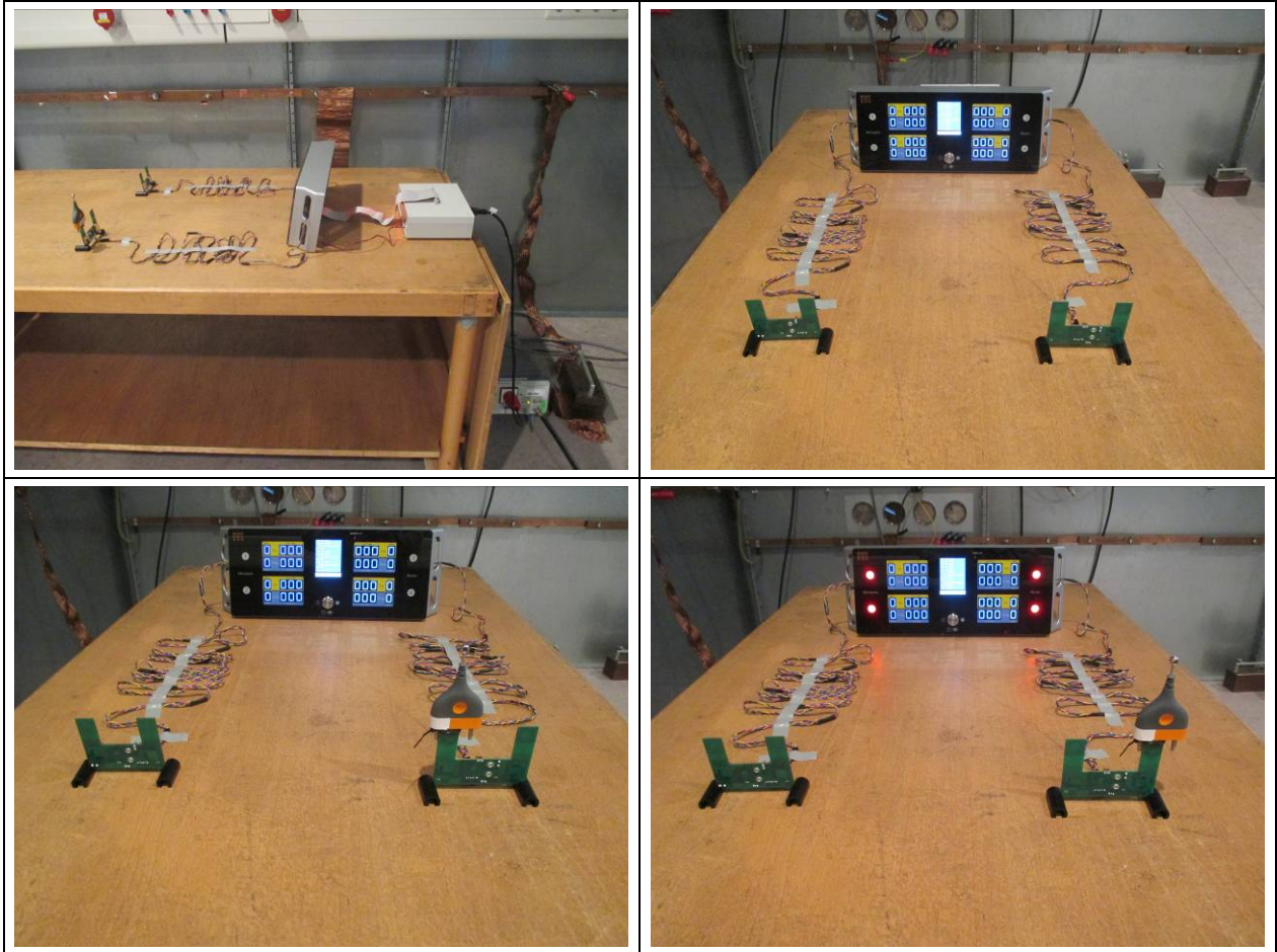
Figure 7-40: Test Setup Conducted Emissions (150 kHz – 30 MHz) – Configurations 11
