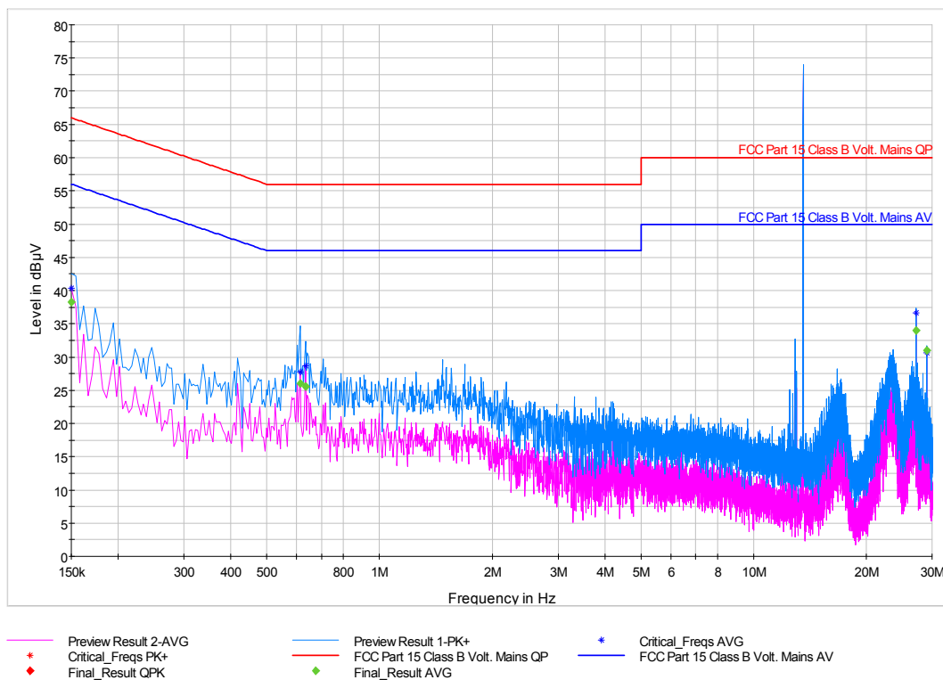
Figure 7-6: Conducted Emissions (150 kHz – 30 MHz), Phase Line – Configuration 12, Bottom antenna (120 V / 60 Hz)
