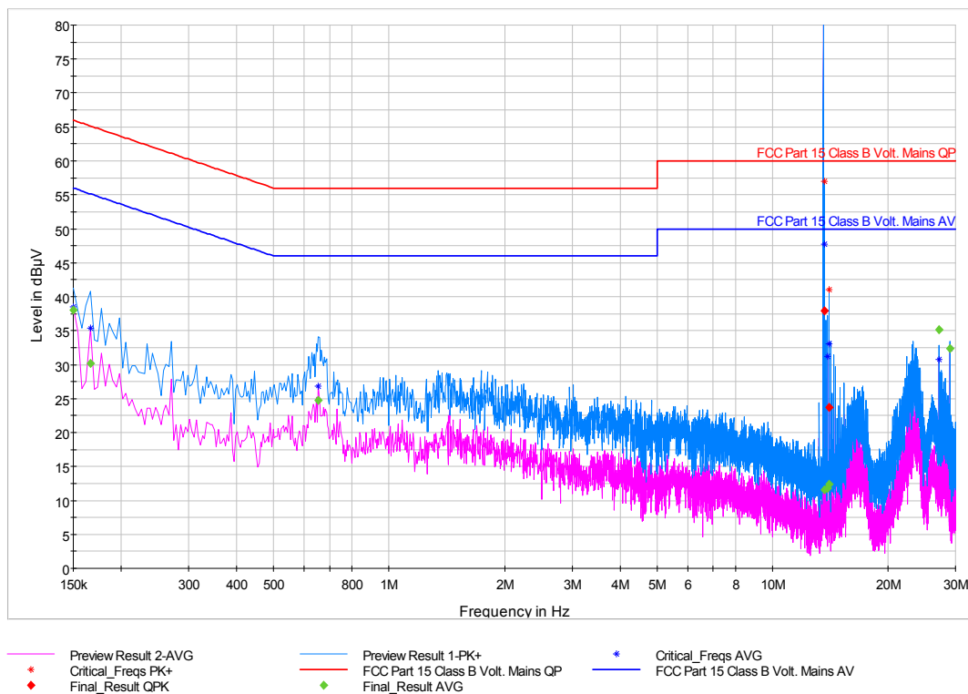
Figure 7-13: Conducted Emissions (150 kHz – 30 MHz), Neutral line – Configuration. 12, Bottom antenna (240 V / 60 Hz)
