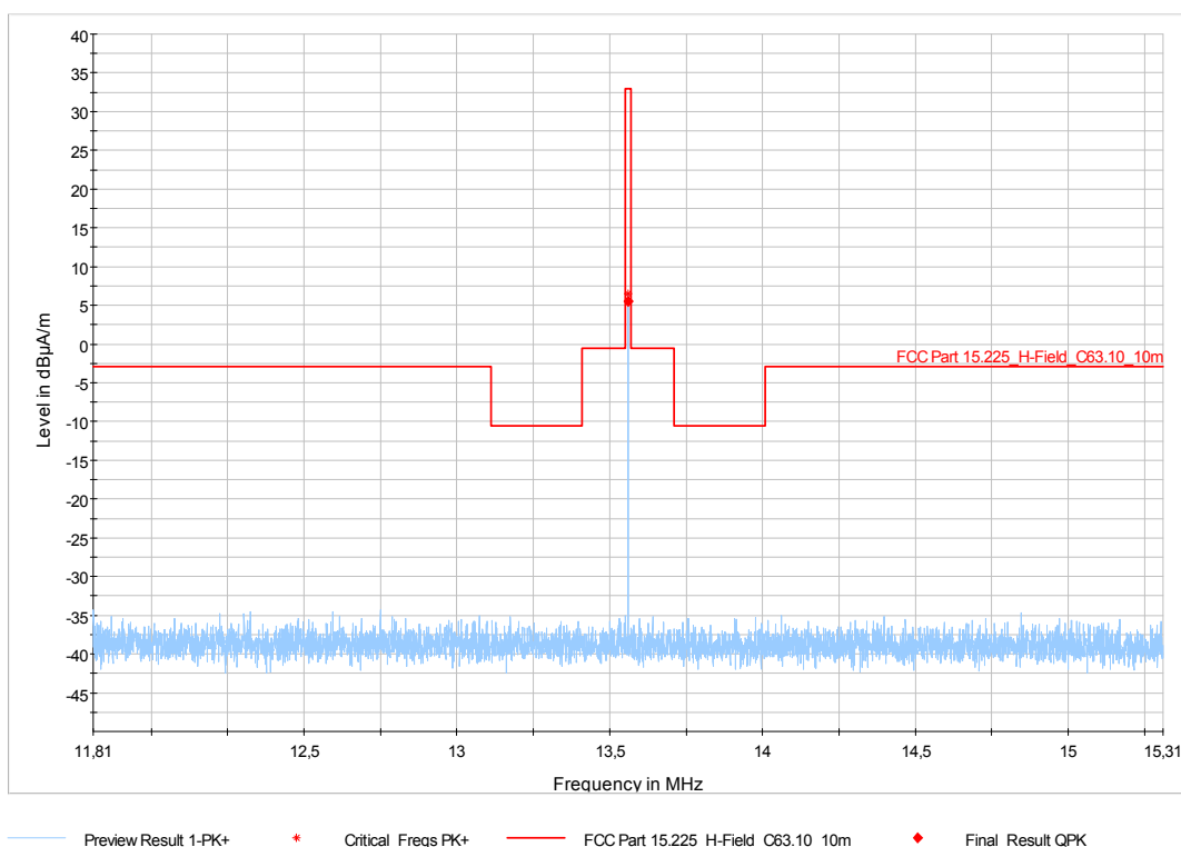
Figure 7-30: Radiated Emissions – 11.810 MHz to 15.310 MHz (§ 15.225a-c) – Configuration 5; Vertical Polarization
