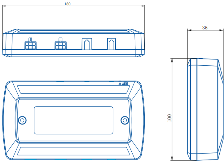
JCB35H7A1dimension and connection
