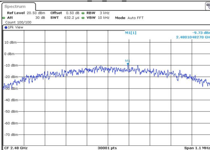
BLE_1M_Ant1_2480
