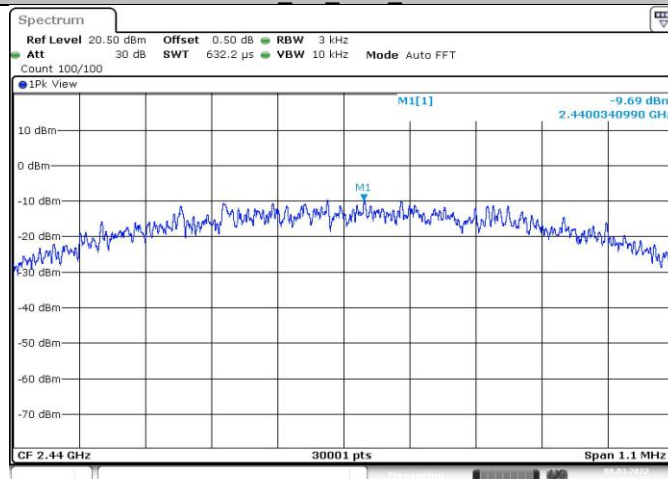
BLE_1M_Ant1_2440
