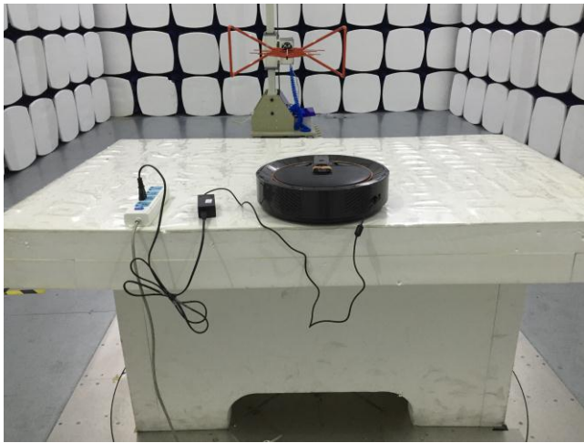
Radiated Emissions Test Setup Below 1GHz(With Direct Charging Mode)
