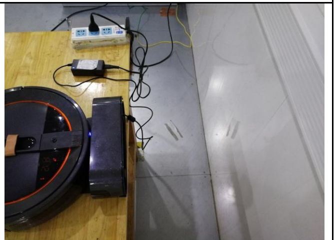
Conducted Emissions Test Setup – Side View(With Charging base Mode)
