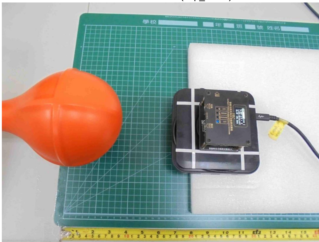
E-Field and H-Field (Top_20cm)
