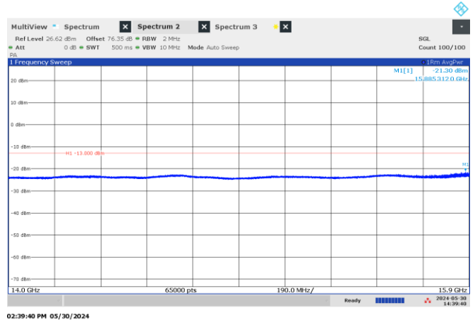
Figure 8.4-70: Emission mask, beyond \pm 250\% of BW (low frequency range), High channel: 16.40 GHz, shortest pulse. (200 MHz BW)
