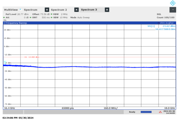
Figure 8.4-66: Emission mask, beyond \pm 250\% of BW (high frequency range), Low channel: 15.90 GHz, shortest pulse. (200 MHz BW)
