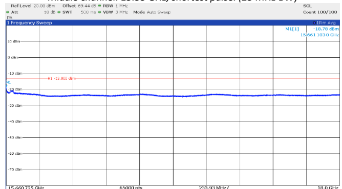
Figure 8.4-30: Emission mask, beyond ±250% of BW (high frequency range), Middle channel: 15.55 GHz, shortest pulse. (25 MHz BW)
