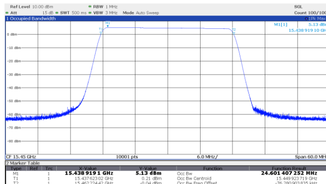
Figure 8.1-1: 99% OBW Low channel: 15.45 GHz, longest pulse (25 MHz BW)
