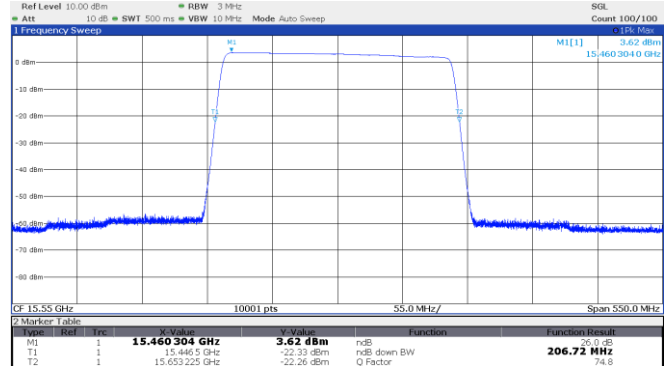
Figure 8.2-16: 26 dB OBW Middle channel: 15.55 GHz, shortest pulse (200 MHz BW)
