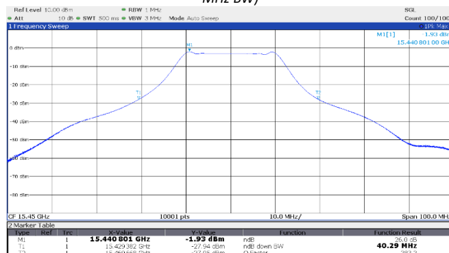
Figure 8.2-9: 26 dB OBW Low channel: 15.45 GHz, shortest pulse (25 MHz BW)
