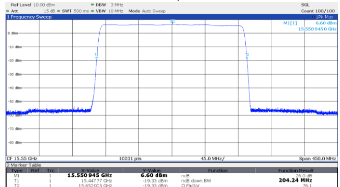
Figure 8.2-8: 26 dB OBW Middle channel: 15.55 GHz, longest pulse (200 MHz BW)
