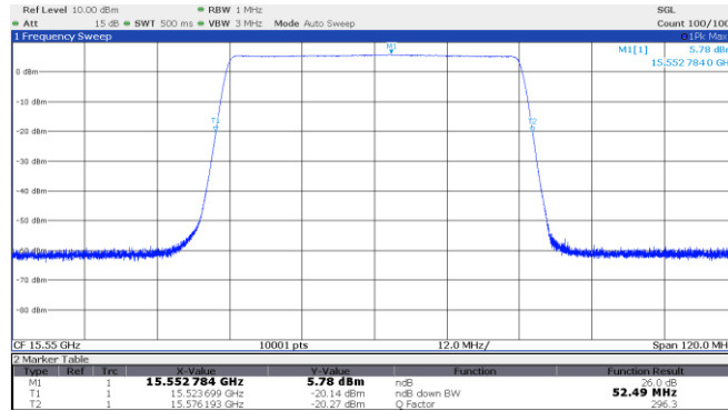
Figure 8.2-5: 26 dB OBW Middle channel: 15.55 GHz, longest pulse (50 MHz BW)
