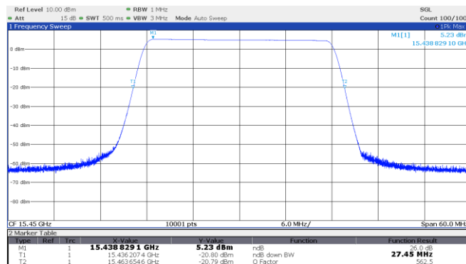
Figure 8.2-1: 26 dB OBW Low channel: 15.45 GHz, longest pulse (25 MHz BW)
