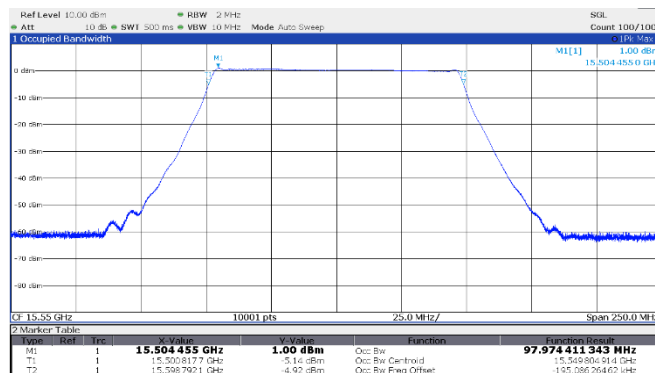
Figure 8.1-15: 99% OBW Middle channel: 15.55 GHz, shortest pulse (100 MHz BW)
