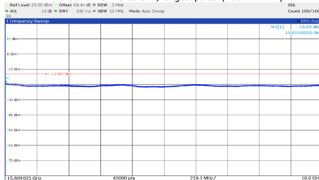
Figure 8.4-21: Emission mask, beyond \pm 250\% of BW (high frequency range), Middle channel: 15.55 GHz, longest pulse. (100 MHz BW)
