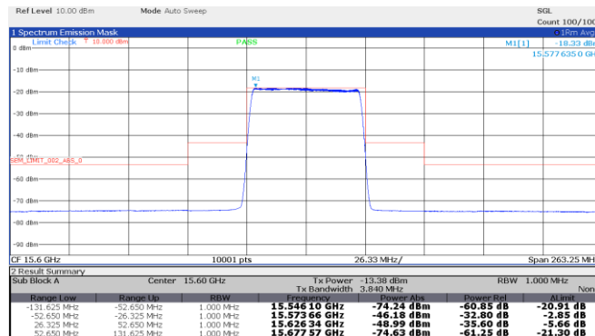
Figure 8.4-17: Emission mask, High channel: 15.60 GHz, longest pulse. (50 MHz BW)
