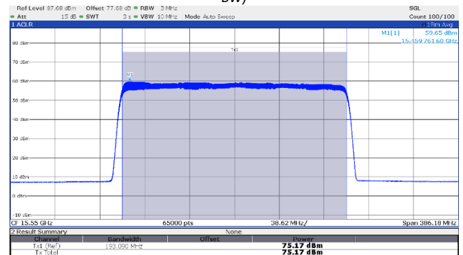
Figure 8.3-8: EIRP Power, Middle channel: 15.55 GHz, longest pulse (200 MHz BW)
