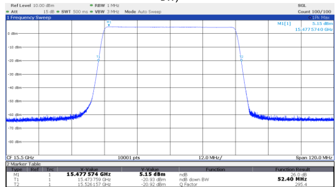
Figure 8.2-4: 26 dB OBW Low channel: 15.50 GHz, longest pulse (50 MHz BW)
