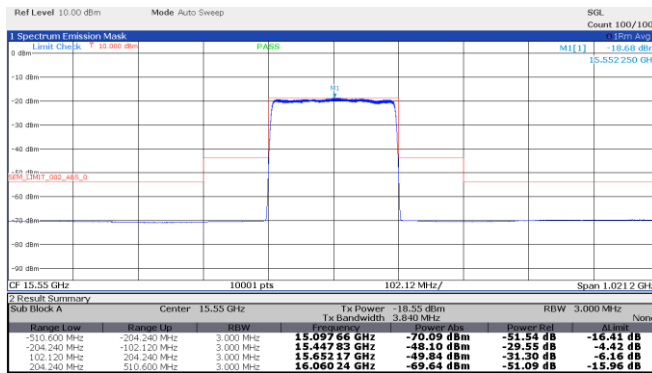
Figure 8.4-23: Emission mask, Middle channel: 15.55 GHz, longest pulse. (200 MHz BW)
