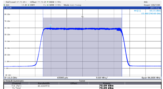
Figure 8.3-4: EIRP Power, Low channel: 15.50 GHz, longest pulse (50 MHz BW)
