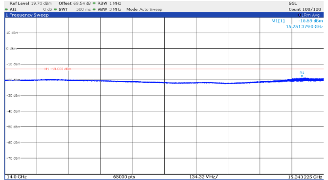
Figure 8.4-34: Emission mask, beyond \pm 250\% of BW (low frequency range), Low channel: 15.50 GHz, shortest pulse. (50 MHz BW)
