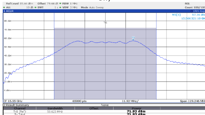
Figure 8.3-13: EIRP Power, Middle channel: 15.55 GHz, shortest pulse (50 MHz BW)
