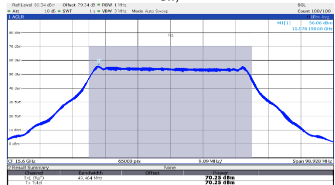
Figure 8.3-14: EIRP Power, High channel: 15.60 GHz, shortest pulse (50 MHz BW)
