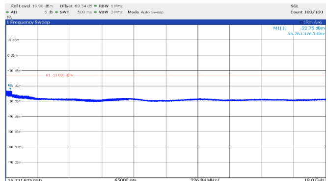
Figure 8.4-18: Emission mask, beyond \pm 250\% of BW (high frequency range), High channel: 15.60 GHz, longest pulse. (50 MHz BW)
