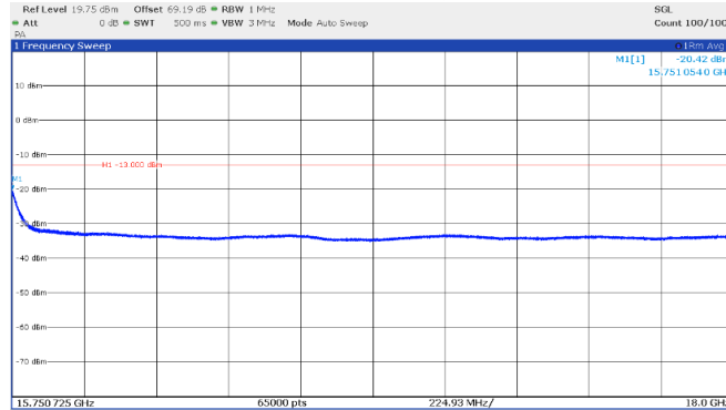
Figure 8.4-33: Emission mask, beyond \pm 250\% of BW (high frequency range), High channel: 15.65 GHz, shortest pulse. (25 MHz BW)
