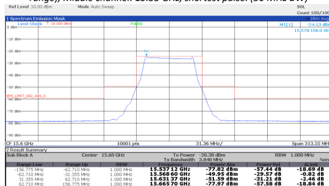
Figure 8.4-41: Emission mask, High channel: 15.60 GHz, shortest pulse. (50 MHz BW)
