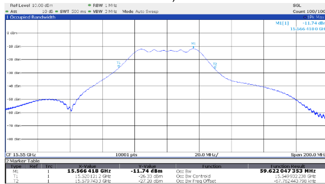
Figure 8.1-13: 99% OBW Middle channel: 15.55 GHz, shortest pulse (50 MHz BW)
