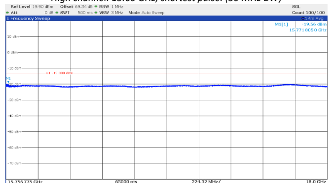
Figure 8.4-42: Emission mask, beyond \pm 250\% of BW (high frequency range), High channel: 15.60 GHz, shortest pulse. (50 MHz BW)
