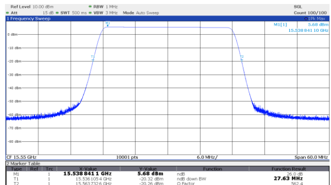
Figure 8.2-2: 26 dB OBW Middle channel: 15.55 GHz, longest pulse (25 MHz BW)
