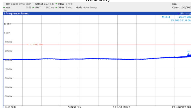
Figure 8.4-13: Emission mask, beyond \pm 250\% of BW (low frequency range), Middle channel: 15.55 GHz, longest pulse. (50 MHz BW)
