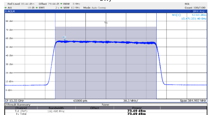
Figure 8.3-16: EIRP Power, Middle channel: 15.55 GHz, shortest pulse (200 MHz BW)
