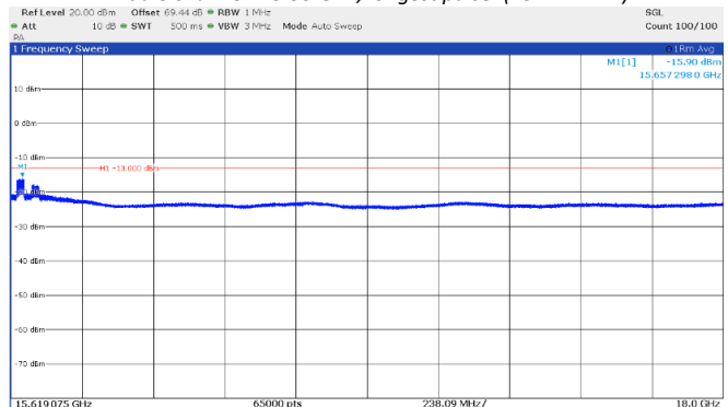
Figure 8.4-6: Emission mask, beyond \pm 250\% of BW (high frequency range), Middle channel: 15.55 GHz, longest pulse. (25 MHz BW)
