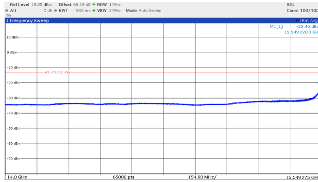
Figure 8.4-31: Emission mask, beyond \pm 250\% of BW (low frequency range), High channel: 15.65 GHz, shortest pulse. (25 MHz BW)
