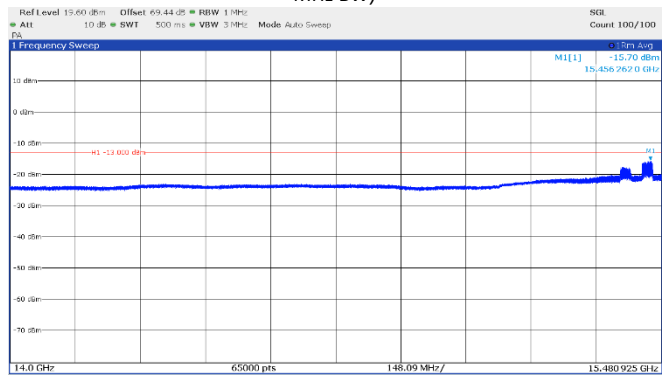
Figure 8.4-4: Emission mask, beyond \pm 250\% of BW (low frequency range), Middle channel: 15.55 GHz, longest pulse. (25 MHz BW)
