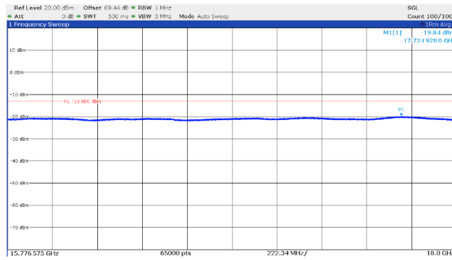
Figure 8.4-39: Emission mask, beyond \pm 250\% of BW (high frequency range), Middle channel: 15.55 GHz, shortest pulse. (50 MHz BW)
