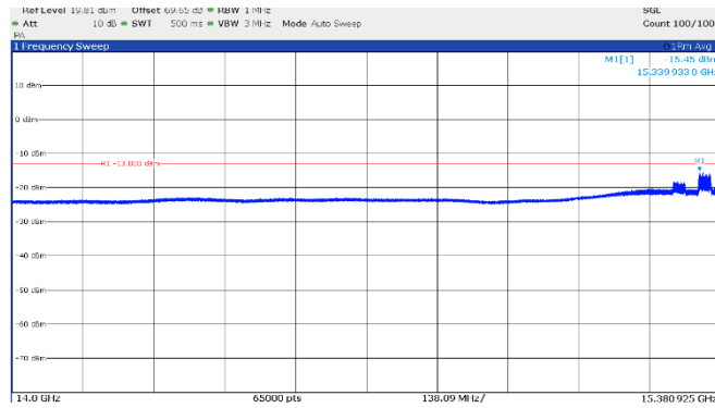
Figure 8.4-1: Emission mask, beyond \pm 250\% of BW (low frequency range), Low channel: 15.45 GHz, longest pulse. (25 MHz BW)
