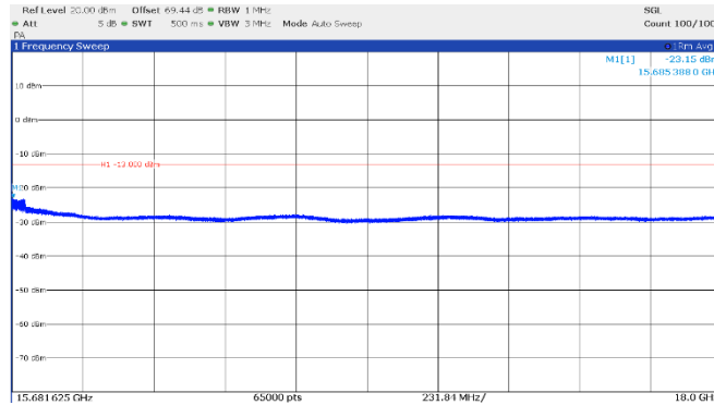
Figure 8.4-15: Emission mask, beyond \pm 250\% of BW (high frequency range), Middle channel: 15.55 GHz, longest pulse. (50 MHz BW)
