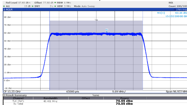
Figure 8.3-5: EIRP Power, Middle channel: 15.55 GHz, longest pulse (50 MHz BW)
