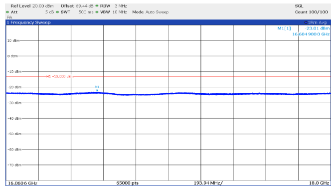
Figure 8.4-24: Emission mask, beyond ±250% of BW (high frequency range), Middle channel: 15.55 GHz, longest pulse. (200 MHz BW)
