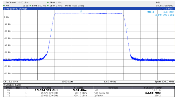
Figure 8.2-6: 26 dB OBW High channel: 15.60 GHz, longest pulse (50 MHz BW)
