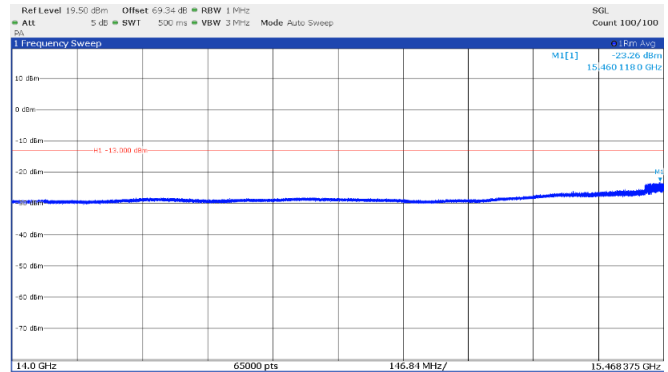
Figure 8.4-16: Emission mask, beyond \pm 250\% of BW (low frequency range), High channel: 15.60 GHz, longest pulse. (50 MHz BW)
