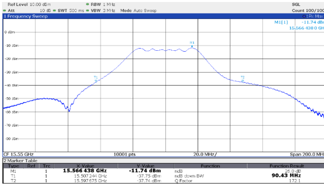
Figure 8.2-13: 26 dB OBW Middle channel: 15.55 GHz, shortest pulse (50 MHz BW)
