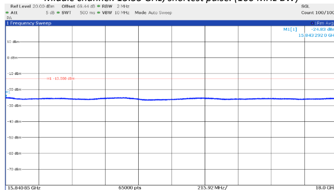
Figure 8.4-45: Emission mask, beyond \pm 250\% of BW (high frequency range), Middle channel: 15.55 GHz, shortest pulse. (100 MHz BW)
