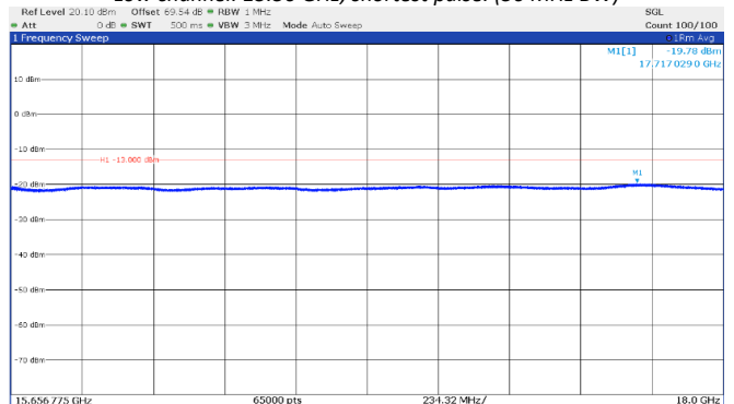
Figure 8.4-36: Emission mask, beyond \pm 250\% of BW (high frequency range), Low channel: 15.50 GHz, shortest pulse. (50 MHz BW)
