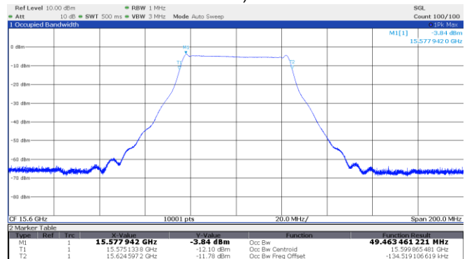
Figure 8.1-14: 99% OBW High channel: 15.60 GHz, shortest pulse (50 MHz BW)
