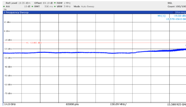
Figure 8.4-7: Emission mask, beyond \pm 250\% of BW (low frequency range), High channel: 15.65 GHz, longest pulse. (25 MHz BW)
