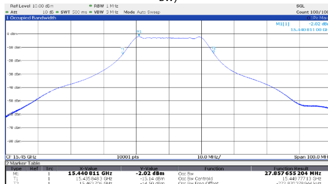
Figure 8.1-9: 99% OBW Low channel: 15.45 GHz, shortest pulse (25 MHz BW)
