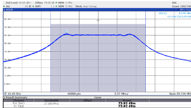
Figure 8.3-9: EIRP Power, Low channel: 15.45 GHz, shortest pulse (25 MHz BW)
