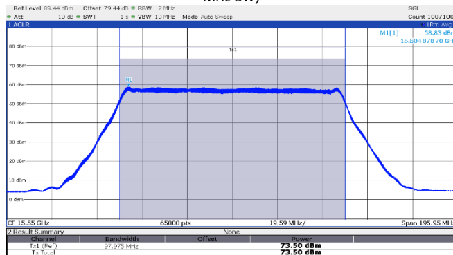
Figure 8.3-15: EIRP Power, Middle channel: 15.55 GHz, shortest pulse (100 MHz BW)
