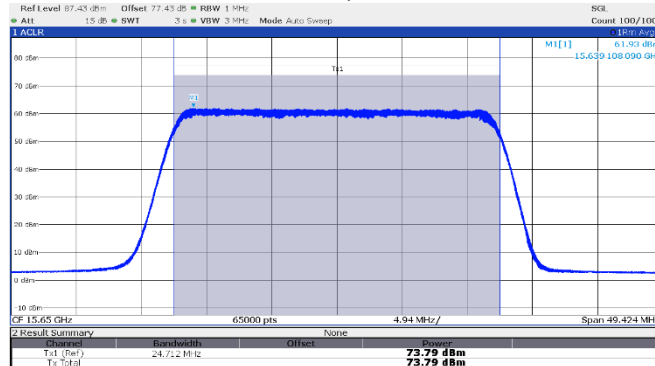
Figure 8.3-3: EIRP Power, High channel: 15.65 GHz, longest pulse (25 MHz BW)
