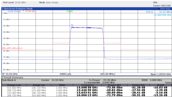
Figure 8.4-47: Emission mask, Middle channel: 15.55 GHz, shortest pulse. (200 MHz BW)
