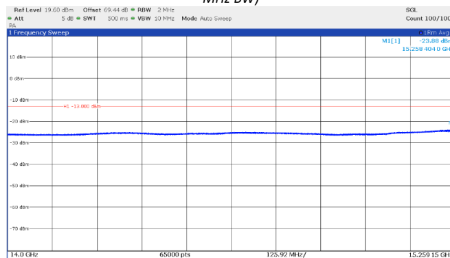
Figure 8.4-43: Emission mask, beyond \pm 250\% of BW (low frequency range), Middle channel: 15.55 GHz, shortest pulse. (100 MHz BW)
