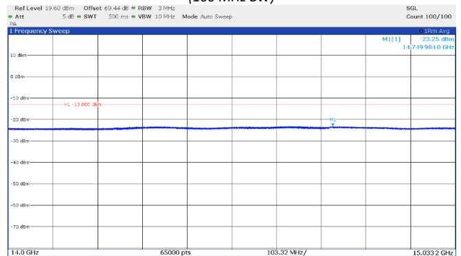
Figure 8.4-46: Emission mask, beyond \pm 250\% of BW (low frequency range), Middle channel: 15.55 GHz, shortest pulse. (200 MHz BW)
