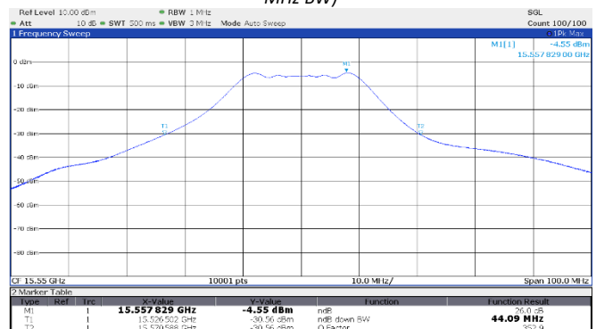
Figure 8.2-10: 26 dB OBW Middle channel: 15.55 GHz, shortest pulse (25 MHz BW)
