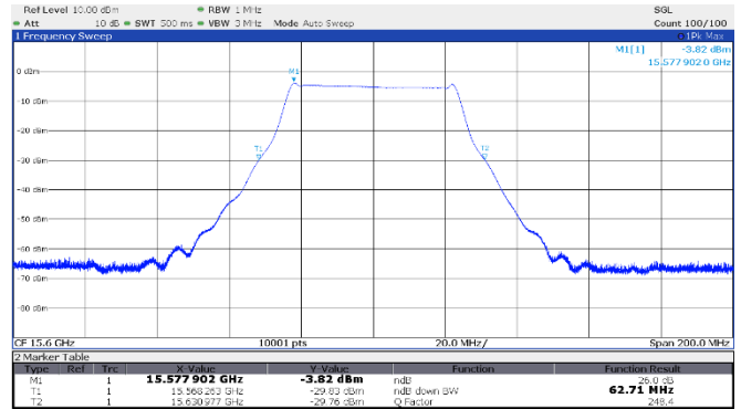
Figure 8.2-14: 26 dB OBW High channel: 15.60 GHz, shortest pulse (50 MHz BW)
