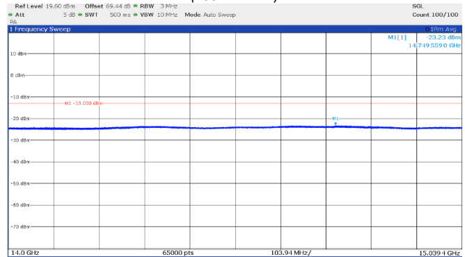
Figure 8.4-22: Emission mask, beyond \pm 250\% of BW (low frequency range), Middle channel: 15.55 GHz, longest pulse. (200 MHz BW)
