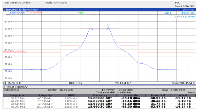
Figure 8.4-32: Emission mask, High channel: 15.65 GHz, shortest pulse. (25 MHz BW)
