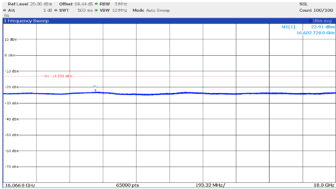
Figure 8.4-48: Emission mask, beyond ±250% of BW (high frequency range), Middle channel: 15.55 GHz, shortest pulse. (200 MHz BW)
