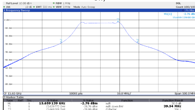
Figure 8.2-11: 26 dB OBW High channel: 15.65 GHz, shortest pulse (25 MHz BW)
