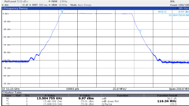
Figure 8.2-15: 26 dB OBW Middle channel: 15.55 GHz, shortest pulse (100 MHz BW)
