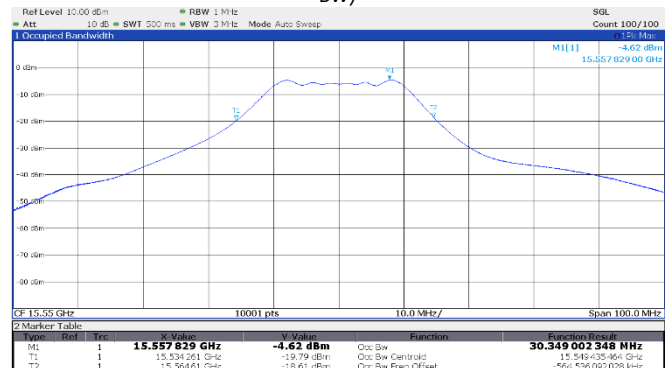
Figure 8.1-10: 99% OBW Middle channel: 15.55 GHz, shortest pulse (25 MHz BW)
