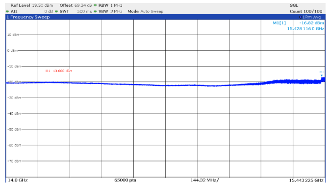
Figure 8.4-40: Emission mask, beyond \pm 250\% of BW (low frequency range), High channel: 15.60 GHz, shortest pulse. (50 MHz BW)
