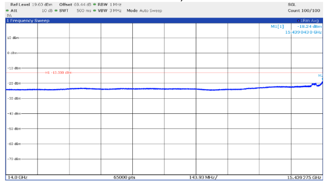
Figure 8.4-28: Emission mask, beyond ±250% of BW (low frequency range), Middle channel: 15.55 GHz, shortest pulse. (25 MHz BW)
