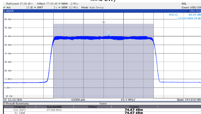
Figure 8.3-7: EIRP Power, Middle channel: 15.55 GHz, longest pulse (100 MHz BW)
