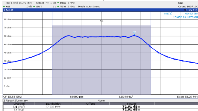
Figure 8.3-11: EIRP Power, High channel: 15.65 GHz, shortest pulse (25 MHz BW)
