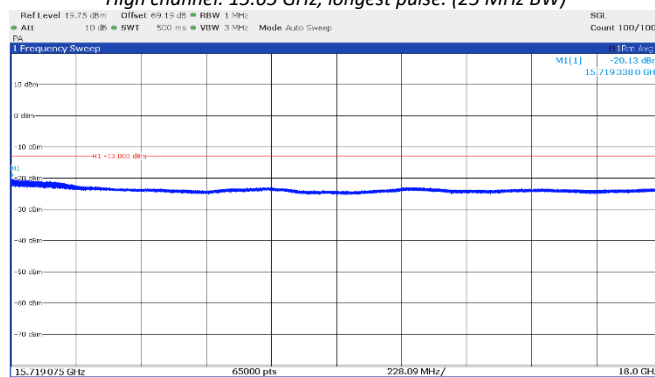
Figure 8.4-9: Emission mask, beyond \pm 250\% of BW (high frequency range), High channel: 15.65 GHz, longest pulse. (25 MHz BW)
