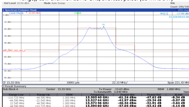
Figure 8.4-29: Emission mask, Middle channel: 15.55 GHz, shortest pulse. (25 MHz BW). RBW/2 Added at the edges.
