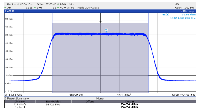
Figure 8.3-2: EIRP Power, Middle channel: 15.55 GHz, longest pulse (25 MHz BW)
