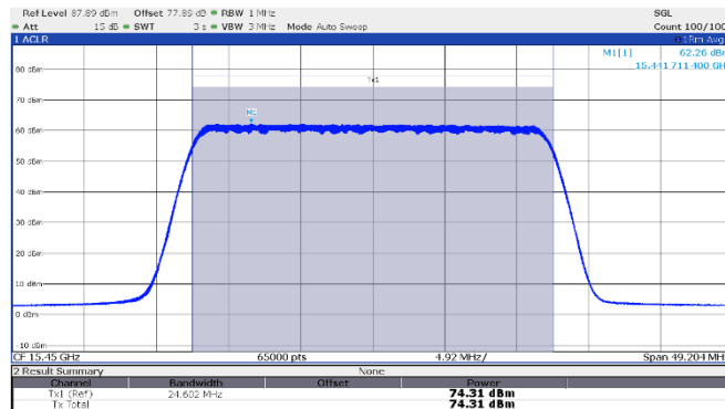
Figure 8.3-1: EIRP Power, Low channel: 15.45 GHz, longest pulse (25 MHz BW)
