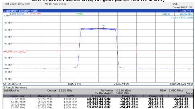
Figure 8.4-14: Emission mask, Middle channel: 15.55 GHz, longest pulse. (50 MHz BW)
