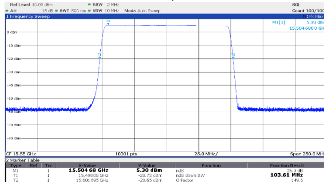
Figure 8.2-7: 26 dB OBW Middle channel: 15.55 GHz, longest pulse (100 MHz BW)
