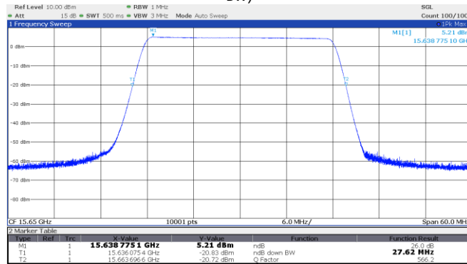
Figure 8.2-3: 26 dB OBW High channel: 15.65 GHz, longest pulse (25 MHz BW)
