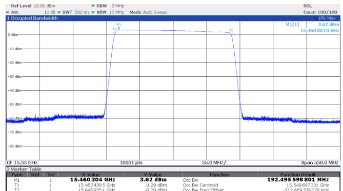
Figure 8.1-16: 99% OBW Middle channel: 15.55 GHz, shortest pulse (200 MHz BW)
