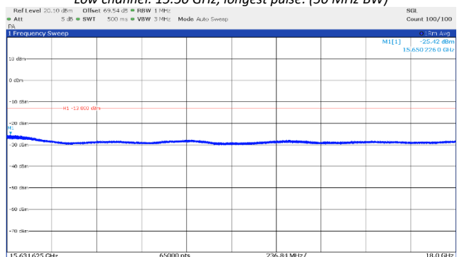
Figure 8.4-12: Emission mask, beyond \pm 250\% of BW (high frequency range), Low channel: 15.50 GHz, longest pulse. (50 MHz BW)
