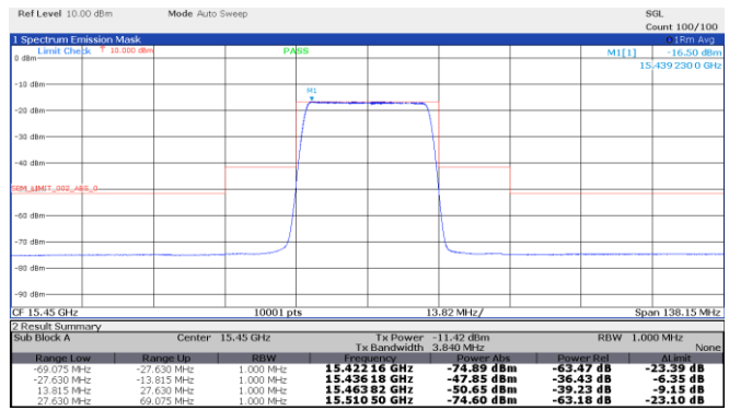
Figure 8.4-2: Emission mask, Low channel: 15.45 GHz, longest pulse. (25 MHz BW)
