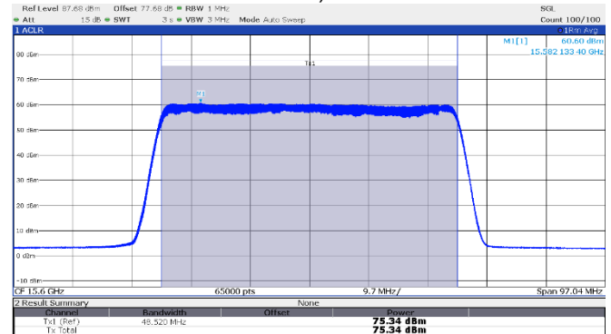
Figure 8.3-6: EIRP Power, High channel: 15.60 GHz, longest pulse (50 MHz BW)
