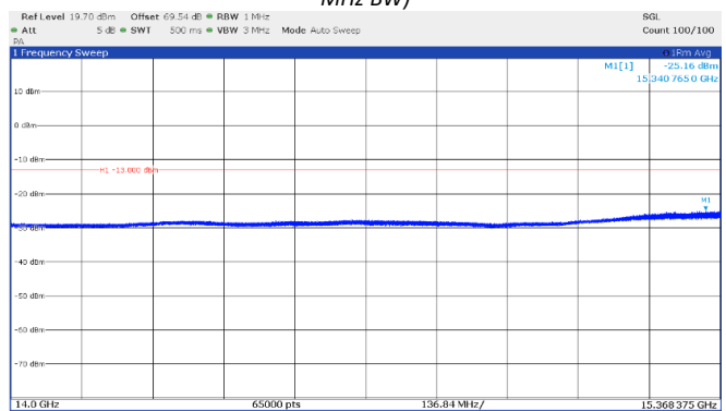
Figure 8.4-10: Emission mask, beyond \pm 250\% of BW (low frequency range), Low channel: 15.50 GHz, longest pulse. (50 MHz BW)
