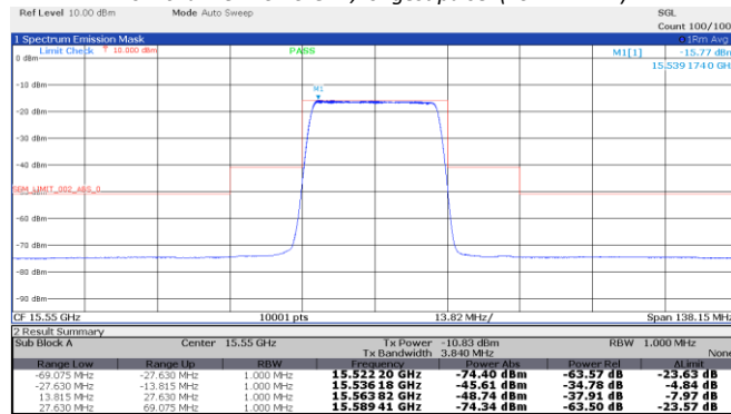
Figure 8.4-5: Emission mask, Middle channel: 15.55 GHz, longest pulse. (25 MHz BW)
