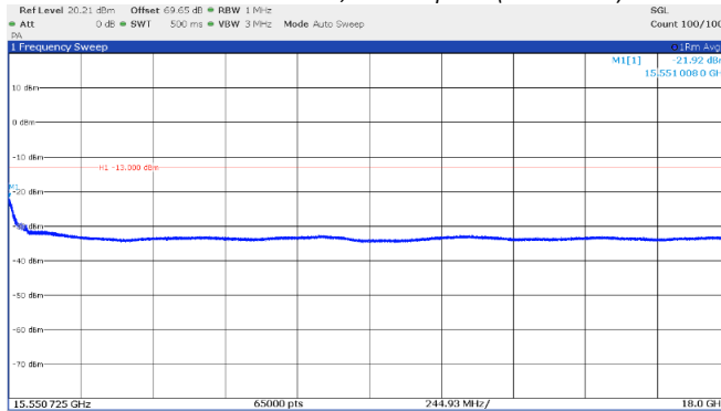
Figure 8.4-27: Emission mask, beyond ±250% of BW (high frequency range), Low channel: 15.45 GHz, shortest pulse. (25 MHz BW)
