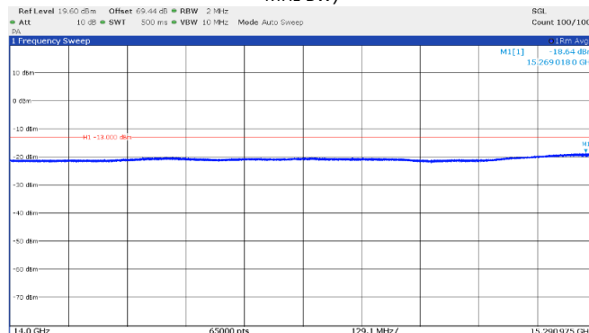
Figure 8.4-19: Emission mask, beyond \pm 250\% of BW (low frequency range), Middle channel: 15.55 GHz, longest pulse. (100 MHz BW)
