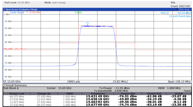
Figure 8.4-8: Emission mask, High channel: 15.65 GHz, longest pulse. (25 MHz BW)
