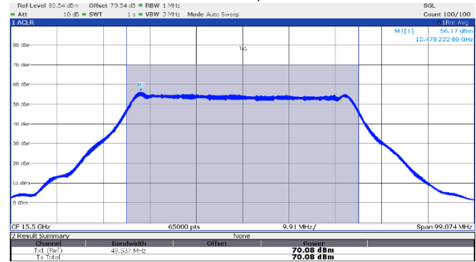
Figure 8.3-12: EIRP Power, Low channel: 15.50 GHz, shortest pulse (50 MHz BW)
