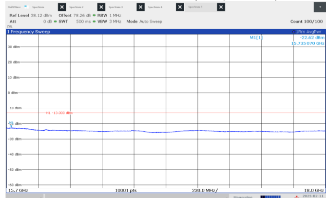
Figure 8.4-36: Emission mask, beyond \pm 250\% of BW (high frequency range), Low channel: 15.50 GHz, shortest pulse. (50 MHz BW)
