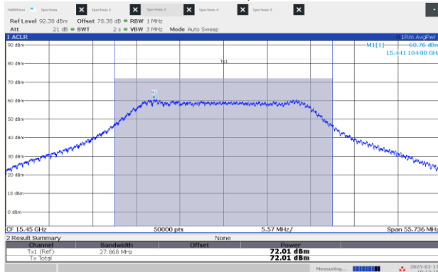
Figure 8.3-9: EIRP Power, Low channel: 15.45 GHz, shortest pulse (25 MHz BW)
