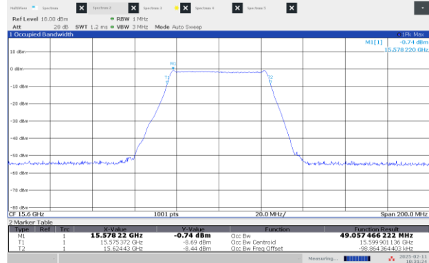
Figure 8.1-14: 99% OBW High channel: 15.60 GHz, shortest pulse (50 MHz BW)
