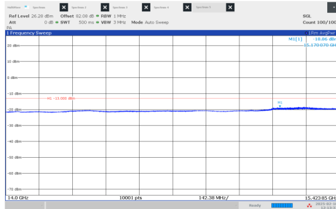
Figure 8.4-19: Emission mask, beyond \pm 250\% of BW (low frequency range), Middle channel: 15.55 GHz, longest pulse. (100 MHz BW)
