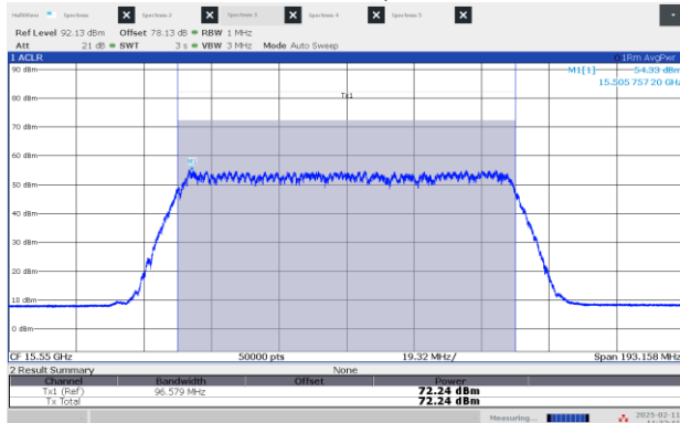
Figure 8.3-15: EIRP Power, Middle channel: 15.55 GHz, shortest pulse (100 MHz BW)
