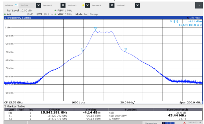
Figure 8.2-10: 26 dB OBW Middle channel: 15.55 GHz, shortest pulse (25 MHz BW)
