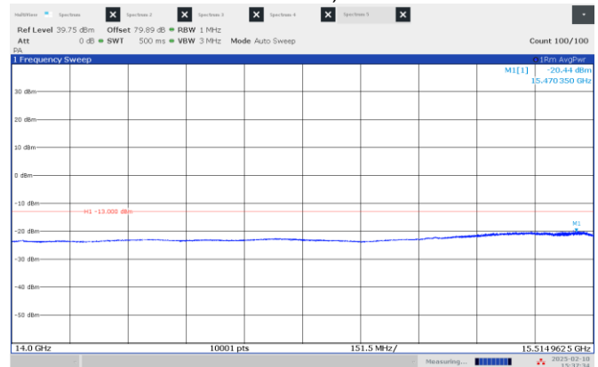
Figure 8.4-4: Emission mask, beyond \pm 250\% of BW (low frequency range), Middle channel: 15.55 GHz, longest pulse. (25 MHz BW)
