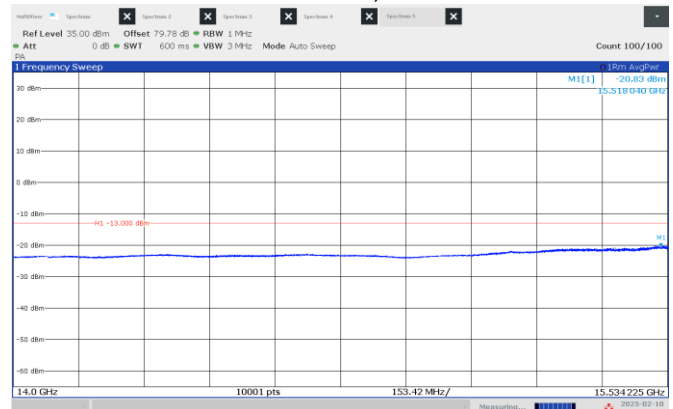
Figure 8.4-16: Emission mask, beyond \pm 250\% of BW (low frequency range), High channel: 15.60 GHz, longest pulse. (50 MHz BW)
