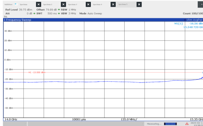
Figure 8.4-37: Emission mask, beyond \pm 250\% of BW (low frequency range), Middle channel: 15.55 GHz, shortest pulse. (50 MHz BW)
