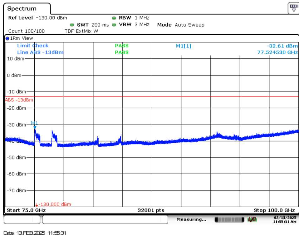
Figure 8.5-6: Radiated emissions spectral plot (75 GHz - 100 GHz) Vertical
