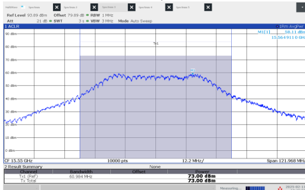
Figure 8.3-13: EIRP Power, Middle channel: 15.55 GHz, shortest pulse (50 MHz BW)
