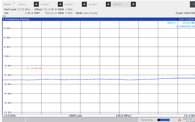
Figure 8.4-43: Emission mask, beyond \pm 250\% of BW (low frequency range), Middle channel: 15.55 GHz, shortest pulse. (100 MHz BW)
