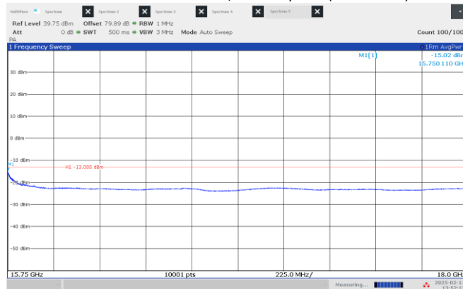
Figure 8.4-39: Emission mask, beyond \pm 250\% of BW (high frequency range), Middle channel: 15.55 GHz, shortest pulse. (50 MHz BW)
