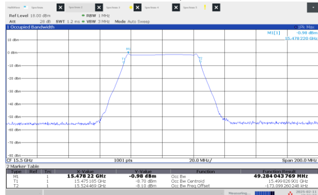
Figure 8.1-12: 99% OBW Low channel: 15.50 GHz, shortest pulse (50 MHz BW)
