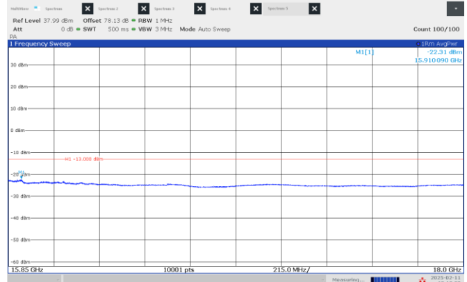
Figure 8.4-48: Emission mask, beyond \pm 250\% of BW (high frequency range), Middle channel: 15.55 GHz, shortest pulse. (200 MHz BW)
