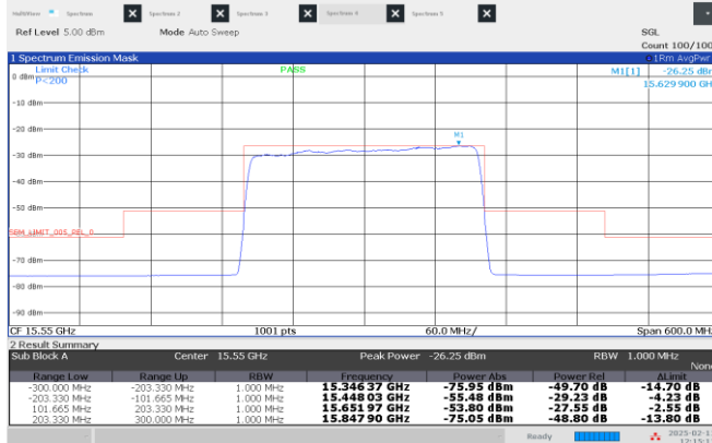
Figure 8.4-47: Emission mask, Middle channel: 15.55 GHz, shortest pulse. (200 MHz BW)
