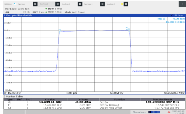
Figure 8.1-8: 99% OBW Middle channel: 15.55 GHz, longest pulse (200 MHz BW)
