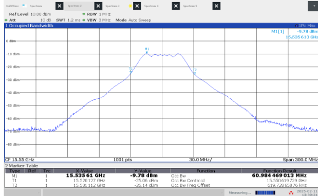
Figure 8.1-13: 99% OBW Middle channel: 15.55 GHz, shortest pulse (50 MHz BW)
