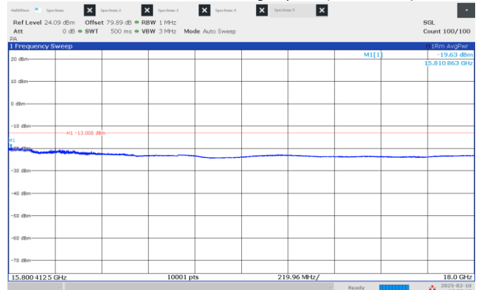
Figure 8.4-24: Emission mask, beyond \pm 250\% of BW (high frequency range), Middle channel: 15.55 GHz, longest pulse. (200 MHz BW)
