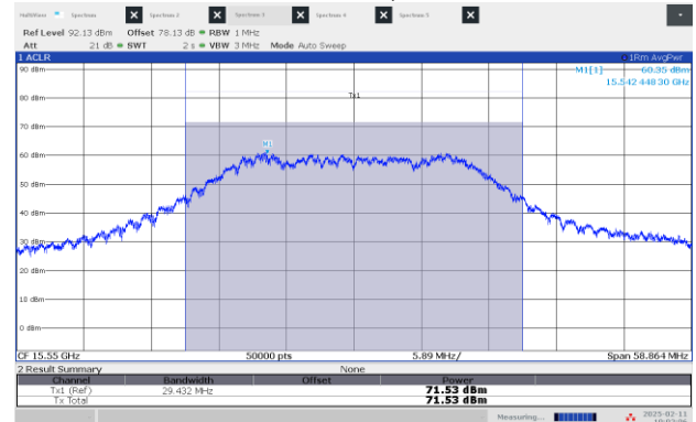
Figure 8.3-10: EIRP Power, Middle channel: 15.55 GHz, shortest pulse (25 MHz BW)
