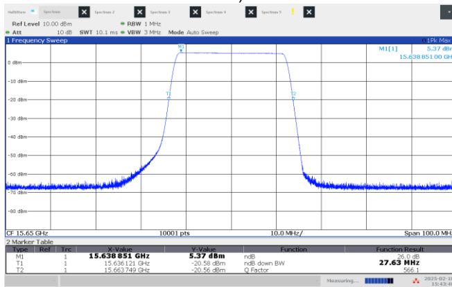
Figure 8.2-3: 26 dB OBW High channel: 15.65 GHz, longest pulse (25 MHz BW)
