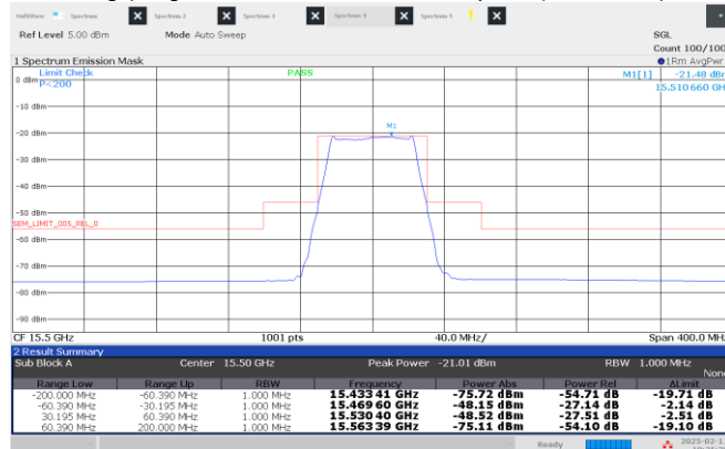
Figure 8.4-35: Emission mask, Low channel: 15.50 GHz, shortest pulse. (50 MHz BW)
