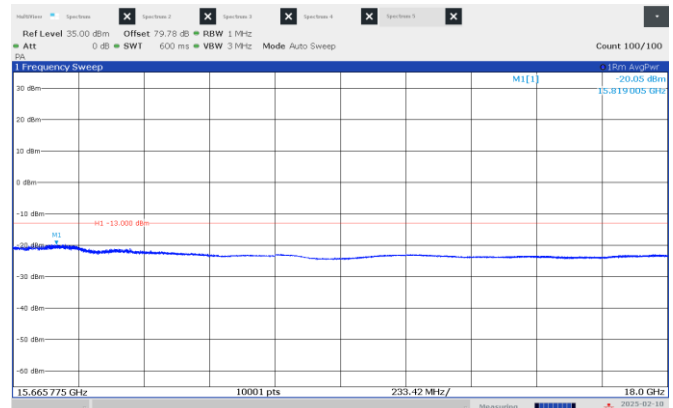
Figure 8.4-18: Emission mask, beyond \pm 250\% of BW (high frequency range), High channel: 15.60 GHz, longest pulse. (50 MHz BW)
