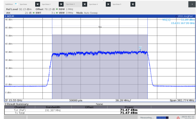
Figure 8.3-16: EIRP Power, Middle channel: 15.55 GHz, shortest pulse (200 MHz BW)
