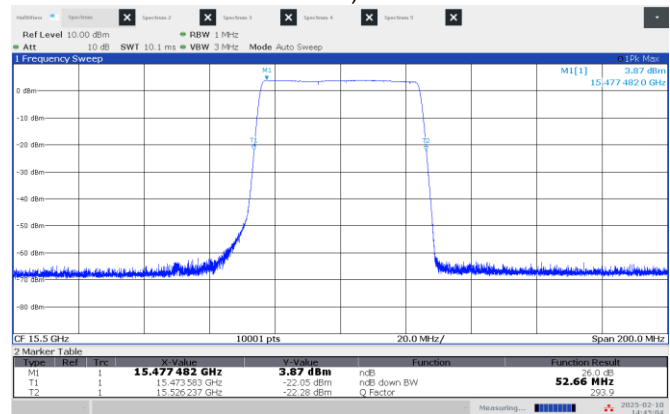
Figure 8.2-4: 26 dB OBW Low channel: 15.50 GHz, longest pulse (50 MHz BW)
