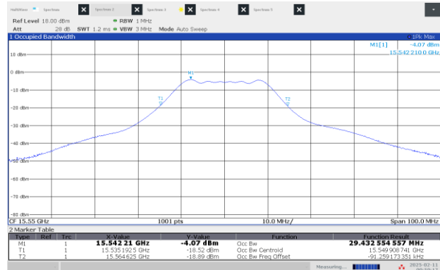
Figure 8.1-10: 99% OBW Middle channel: 15.55 GHz, shortest pulse (25 MHz BW)
