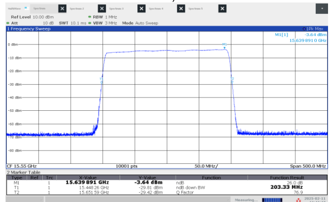
Figure 8.2-16: 26 dB OBW Middle channel: 15.55 GHz, shortest pulse (200 MHz BW)
