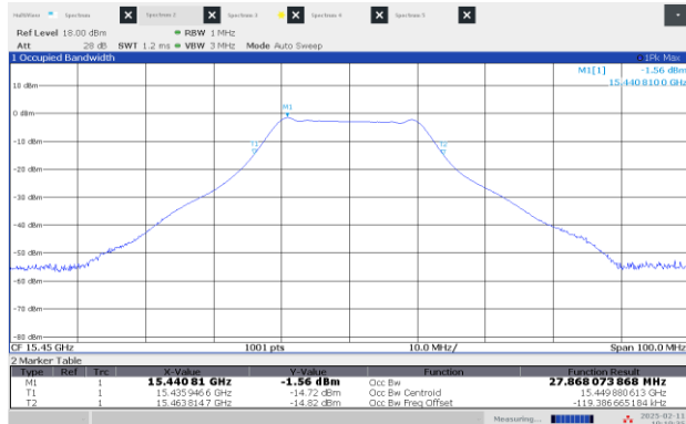
Figure 8.1-9: 99% OBW Low channel: 15.45 GHz, shortest pulse (25 MHz BW)
