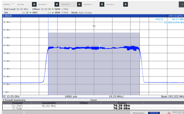
Figure 8.3-7: EIRP Power, Middle channel: 15.55 GHz, longest pulse (100 MHz BW)
