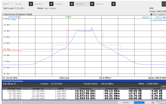
Figure 8.4-29: Emission mask, Middle channel: 15.55 GHz, shortest pulse. (25 MHz BW).
