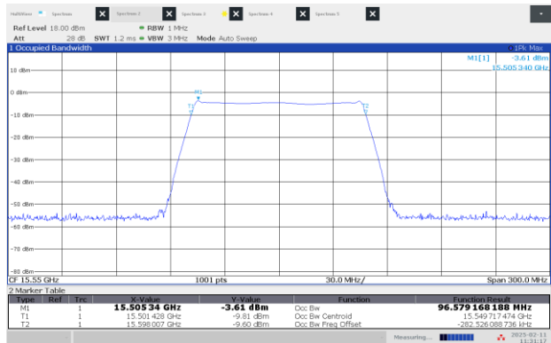
Figure 8.1-15: 99% OBW Middle channel: 15.55 GHz, shortest pulse (100 MHz BW)
