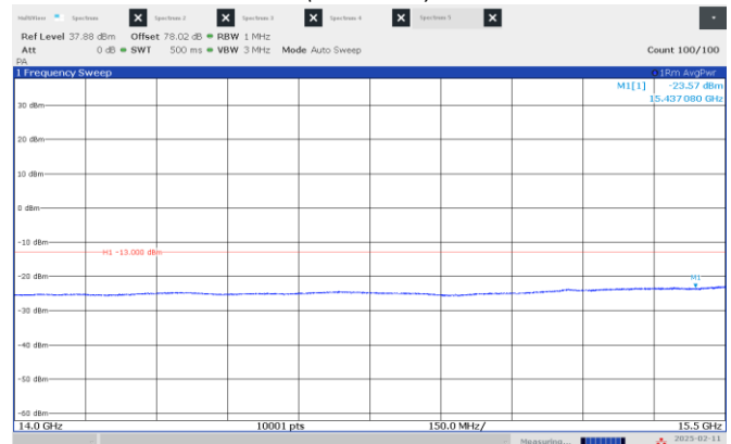
Figure 8.4-40: Emission mask, beyond \pm 250\% of BW (low frequency range), High channel: 15.60 GHz, shortest pulse. (50 MHz BW)
