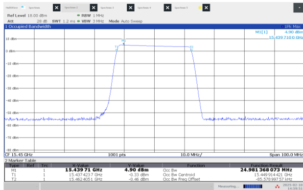
Figure 8.1-1: 99% OBW Low channel: 15.45 GHz, longest pulse (25 MHz BW)
