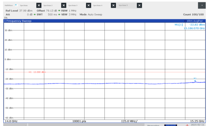
Figure 8.4-46: Emission mask, beyond \pm 250\% of BW (low frequency range), Middle channel: 15.55 GHz, shortest pulse. (200 MHz BW)
