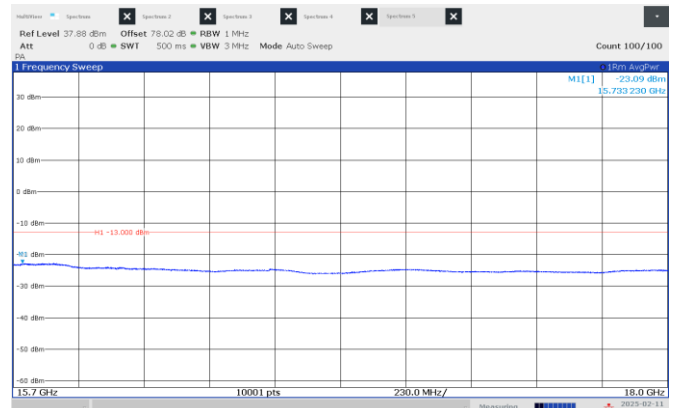
Figure 8.4-42: Emission mask, beyond \pm 250\% of BW (high frequency range), High channel: 15.60 GHz, shortest pulse. (50 MHz BW)
