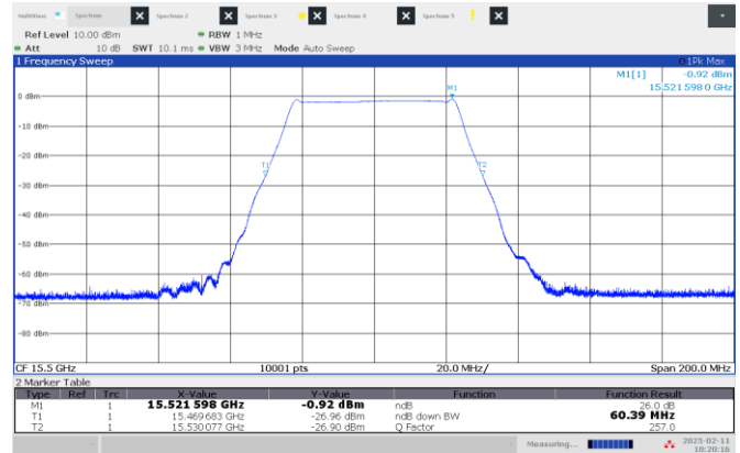
Figure 8.2-12: 26 dB OBW Low channel: 15.50 GHz, shortest pulse (50 MHz BW)
