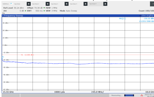
Figure 8.4-27: Emission mask, beyond \pm 250\% of BW (high frequency range), Low channel: 15.45 GHz, shortest pulse. (25 MHz BW)
