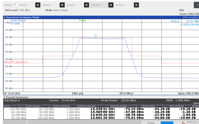
Figure 8.4-41: Emission mask, High channel: 15.60 GHz, shortest pulse. (50 MHz BW)
