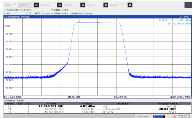
Figure 8.2-2: 26 dB OBW Middle channel: 15.55 GHz, longest pulse (25 MHz BW)
