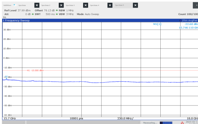
Figure 8.4-45: Emission mask, beyond \pm 250\% of BW (high frequency range), Middle channel: 15.55 GHz, shortest pulse. (100 MHz BW)
