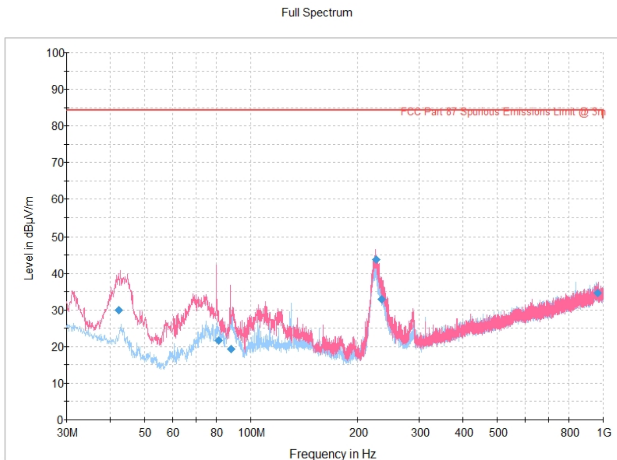
Figure 8.5-1: Radiated emissions spectral plot (30-1000MHz)
