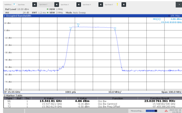
Figure 8.1-2: 99% OBW Middle channel: 15.55 GHz, longest pulse (25 MHz BW)
