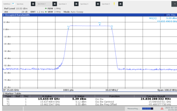
Figure 8.1-3: 99% OBW High channel: 15.65 GHz, longest pulse (25 MHz BW)
