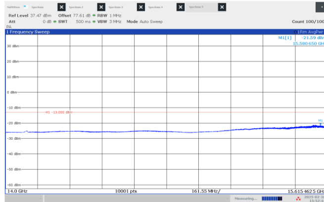
Figure 8.4-7: Emission mask, beyond \pm 250\% of BW (low frequency range), High channel: 15.65 GHz, longest pulse. (25 MHz BW)
