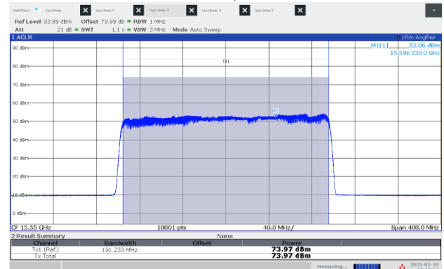
Figure 8.3-8: EIRP Power, Middle channel: 15.55 GHz, longest pulse (200 MHz BW)
