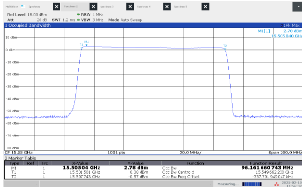
Figure 8.1-7: 99% OBW Middle channel: 15.55 GHz, longest pulse (100 MHz BW)
