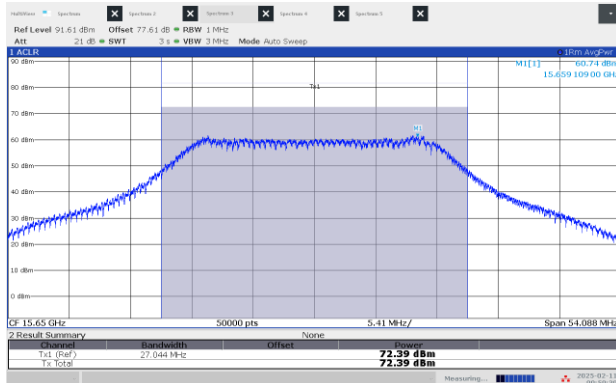
Figure 8.3-11: EIRP Power, High channel: 15.65 GHz, shortest pulse (25 MHz BW)
