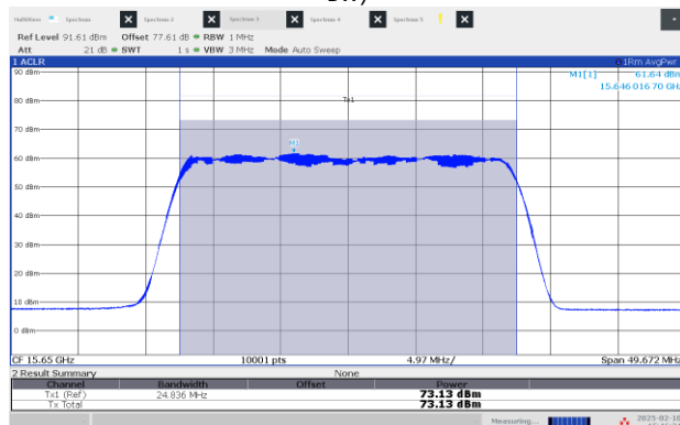
Figure 8.3-3: EIRP Power, High channel: 15.65 GHz, longest pulse (25 MHz BW)
