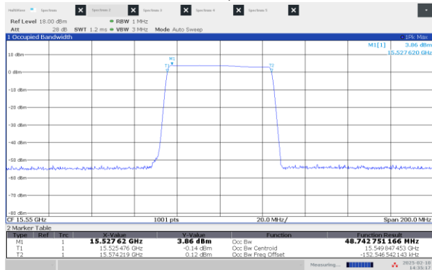
Figure 8.1-5: 99% OBW Middle channel: 15.55 GHz, longest pulse (50 MHz BW)
