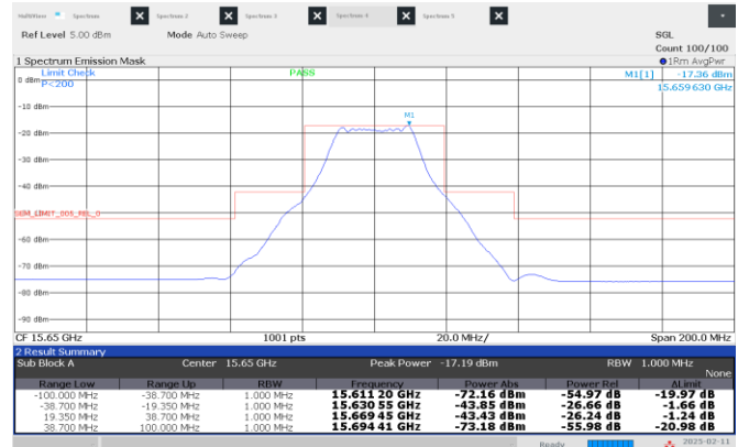
Figure 8.4-32: Emission mask, High channel: 15.65 GHz, shortest pulse. (25 MHz BW)
