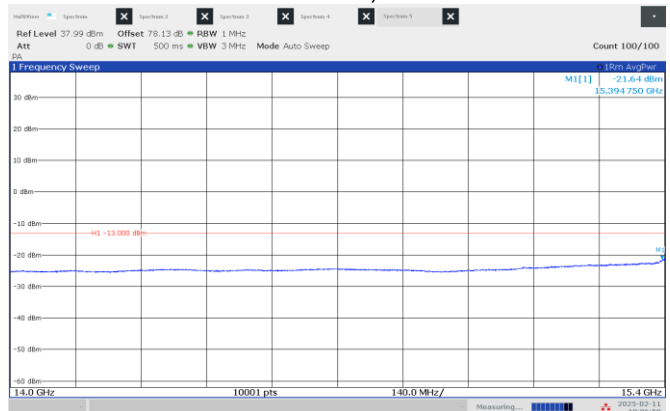
Figure 8.4-28: Emission mask, beyond \pm 250\% of BW (low frequency range), Middle channel: 15.55 GHz, shortest pulse. (25 MHz BW)
