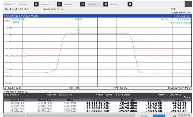
Figure 8.4-8: Emission mask, High channel: 15.65 GHz, longest pulse. (25 MHz BW)
