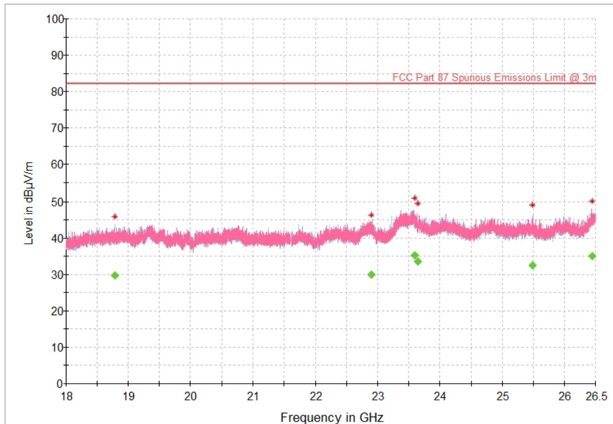
Figure 8.5-3: Radiated emissions spectral plot (18-26.5GHz)
