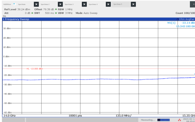
Figure 8.4-25: Emission mask, beyond \pm 250\% of BW (low frequency range), Low channel: 15.45 GHz, shortest pulse. (25 MHz BW)
