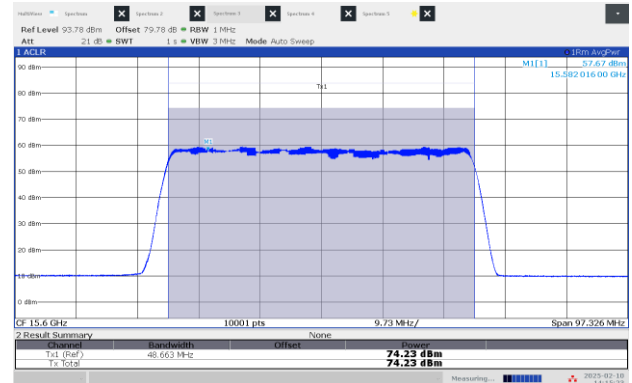
Figure 8.3-6: EIRP Power, High channel: 15.60 GHz, longest pulse (50 MHz BW)
