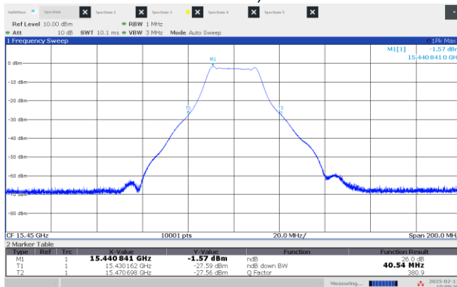
Figure 8.2-9: 26 dB OBW Low channel: 15.45 GHz, shortest pulse (25 MHz BW)
