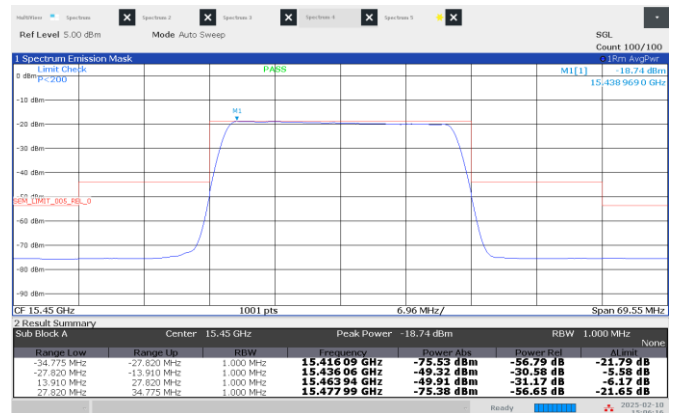
Figure 8.4-2: Emission mask, Low channel: 15.45 GHz, longest pulse. (25 MHz BW)
