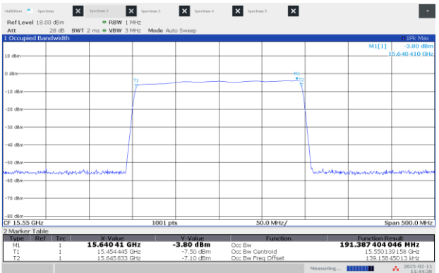
Figure 8.1-16: 99% OBW Middle channel: 15.55 GHz, shortest pulse (200 MHz BW)
