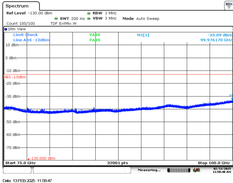
Figure 8.5-5: Radiated emissions spectral plot (75 GHz - 100 GHz) Horizontal
