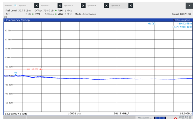
Figure 8.4-6: Emission mask, beyond \pm 250\% of BW (high frequency range), Middle channel: 15.55 GHz, longest pulse. (25 MHz BW)
