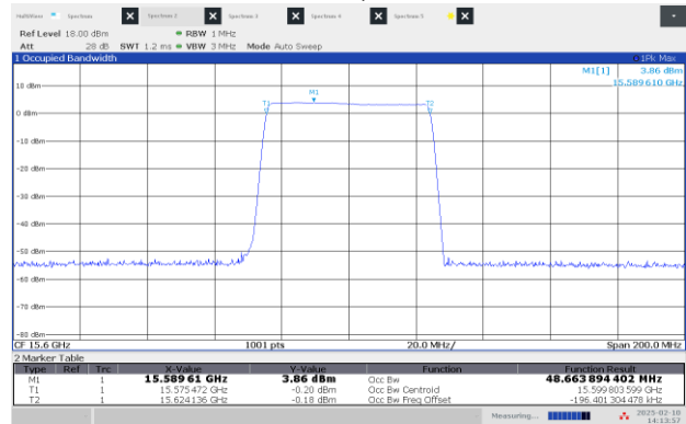
Figure 8.1-6: 99% OBW High channel: 15.60 GHz, longest pulse (50 MHz BW)
