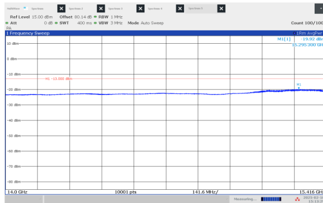
Figure 8.4-1: Emission mask, beyond \pm 250\% of BW (low frequency range), Low channel: 15.45 GHz, longest pulse. (25 MHz BW)
