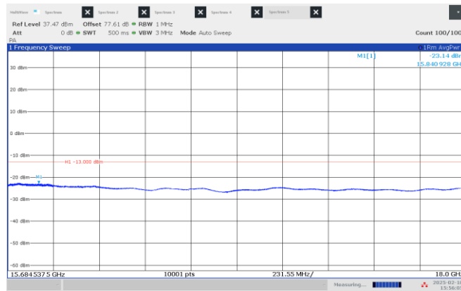
Figure 8.4-9: Emission mask, beyond \pm 250\% of BW (high frequency range), High channel: 15.65 GHz, longest pulse. (25 MHz BW)
