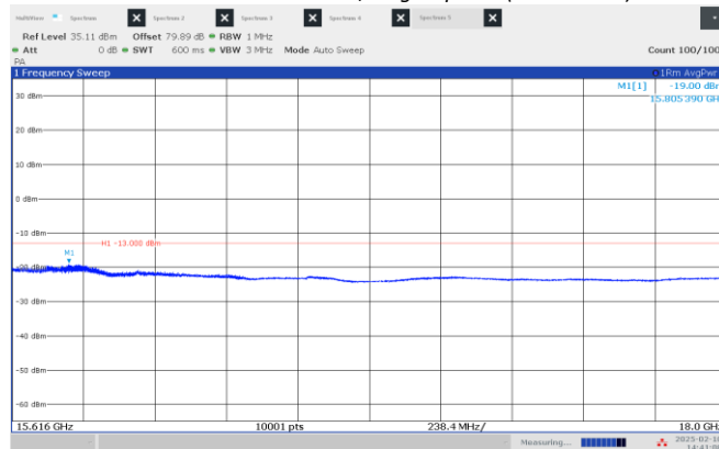
Figure 8.4-15: Emission mask, beyond \pm 250\% of BW (high frequency range), Middle channel: 15.55 GHz, longest pulse. (50 MHz BW)
