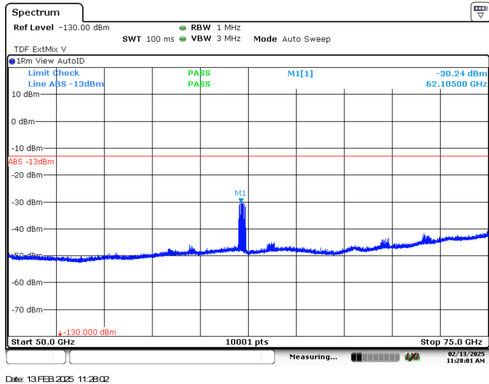
Figure 8.5-3: Radiated emissions spectral plot (50 GHz - 75 GHz) Horizontal
