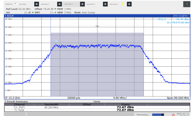
Figure 8.3-12: EIRP Power, Low channel: 15.50 GHz, shortest pulse (50 MHz BW)
