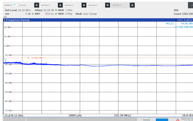
Figure 8.4-21: Emission mask, beyond \pm 250\% of BW (high frequency range), Middle channel: 15.55 GHz, longest pulse. (100 MHz BW)
