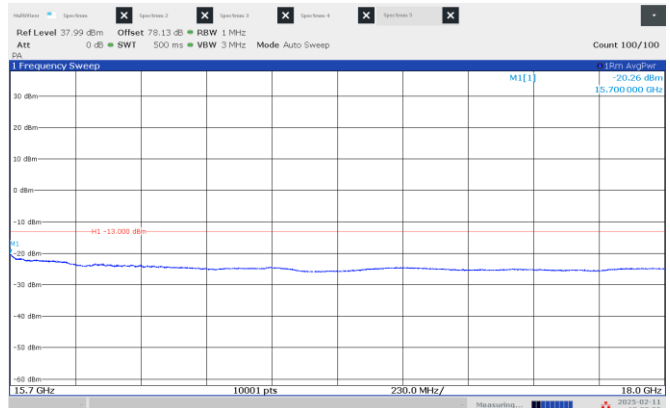
Figure 8.4-30: Emission mask, beyond \pm 250\% of BW (high frequency range), Middle channel: 15.55 GHz, shortest pulse. (25 MHz BW)
