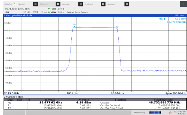
Figure 8.1-4: 99% OBW Low channel: 15.50 GHz, longest pulse (50 MHz BW)
