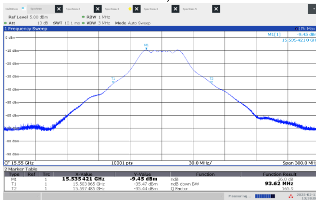
Figure 8.2-13: 26 dB OBW Middle channel: 15.55 GHz, shortest pulse (50 MHz BW)
