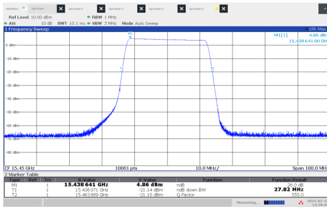
Figure 8.2-1: 26 dB OBW Low channel: 15.45 GHz, longest pulse (25 MHz BW)
