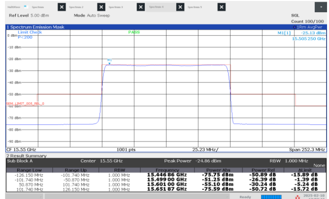
Figure 8.4-20: Emission mask, Middle channel: 15.55 GHz, longest pulse. (100 MHz BW)
