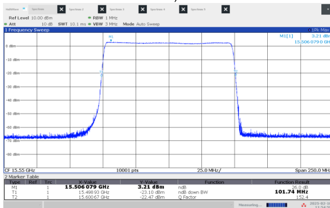
Figure 8.2-7: 26 dB OBW Middle channel: 15.55 GHz, longest pulse (100 MHz BW)
