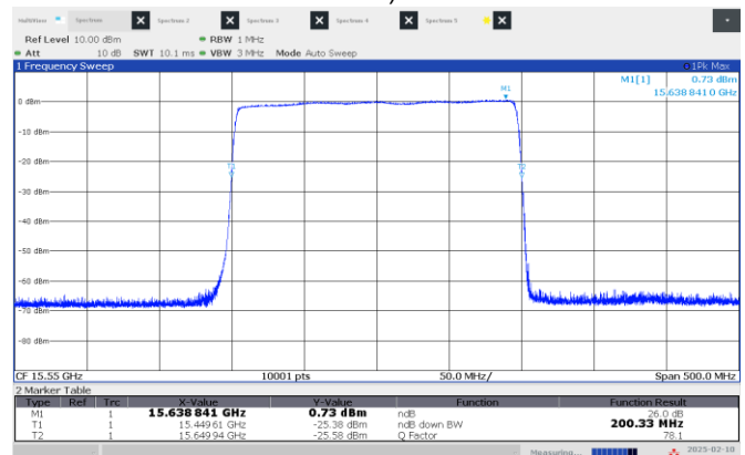
Figure 8.2-8: 26 dB OBW Middle channel: 15.55 GHz, longest pulse (200 MHz BW)
