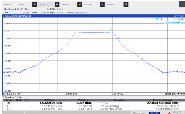
Figure 8.1-11: 99% OBW High channel: 15.65 GHz, shortest pulse (25 MHz BW)
