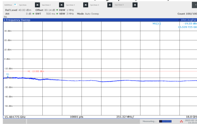
Figure 8.4-3: Emission mask, beyond \pm 250\% of BW (high frequency range), Low channel: 15.45 GHz, longest pulse. (25 MHz BW)
