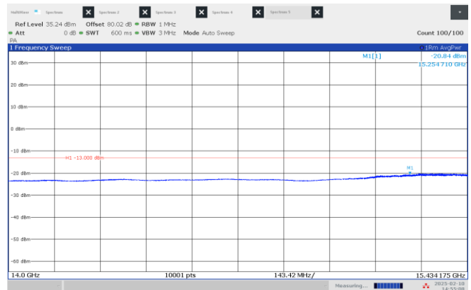
Figure 8.4-10: Emission mask, beyond \pm 250\% of BW (low frequency range), Low channel: 15.50 GHz, longest pulse. (50 MHz BW)
