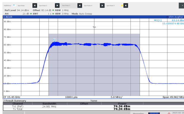
Figure 8.3-1: EIRP Power, Low channel: 15.45 GHz, longest pulse (25 MHz BW)
