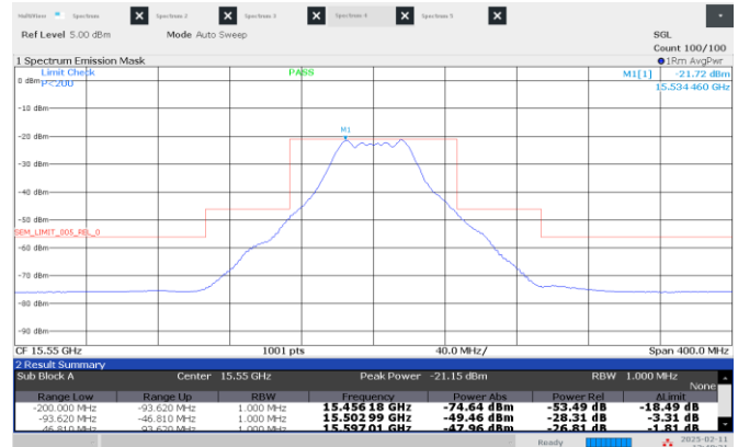
Figure 8.4-38: Emission mask, Middle channel: 15.55 GHz, shortest pulse. (50 MHz BW)
