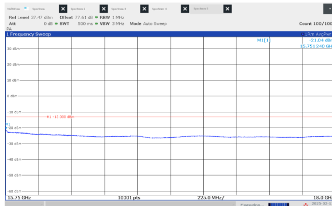
Figure 8.4-33: Emission mask, beyond \pm 250\% of BW (high frequency range), High channel: 15.65 GHz, shortest pulse. (25 MHz BW)
