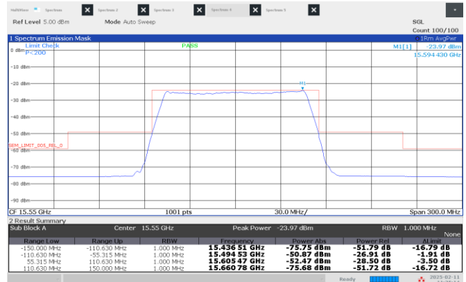
Figure 8.4-44: Emission mask, Middle channel: 15.55 GHz, shortest pulse. (100 MHz BW)
