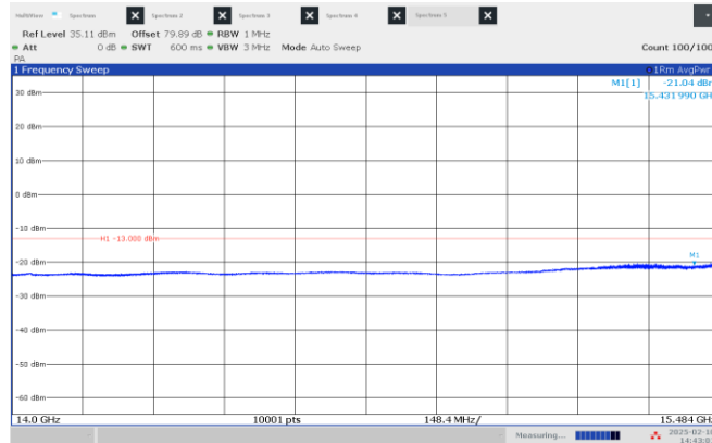
Figure 8.4-13: Emission mask, beyond \pm 250\% of BW (low frequency range), Middle channel: 15.55 GHz, longest pulse. (50 MHz BW)
