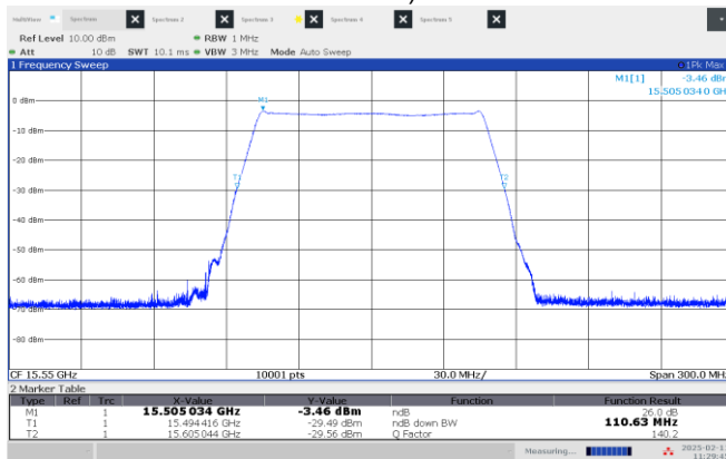
Figure 8.2-15: 26 dB OBW Middle channel: 15.55 GHz, shortest pulse (100 MHz BW)
