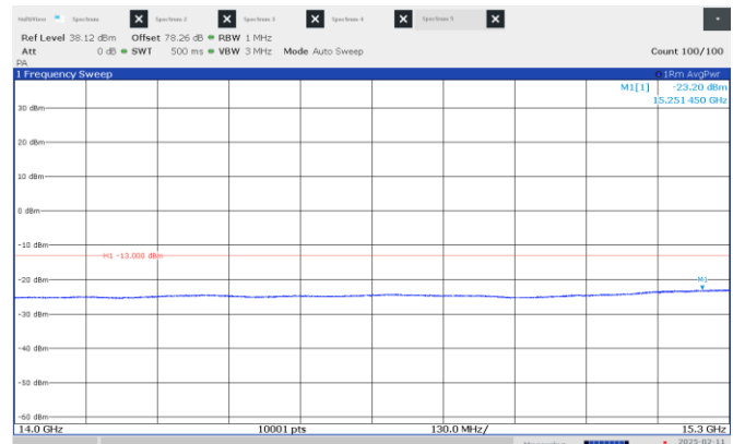
Figure 8.4-34: Emission mask, beyond \pm 250\% of BW (low frequency range), Low channel: 15.50 GHz, shortest pulse. (50 MHz BW)
