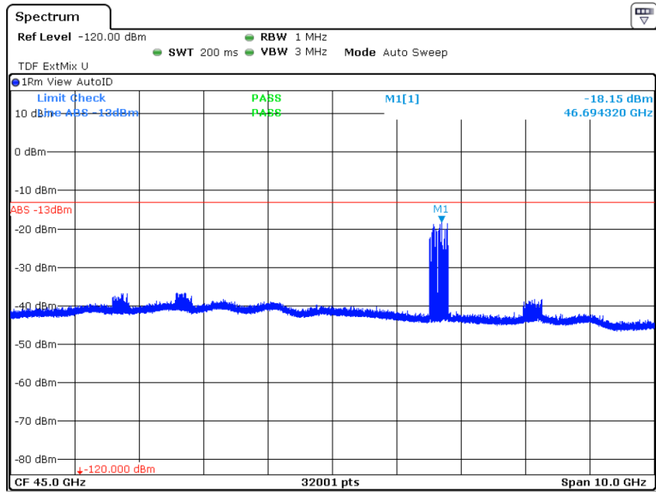
Figure 8.5-1: Radiated emissions spectral plot (40 GHz - 50 GHz) Horizontal
