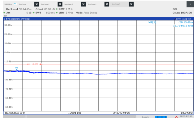
Figure 8.4-12: Emission mask, beyond \pm 250\% of BW (high frequency range), Low channel: 15.50 GHz, longest pulse. (50 MHz BW)
