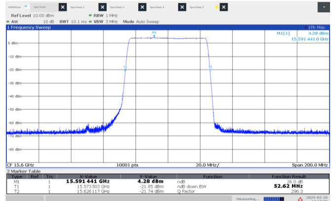
Figure 8.2-6: 26 dB OBW High channel: 15.60 GHz, longest pulse (50 MHz BW)
