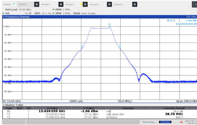
Figure 8.2-11: 26 dB OBW High channel: 15.65 GHz, shortest pulse (25 MHz BW)
