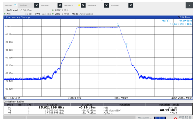
Figure 8.2-14: 26 dB OBW High channel: 15.60 GHz, shortest pulse (50 MHz BW)
