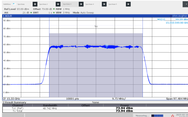
Figure 8.3-5: EIRP Power, Middle channel: 15.55 GHz, longest pulse (50 MHz BW)
