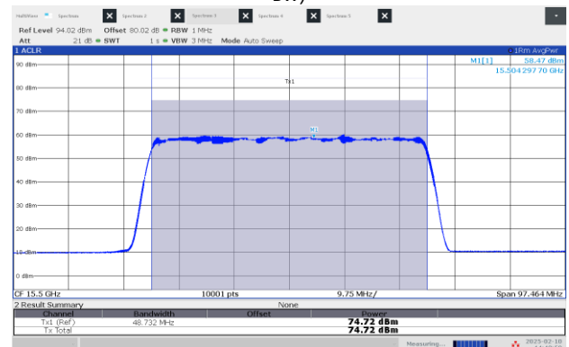
Figure 8.3-4: EIRP Power, Low channel: 15.50 GHz, longest pulse (50 MHz BW)
