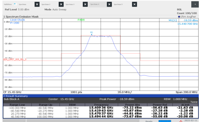
Figure 8.4-26: Emission mask, Low channel: 15.45 GHz, shortest pulse. (25 MHz BW)
