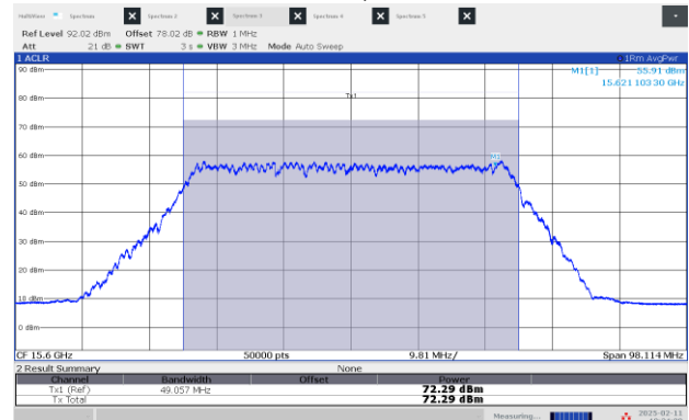
Figure 8.3-14: EIRP Power, High channel: 15.60 GHz, shortest pulse (50 MHz BW)
