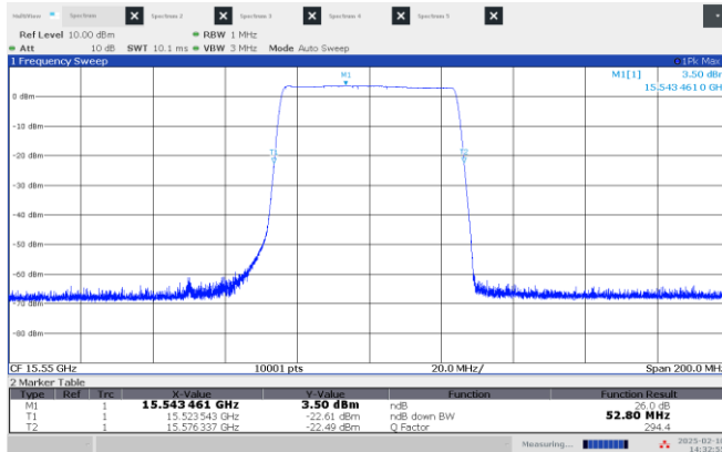
Figure 8.2-5: 26 dB OBW Middle channel: 15.55 GHz, longest pulse (50 MHz BW)
