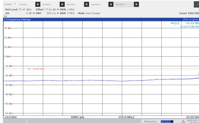
Figure 8.4-31: Emission mask, beyond \pm 250\% of BW (low frequency range), High channel: 15.65 GHz, shortest pulse. (25 MHz BW)
