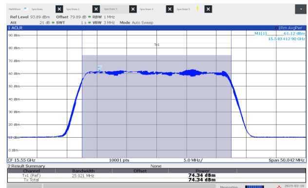
Figure 8.3-2: EIRP Power, Middle channel: 15.55 GHz, longest pulse (25 MHz BW)
