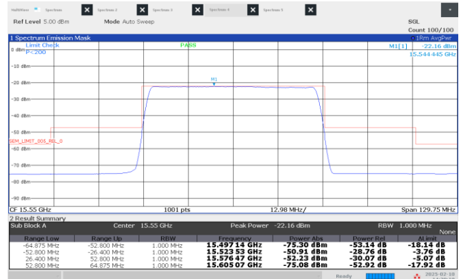
Figure 8.4-14: Emission mask, Middle channel: 15.55 GHz, longest pulse. (50 MHz BW)
