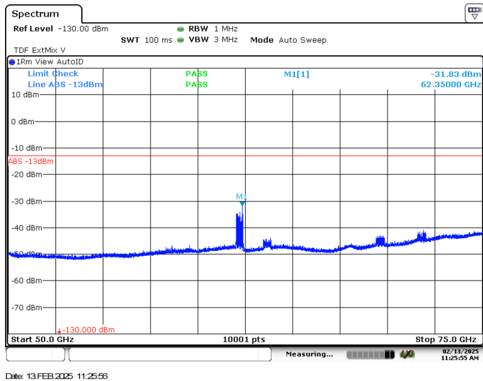
Figure 8.5-4: Radiated emissions spectra I plot (50 GHz - 75 GHz) Vertical
