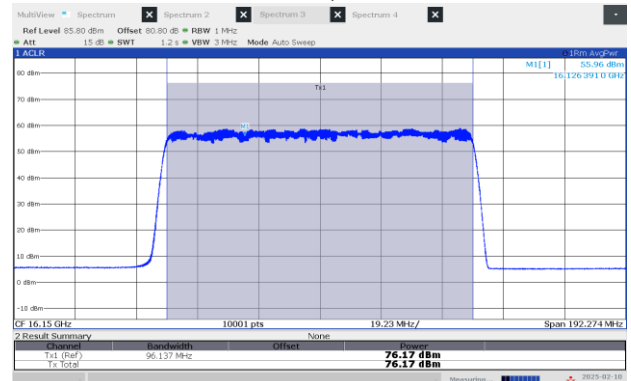
Figure 8.3-8: EIRP Power, Middle channel: 16.15 GHz, longest pulse (100 MHz BW)
