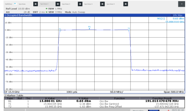
Figure 8.1-10: 99% OBW Low channel: 15.90 GHz, longest pulse (200 MHz BW)
