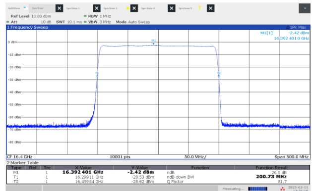
Figure 8.2-24: 26 dB OBW High channel: 16.40 GHz, shortest pulse (200 MHz BW)
