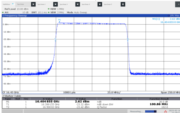
Figure 8.2-9: 26 dB OBW High channel: 16.45 GHz, longest pulse (100 MHz BW)
