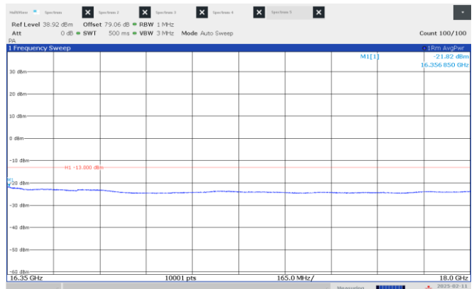
Figure 8.4-42: Emission mask, beyond \pm 250\% of BW (high frequency range), Middle channel: 16.15 GHz, shortest pulse. (25 MHz BW)
