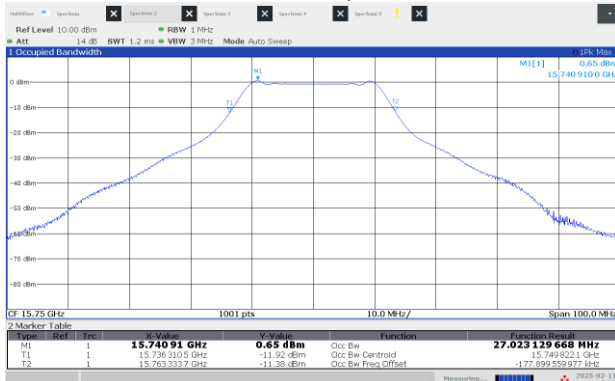
Figure 8.1-13: 99% OBW Low channel: 15.75 GHz, shortest pulse (25 MHz BW)
