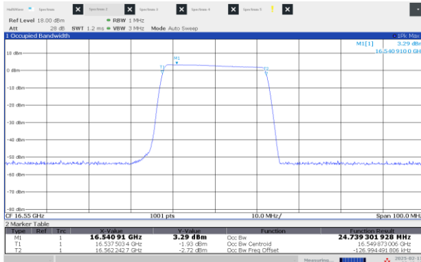
Figure 8.1-3: 99% OBW High channel: 16.55 GHz, longest pulse (25 MHz BW)
