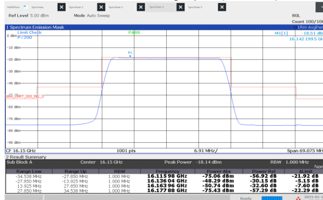
Figure 8.4-5: Emission mask, Middle channel: 16.15 GHz, longest pulse. (25 MHz BW)
