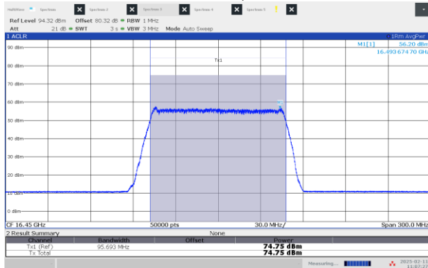
Figure 8.3-21: EIRP Power, High channel: 16.45 GHz, shortest pulse (100 MHz BW)
