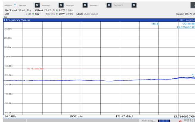
Figure 8.4-1: Emission mask, beyond \pm 250\% of BW (low frequency range), Low channel: 15.75 GHz, longest pulse. (25 MHz BW)
