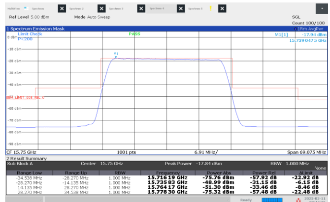
Figure 8.4-2: Emission mask, Low channel: 15.75 GHz, longest pulse. (25 MHz BW)
