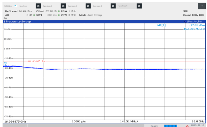
Figure 8.4-18: Emission mask, beyond \pm 250\% of BW (high frequency range), High channel: 16.50 GHz, longest pulse. (50 MHz BW)
