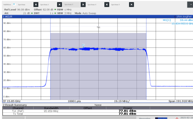
Figure 8.3-7: EIRP Power, Low channel: 15.85 GHz, longest pulse (100 MHz BW)
