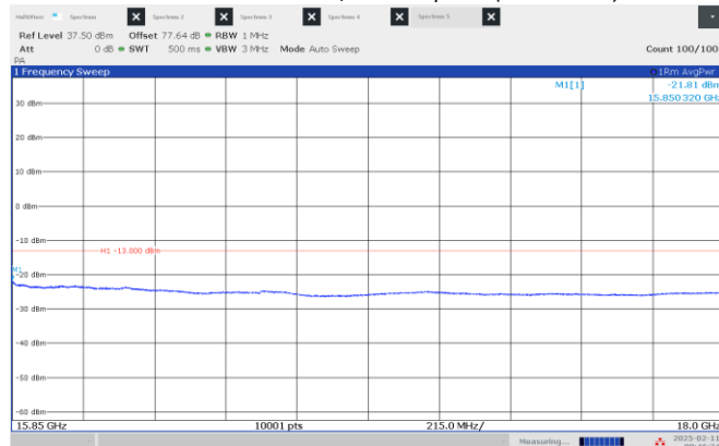
Figure 8.4-39: Emission mask, beyond \pm 250\% of BW (high frequency range), Low channel: 15.75 GHz, shortest pulse. (25 MHz BW)
