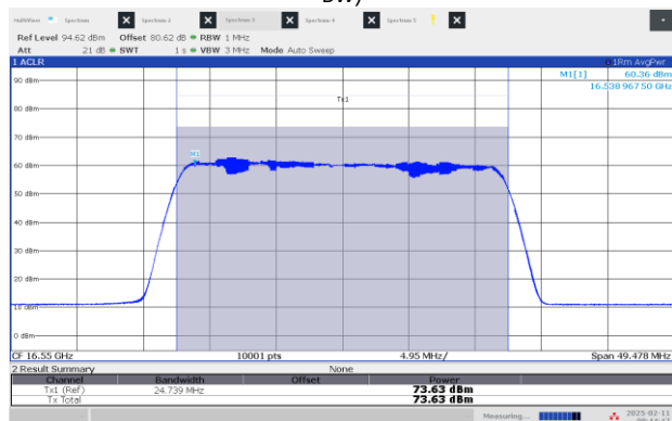
Figure 8.3-3: EIRP Power, High channel: 16.55 GHz, longest pulse (25 MHz BW)
