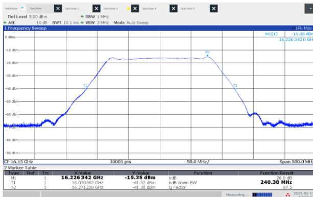
Figure 8.2-23: 26 dB OBW Middle channel: 16.15 GHz, shortest pulse (200 MHz BW)
