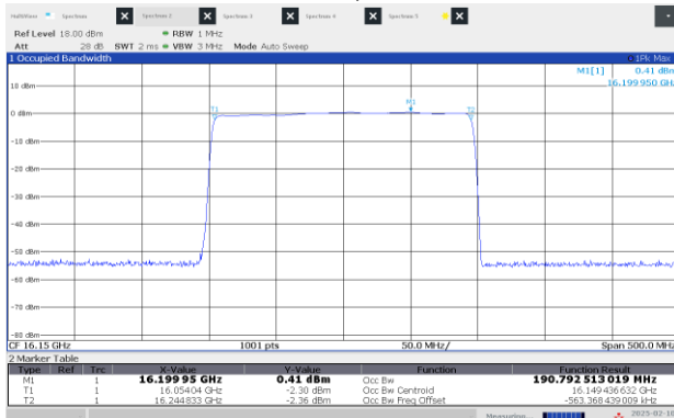
Figure 8.1-11: 99% OBW Middle channel: 16.15 GHz, longest pulse (200 MHz BW)
