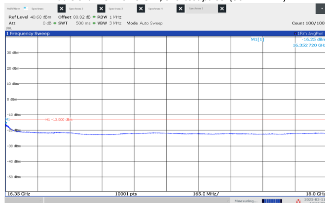
Figure 8.4-51: Emission mask, beyond \pm 250\% of BW (high frequency range), Middle channel: 16.15 GHz, shortest pulse. (50 MHz BW)
