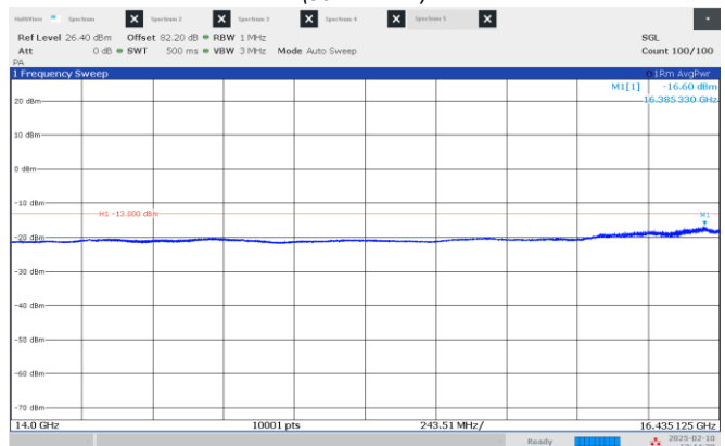
Figure 8.4-16: Emission mask, beyond \pm 250\% of BW (low frequency range), High channel: 16.50 GHz, longest pulse. (50 MHz BW)
