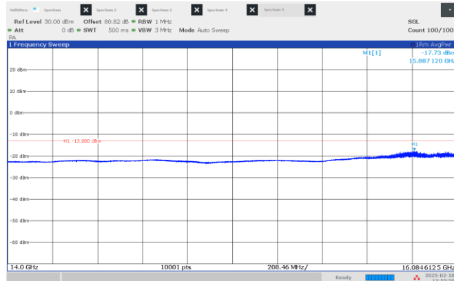
Figure 8.4-13: Emission mask, beyond \pm 250\% of BW (low frequency range), Middle channel: 16.15 GHz, longest pulse. (50 MHz BW)
