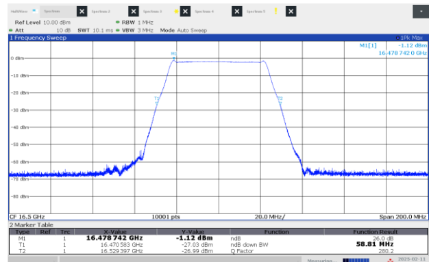
Figure 8.2-18: 26 dB OBW High channel: 16.50 GHz, shortest pulse (50 MHz BW)
