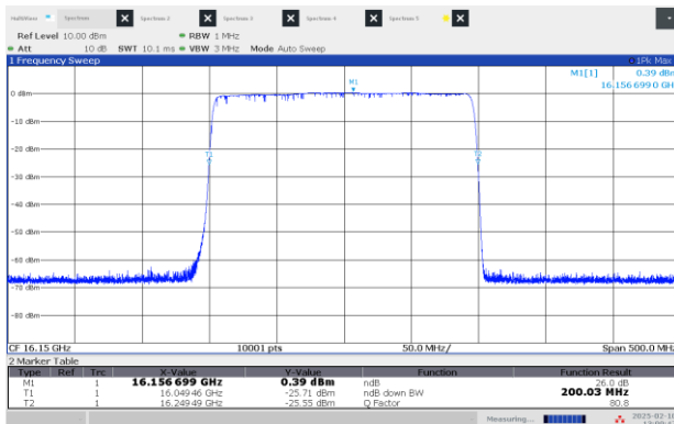
Figure 8.2-11: 26 dB OBW Middle channel: 16.15 GHz, longest pulse (200 MHz BW)
