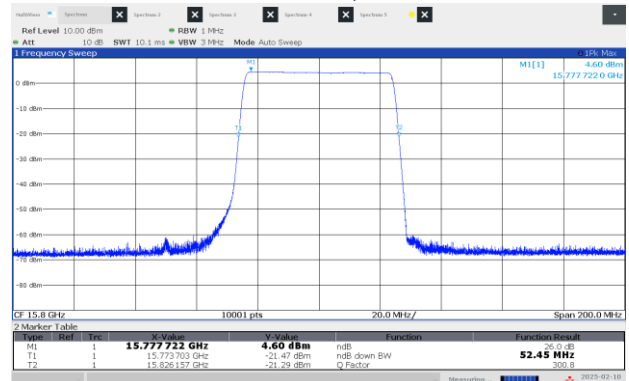
Figure 8.2-4: 26 dB OBW Low channel: 15.80 GHz, longest pulse (50 MHz BW)
