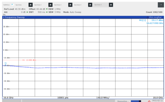
Figure 8.4-54: Emission mask, beyond \pm 250\% of BW (high frequency range), High channel: 16.50 GHz, shortest pulse. (50 MHz BW)
