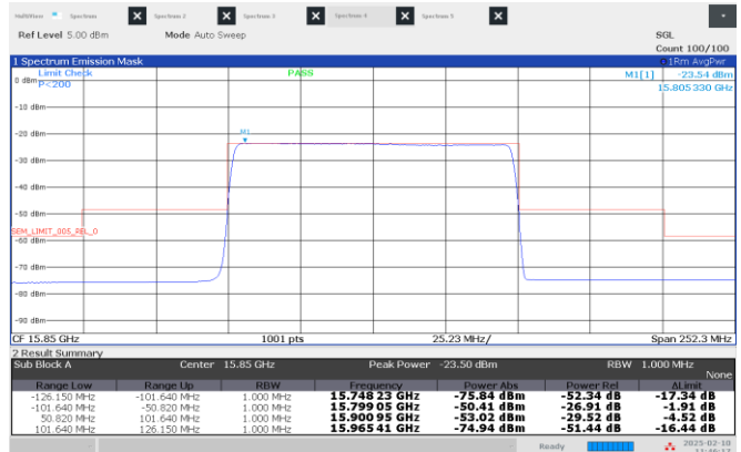
Figure 8.4-20: Emission mask, Low channel: 15.85 GHz, longest pulse. (100 MHz BW)
