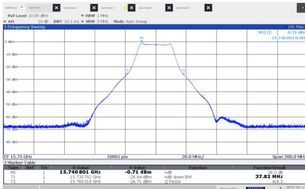
Figure 8.2-13: 26 dB OBW Low channel: 15.75 GHz, shortest pulse (25 MHz BW)
