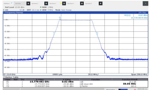
Figure 8.2-16: 26 dB OBW Low channel: 15.80 GHz, shortest pulse (50 MHz BW)
