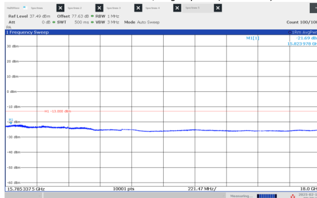
Figure 8.4-3: Emission mask, beyond \pm 250\% of BW (high frequency range), Low channel: 15.75 GHz, longest pulse. (25 MHz BW)
