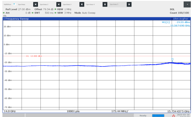
Figure 8.4-10: Emission mask, beyond \pm 250\% of BW (low frequency range), Low channel: 15.80 GHz, longest pulse. (50 MHz BW)
