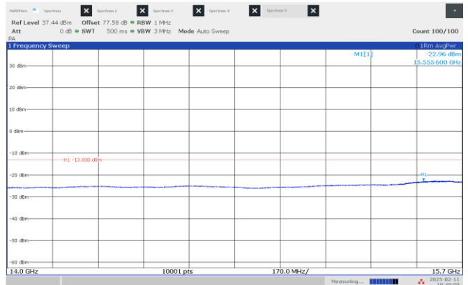
Figure 8.4-46: Emission mask, beyond \pm 250\% of BW (low frequency range), Low channel: 15.80 GHz, shortest pulse. (50 MHz BW)
