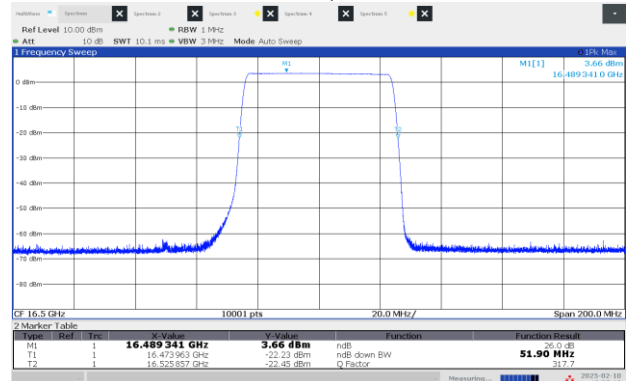
Figure 8.2-6: 26 dB OBW High channel: 16.50 GHz, longest pulse (50 MHz BW)
