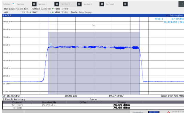
Figure 8.3-9: EIRP Power, High channel: 16.45 GHz, longest pulse (100 MHz BW)
