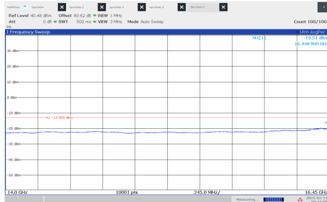
Figure 8.4-43: Emission mask, beyond \pm 250\% of BW (low frequency range), High channel: 16.55 GHz, shortest pulse. (25 MHz BW)
