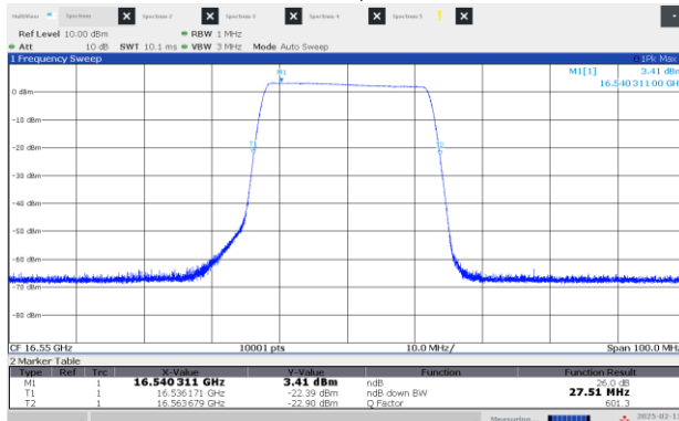
Figure 8.2-3: 26 dB OBW High channel: 16.55 GHz, longest pulse (25 MHz BW)
