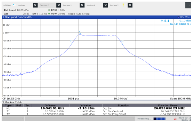
Figure 8.1-15: 99% OBW High channel: 16.55 GHz, shortest pulse (25 MHz BW)
