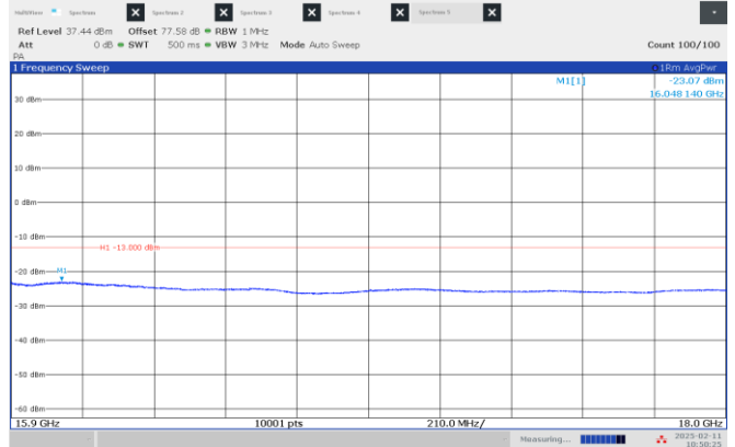
Figure 8.4-48: Emission mask, beyond \pm 250\% of BW (high frequency range), Low channel: 15.80 GHz, shortest pulse. (50 MHz BW)
