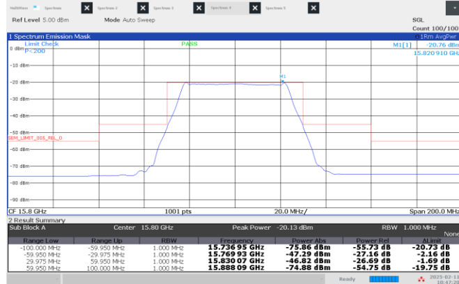
Figure 8.4-47: Emission mask, Low channel: 15.80 GHz, shortest pulse. (50 MHz BW)
