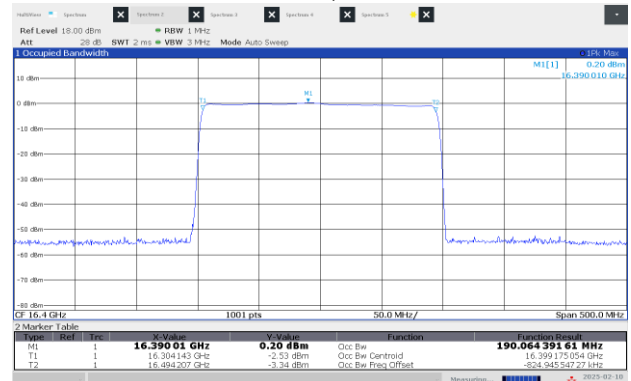
Figure 8.1-12: 99% OBW High channel: 16.40 GHz, longest pulse (200 MHz BW)
