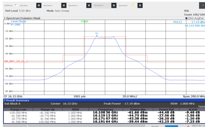
Figure 8.4-41: Emission mask, Middle channel: 16.15 GHz, shortest pulse. (25 MHz BW)
