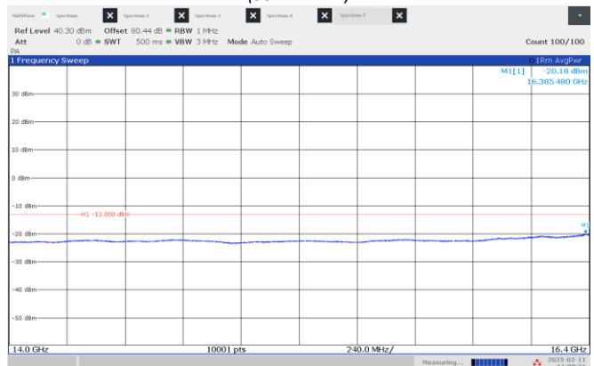
Figure 8.4-52: Emission mask, beyond \pm 250\% of BW (low frequency range), High channel: 16.50 GHz, shortest pulse. (50 MHz BW)
