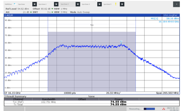
Figure 8.3-20: EIRP Power, Middle channel: 16.15 GHz, shortest pulse (100 MHz BW)
