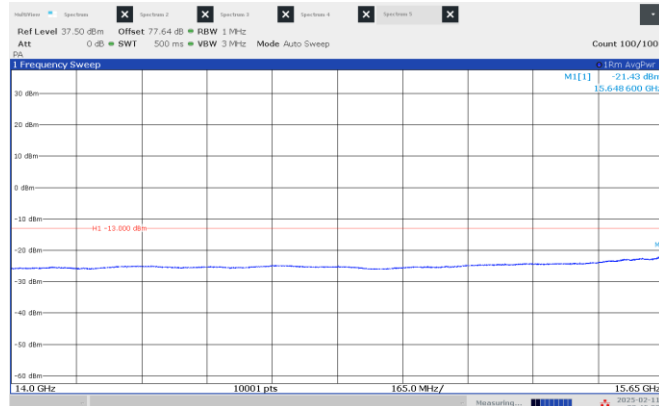
Figure 8.4-37: Emission mask, beyond \pm 250\% of BW (low frequency range), Low channel: 15.75 GHz, shortest pulse. (25 MHz BW)
