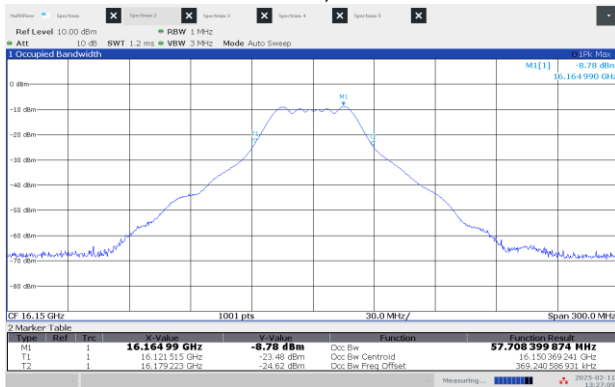
Figure 8.1-17: 99% OBW Middle channel: 16.15 GHz, shortest pulse (50 MHz BW)
