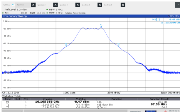
Figure 8.2-17: 26 dB OBW Middle channel: 16.15 GHz, shortest pulse (50 MHz BW)
