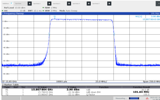
Figure 8.2-7: 26 dB OBW Low channel: 15.85 GHz, longest pulse (100 MHz BW)
