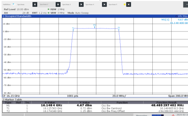
Figure 8.1-5: 99% OBW Middle channel: 16.15 GHz, longest pulse (50 MHz BW)
