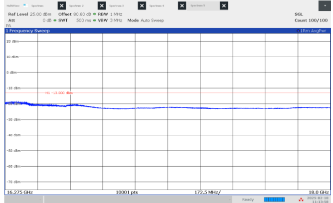
Figure 8.4-24: Emission mask, beyond \pm 250\% of BW (high frequency range), Middle channel: 16.15 GHz, longest pulse. (100 MHz BW)
