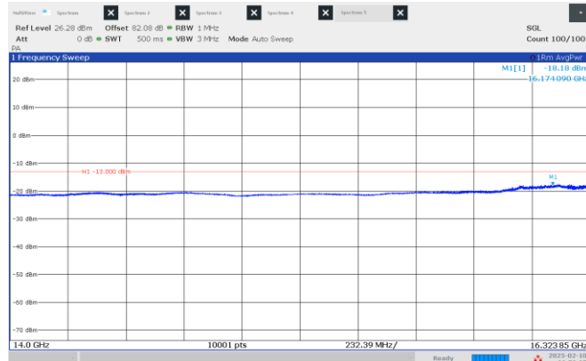
Figure 8.4-25: Emission mask, beyond \pm 250\% of BW (low frequency range), High channel: 16.45 GHz, longest pulse. (100 MHz BW)
