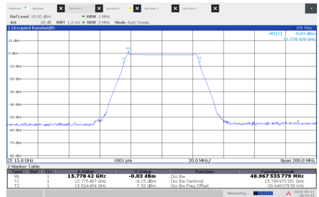
Figure 8.1-16: 99% OBW Low channel: 15.80 GHz, shortest pulse (50 MHz BW)
