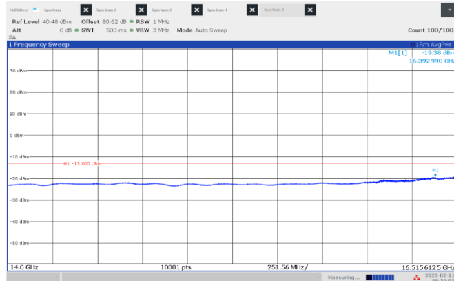
Figure 8.4-7: Emission mask, beyond \pm 250\% of BW (low frequency range), High channel: 16.55 GHz, longest pulse. (25 MHz BW)
