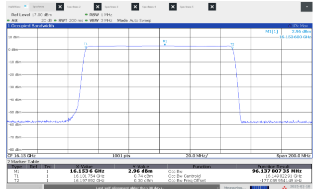
Figure 8.1-8: 99% OBW Middle channel: 16.15 GHz, longest pulse (100 MHz BW)
