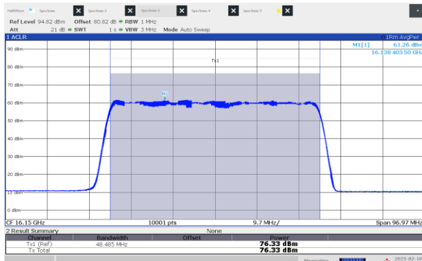
Figure 8.3-5: EIRP Power, Middle channel: 16.15 GHz, longest pulse (50 MHz BW)
