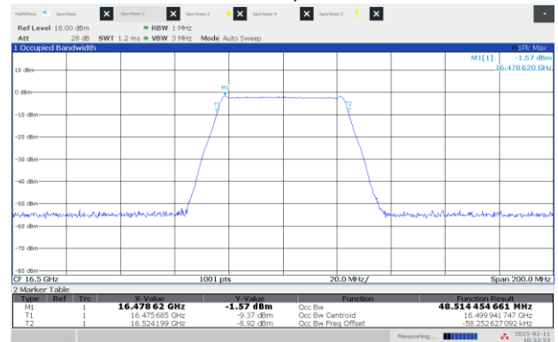
Figure 8.1-18: 99% OBW High channel: 16.50 GHz, shortest pulse (50 MHz BW)
