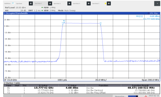
Figure 8.1-4: 99% OBW Low channel: 15.80 GHz, longest pulse (50 MHz BW)
