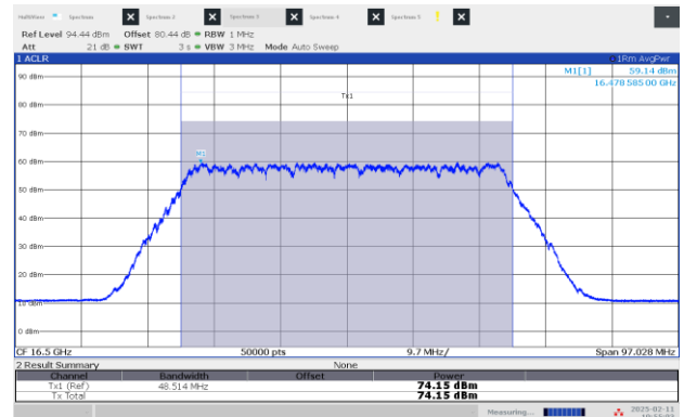
Figure 8.3-18: EIRP Power, High channel: 16.50 GHz, shortest pulse (50 MHz BW)
