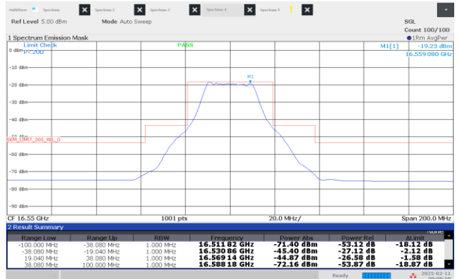
Figure 8.4-44: Emission mask, High channel: 16.55 GHz, shortest pulse. (25 MHz BW)
