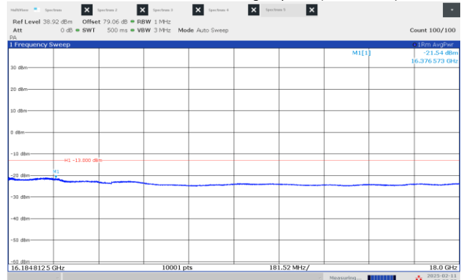
Figure 8.4-6: Emission mask, beyond \pm 250\% of BW (high frequency range), Middle channel: 16.15 GHz, longest pulse. (25 MHz BW)
