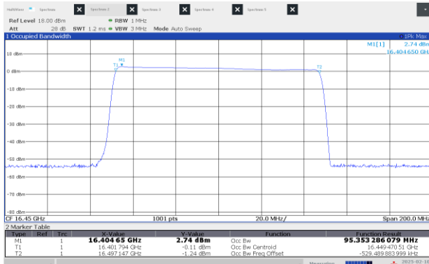
Figure 8.1-9: 99% OBW High channel: 16.45 GHz, longest pulse (100 MHz BW)
