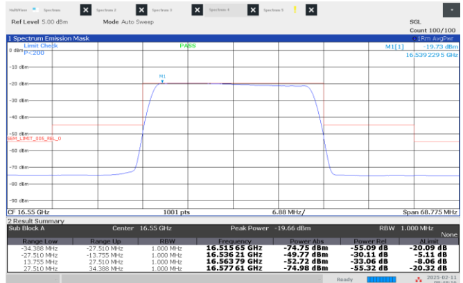
Figure 8.4-8: Emission mask, High channel: 16.55 GHz, longest pulse. (25 MHz BW)
