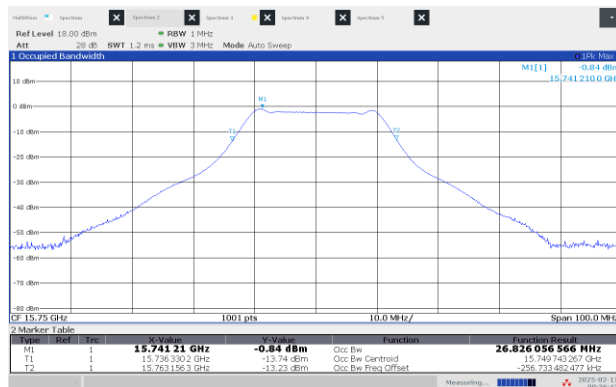
Figure 8.1-1: 99% OBW Low channel: 15.75 GHz, longest pulse (25 MHz BW)
