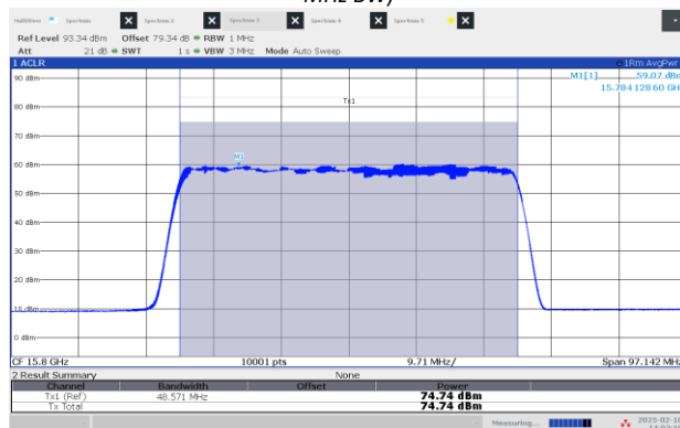
Figure 8.3-4: EIRP Power, Low channel: 15.80 GHz, longest pulse (50 MHz BW)
