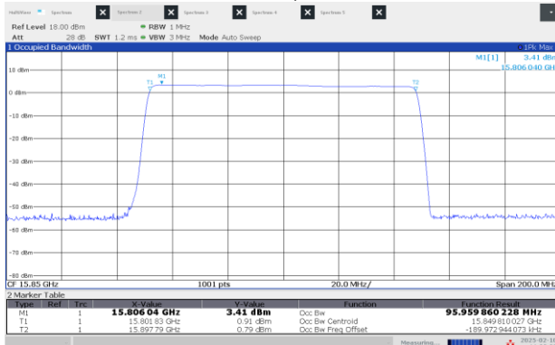
Figure 8.1-7: 99% OBW Low channel: 15.85 GHz, longest pulse (100 MHz BW)
