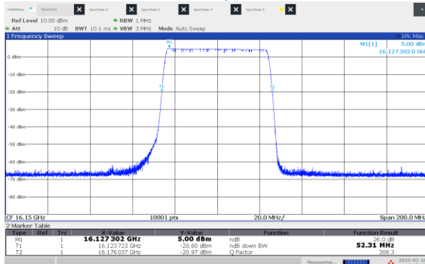
Figure 8.2-5: 26 dB OBW Middle channel: 16.15 GHz, longest pulse (50 MHz BW)
