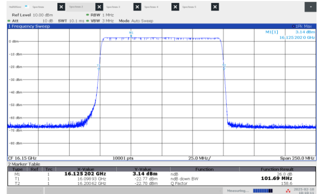
Figure 8.2-8: 26 dB OBW Middle channel: 16.15 GHz, longest pulse (100 MHz BW)
