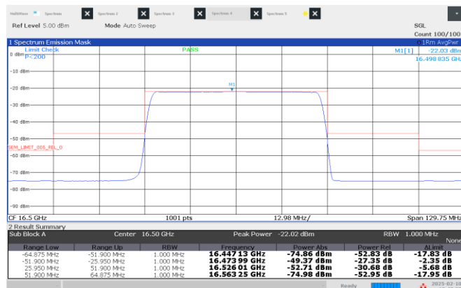
Figure 8.4-17: Emission mask, High channel: 16.50 GHz, longest pulse. (50 MHz BW)
