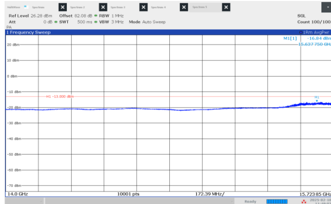
Figure 8.4-19: Emission mask, beyond \pm 250\% of BW (low frequency range), Low channel: 15.85 GHz, longest pulse. (100 MHz BW)
