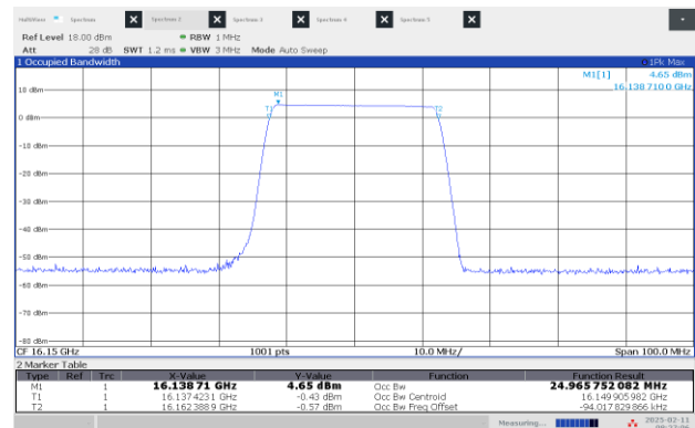
Figure 8.1-2: 99% OBW Middle channel: 16.15 GHz, longest pulse (25 MHz BW)
