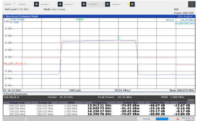
Figure 8.4-32: Emission mask, Middle channel: 16.15 GHz, longest pulse. (200 MHz BW)
