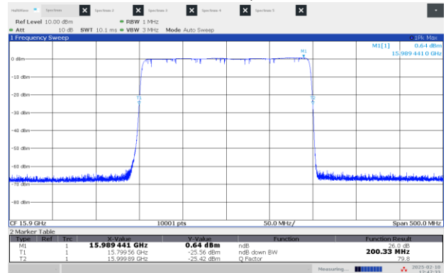
Figure 8.2-10: 26 dB OBW Low channel: 15.90 GHz, longest pulse (200 MHz BW)
