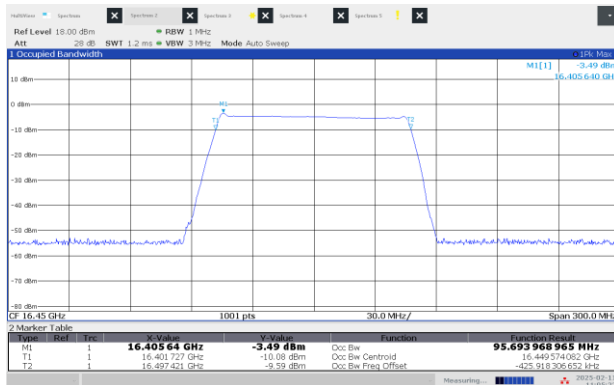
Figure 8.1-21: 99% OBW High channel: 16.45 GHz, shortest pulse (100 MHz BW)
