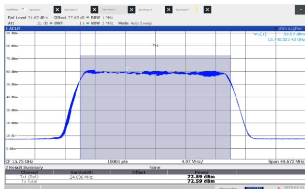
Figure 8.3-1: EIRP Power, Low channel: 15.75 GHz, longest pulse (25 MHz BW)
