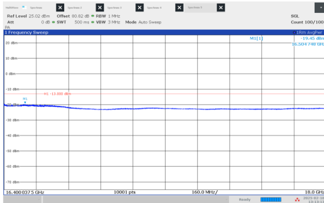
Figure 8.4-33: Emission mask, beyond \pm 250\% of BW (high frequency range), Middle channel: 16.15 GHz, longest pulse. (200 MHz BW)
