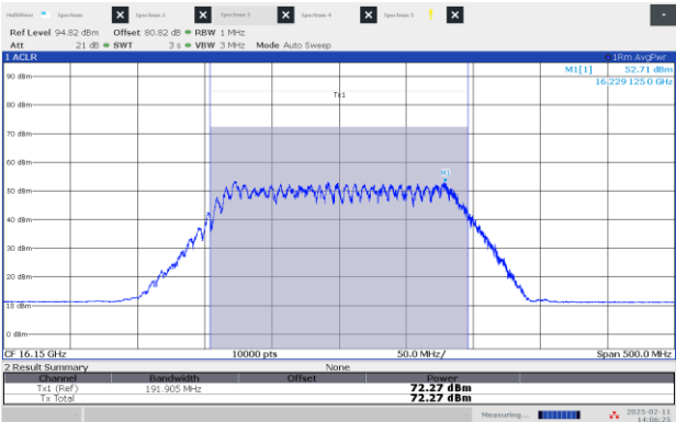
Figure 8.3-23: EIRP Power, Middle channel: 16.15 GHz, shortest pulse (200 MHz BW)
