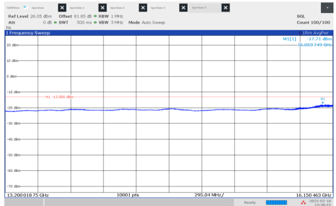
Figure 8.4-34: Emission mask, beyond \pm 250\% of BW (low frequency range), High channel: 16.40 GHz, longest pulse. (200 MHz BW)
