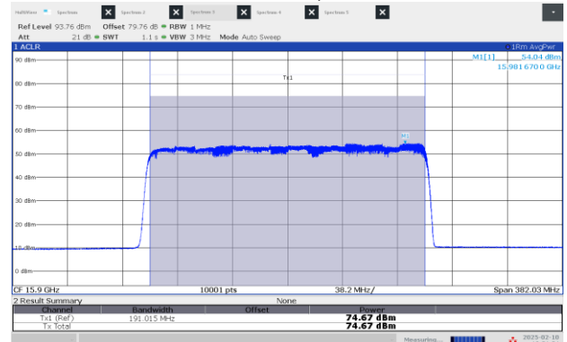
Figure 8.3-10: EIRP Power, Low channel: 15.90 GHz, longest pulse (200 MHz BW)
