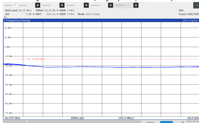
Figure 8.4-27: Emission mask, beyond \pm 250\% of BW (high frequency range), High channel: 16.45 GHz, longest pulse. (100 MHz BW)
