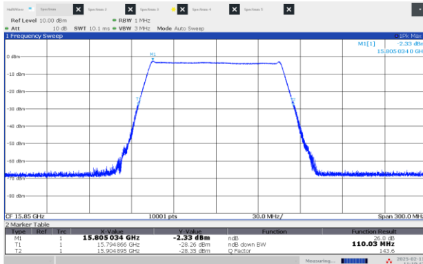
Figure 8.2-19: 26 dB OBW Low channel: 15.85 GHz, shortest pulse (100 MHz BW)
