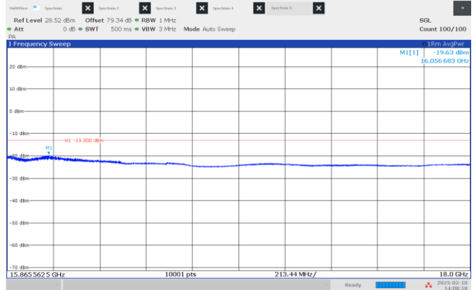
Figure 8.4-12: Emission mask, beyond \pm 250\% of BW (high frequency range), Low channel: 15.80 GHz, longest pulse. (50 MHz BW)
