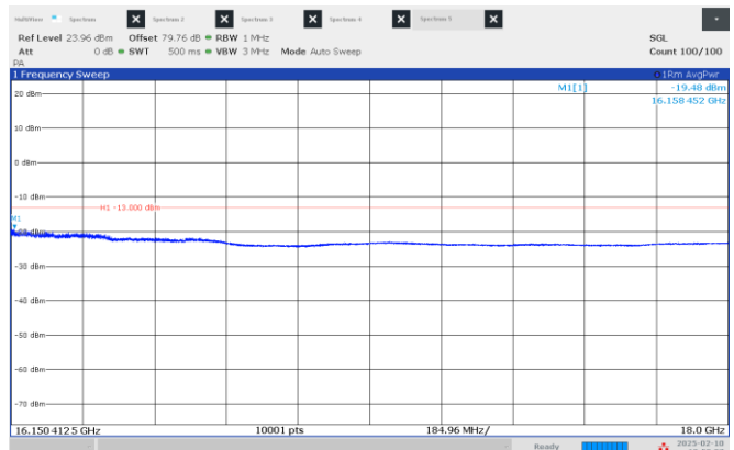
Figure 8.4-30: Emission mask, beyond \pm 250\% of BW (high frequency range), Low channel: 15.90 GHz, longest pulse. (200 MHz BW)
