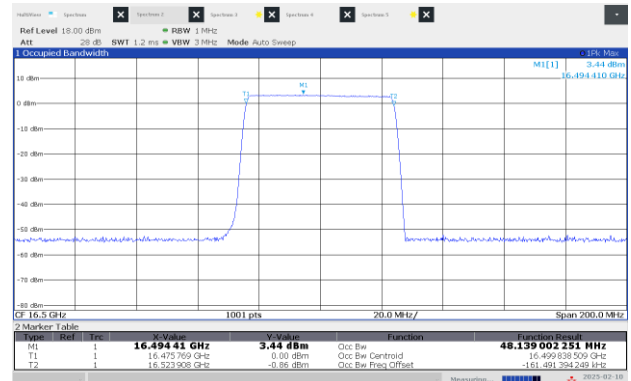
Figure 8.1-6: 99% OBW High channel: 16.50 GHz, longest pulse (50 MHz BW)
