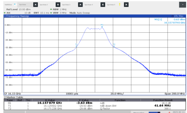
Figure 8.2-14: 26 dB OBW Middle channel: 16.15 GHz, shortest pulse (25 MHz BW)
