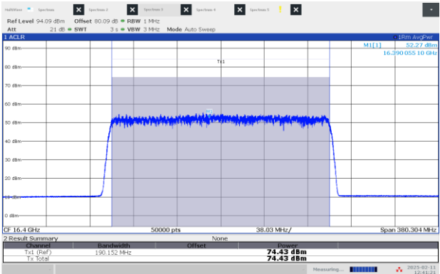
Figure 8.3-24: EIRP Power, High channel: 16.40 GHz, shortest pulse (200 MHz BW)
