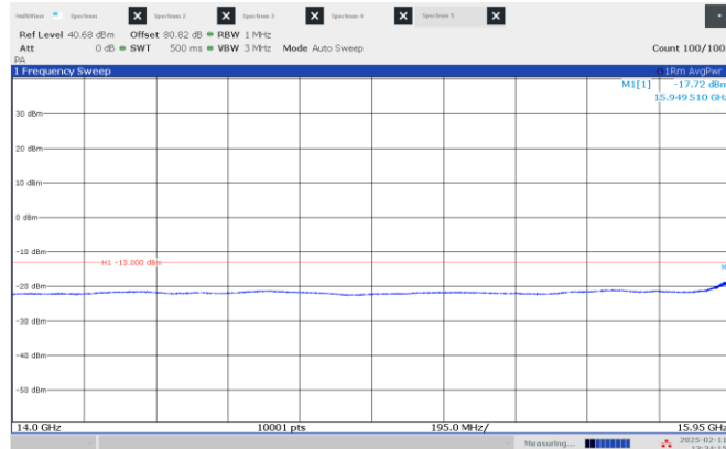
Figure 8.4-49: Emission mask, beyond \pm 250\% of BW (low frequency range), Middle channel: 16.15 GHz, shortest pulse. (50 MHz BW)
