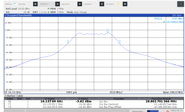
Figure 8.1-14: 99% OBW Middle channel: 16.15 GHz, shortest pulse (25 MHz BW)
