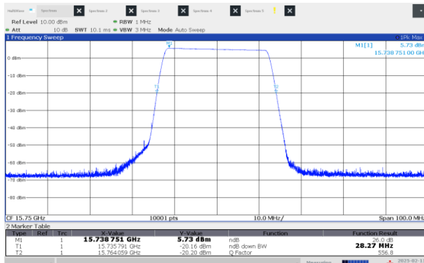
Figure 8.2-1: 26 dB OBW Low channel: 15.75 GHz, longest pulse (25 MHz BW)
