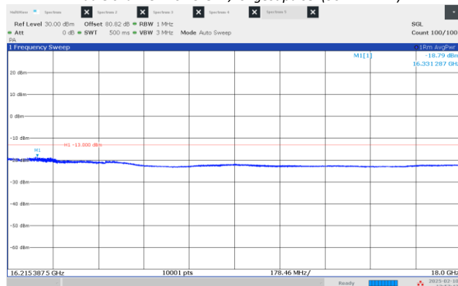
Figure 8.4-15: Emission mask, beyond \pm 250\% of BW (high frequency range), Middle channel: 16.15 GHz, longest pulse. (50 MHz BW)
