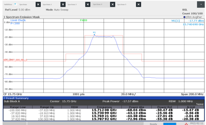
Figure 8.4-38: Emission mask, Low channel: 15.75 GHz, shortest pulse. (25 MHz BW)
