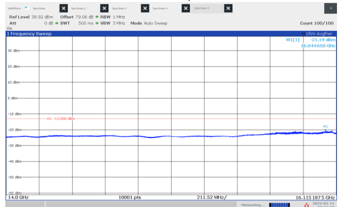
Figure 8.4-4: Emission mask, beyond \pm 250\% of BW (low frequency range), Middle channel: 16.15 GHz, longest pulse. (25 MHz BW)
