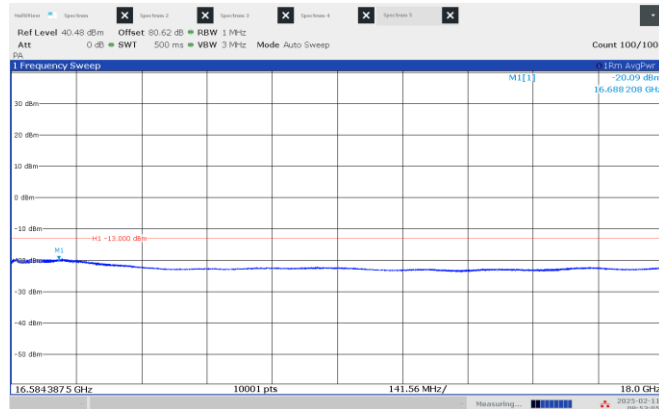
Figure 8.4-9: Emission mask, beyond \pm 250\% of BW (high frequency range), High channel: 16.55 GHz, longest pulse. (25 MHz BW)
