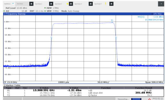
Figure 8.2-22: 26 dB OBW Low channel: 15.90 GHz, shortest pulse (200 MHz BW)
