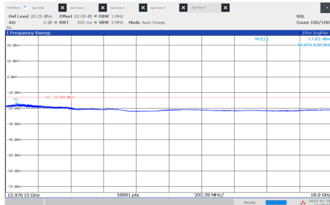
Figure 8.4-21: Emission mask, beyond \pm 250\% of BW (high frequency range), Low channel: 15.85 GHz, longest pulse. (100 MHz BW)
