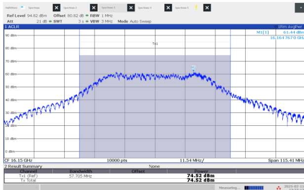
Figure 8.3-17: EIRP Power, Middle channel: 16.15 GHz, shortest pulse (50 MHz BW)
