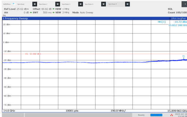
Figure 8.4-31: Emission mask, beyond \pm 250\% of BW (low frequency range), Middle channel: 16.15 GHz, longest pulse. (200 MHz BW)
