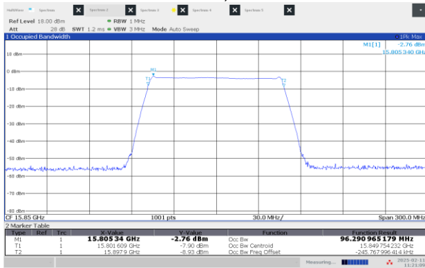
Figure 8.1-19: 99% OBW Low channel: 15.85 GHz, shortest pulse (100 MHz BW)
