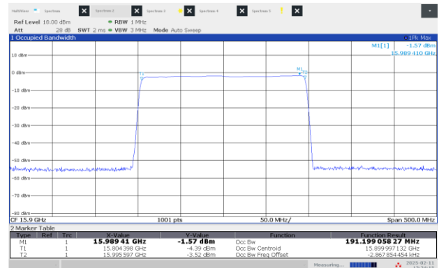
Figure 8.1-22: 99% OBW Low channel: 15.90 GHz, shortest pulse (200 MHz BW)
