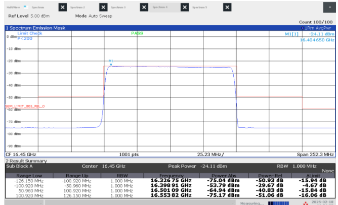
Figure 8.4-26: Emission mask, High channel: 16.45 GHz, longest pulse. (100 MHz BW)
