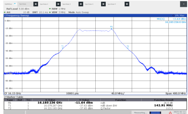
Figure 8.2-20: 26 dB OBW Middle channel: 16.15 GHz, shortest pulse (100 MHz BW)
