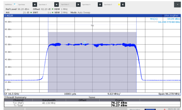
Figure 8.3-6: EIRP Power, High channel: 16.50 GHz, longest pulse (50 MHz BW)
