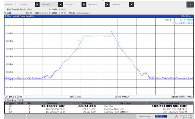
Figure 8.1-20: 99% OBW Middle channel: 16.15 GHz, shortest pulse (100 MHz BW)
