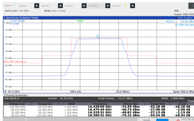
Figure 8.4-53: Emission mask, High channel: 16.50 GHz, shortest pulse. (50 MHz BW)
