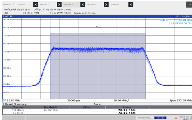
Figure 8.3-19: EIRP Power, Low channel: 15.85 GHz, shortest pulse (100 MHz BW)
