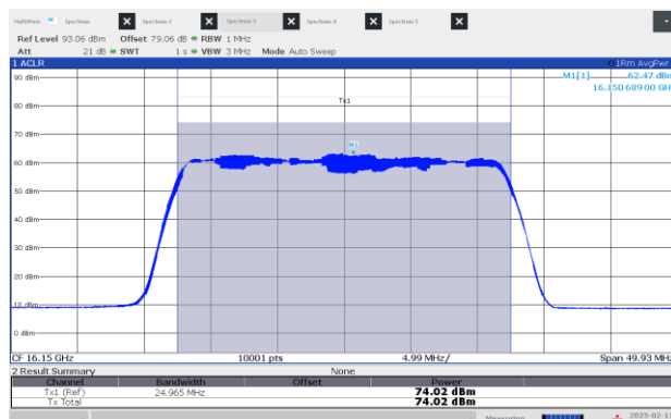
Figure 8.3-2: EIRP Power, Middle channel: 16.15 GHz, longest pulse (25 MHz BW)
