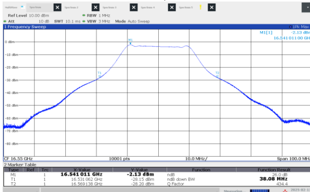
Figure 8.2-15: 26 dB OBW High channel: 16.55 GHz, shortest pulse (25 MHz BW)
