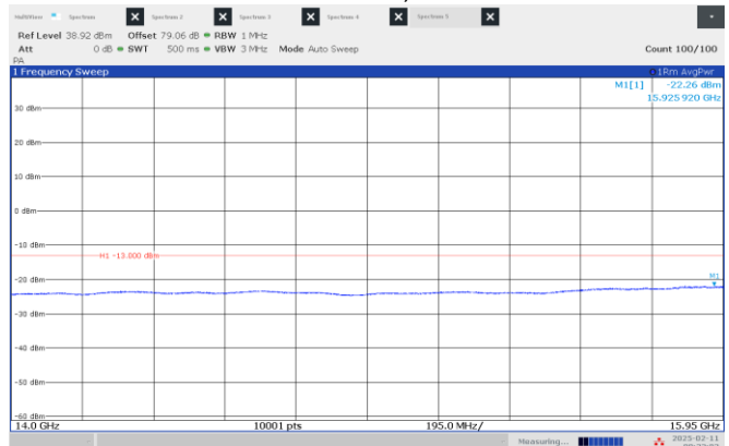
Figure 8.4-40: Emission mask, beyond \pm 250\% of BW (low frequency range), Middle channel: 16.15 GHz, shortest pulse. (25 MHz BW)
