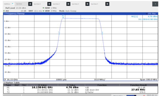
Figure 8.2-2: 26 dB OBW Middle channel: 16.15 GHz, longest pulse (25 MHz BW)
