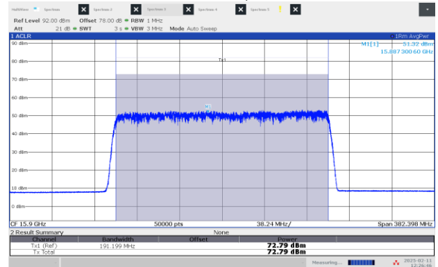
Figure 8.3-22: EIRP Power, Low channel: 15.90 GHz, shortest pulse (200 MHz BW)
