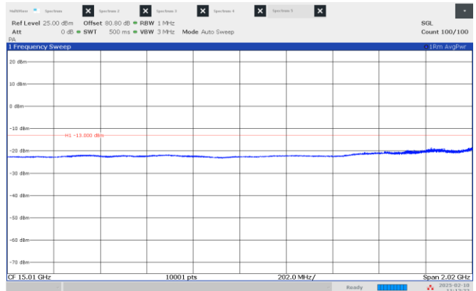
Figure 8.4-22: Emission mask, beyond \pm 250\% of BW (low frequency range), Middle channel: 16.15 GHz, longest pulse. (100 MHz BW)
