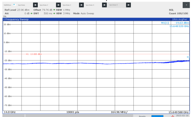
Figure 8.4-28: Emission mask, beyond \pm 250\% of BW (low frequency range), Low channel: 15.90 GHz, longest pulse. (200 MHz BW)
