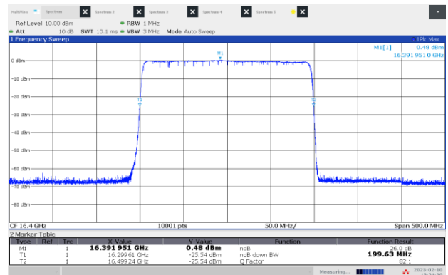
Figure 8.2-12: 26 dB OBW High channel: 16.40 GHz, longest pulse (200 MHz BW)
