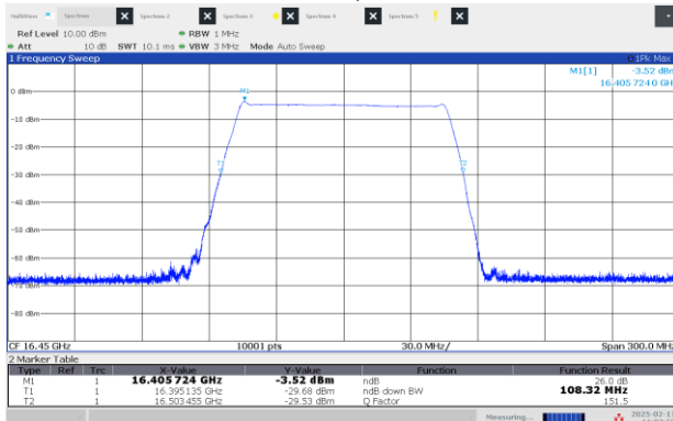
Figure 8.2-21: 26 dB OBW High channel: 16.45 GHz, shortest pulse (100 MHz BW)
