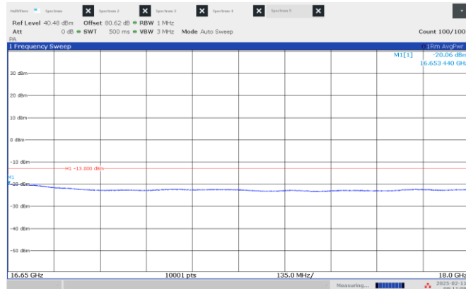
Figure 8.4-45: Emission mask, beyond \pm 250\% of BW (high frequency range), High channel: 16.55 GHz, shortest pulse. (25 MHz BW)
