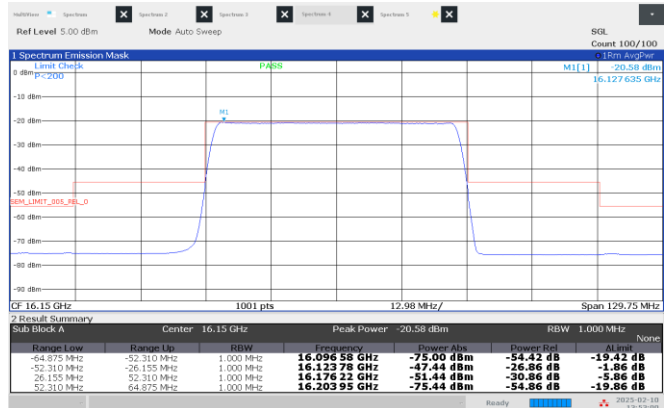
Figure 8.4-14: Emission mask, Middle channel: 16.15 GHz, longest pulse. (50 MHz BW)
