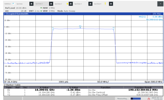
Figure 8.1-24: 99% OBW High channel: 16.40 GHz, shortest pulse (200 MHz BW)
