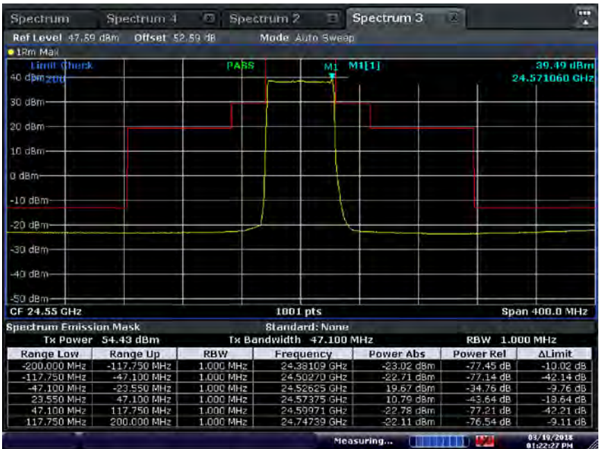
Figure 8.3-5: FCC Part 87 Emission mask (MC, 24.55 GHz)
