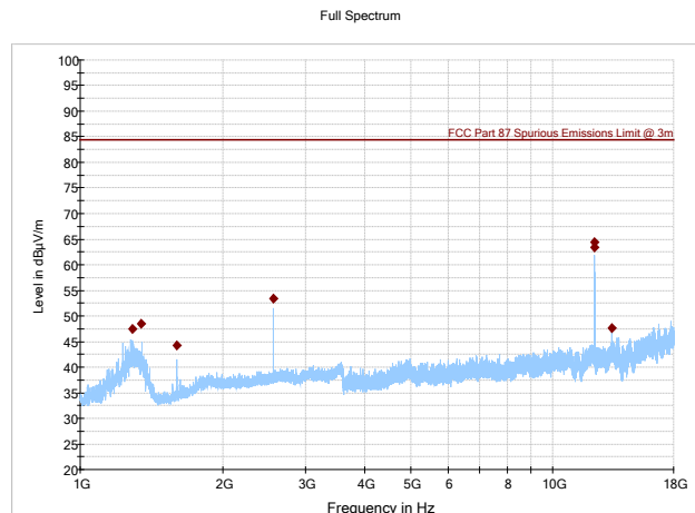
Figure 8.6.2: Radiated spurious emissions, 1-18 GHz Low Channel
