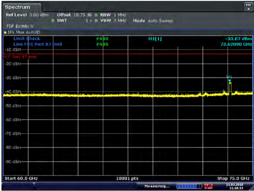
Figure 8.5.15: 60-75 GHz (High channel, 24.61 GHz)
