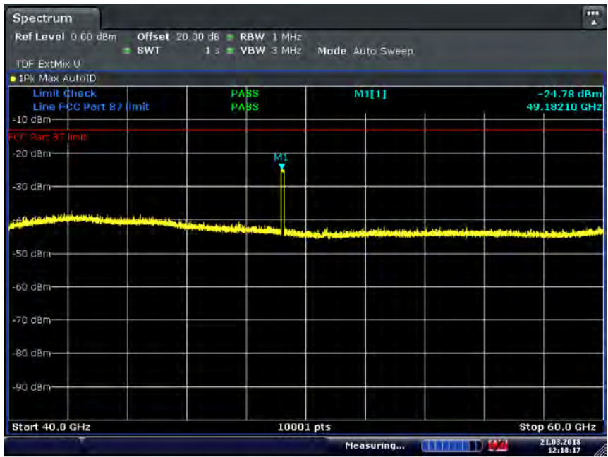
Figure 8.5.13: 40-60 GHz (High channel, 24.61 GHz)
