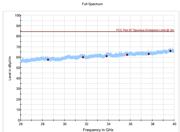
Figure 8.6.8: Radiated spurious emissions, 26-40 GHz Mid Channel
