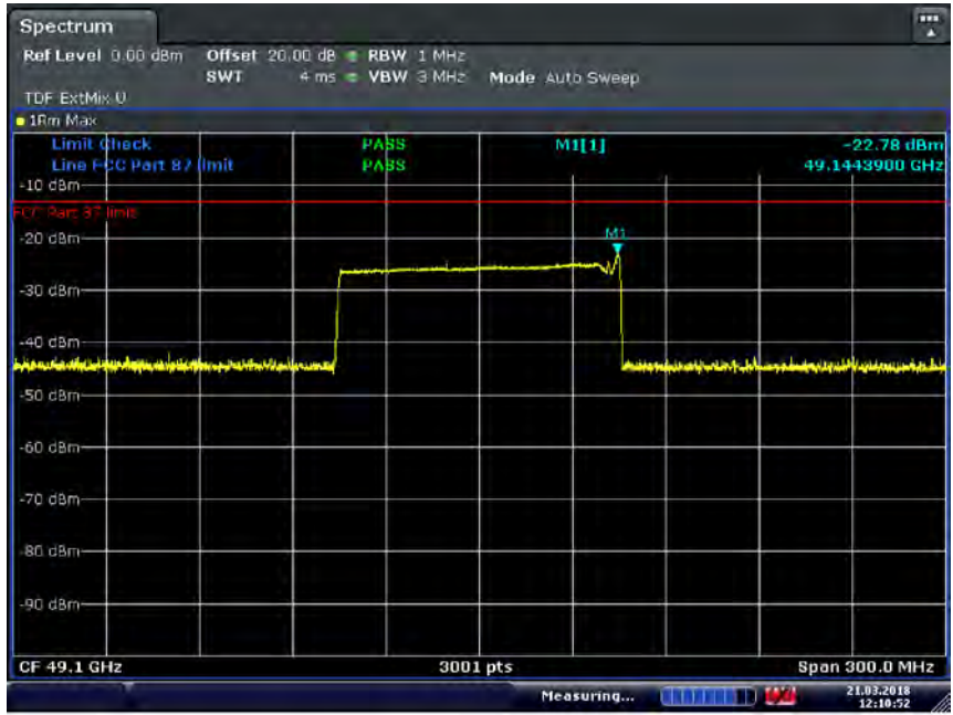
Figure 8.5.8: Zoom @ 49.1 GHz (Mid channel, 24.55 GHz)
