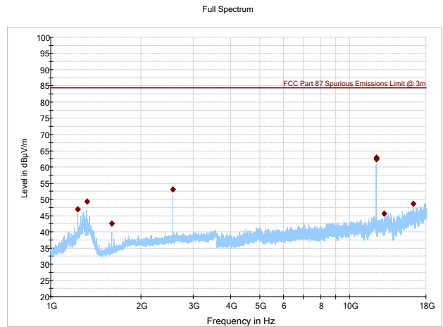
Figure 8.6.6: Radiated spurious emissions, 1-18 GHz Mid Channel
