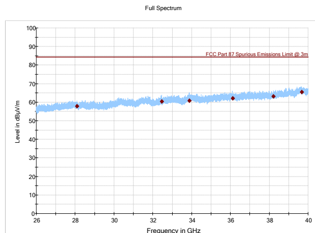
Figure 8.6.4: Radiated spurious emissions, 26-40 GHz Low Channel
