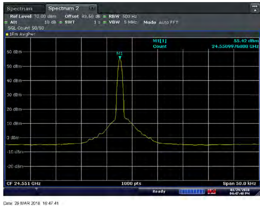
Figure 8.4-1: -45°C (Nominal Voltage)
