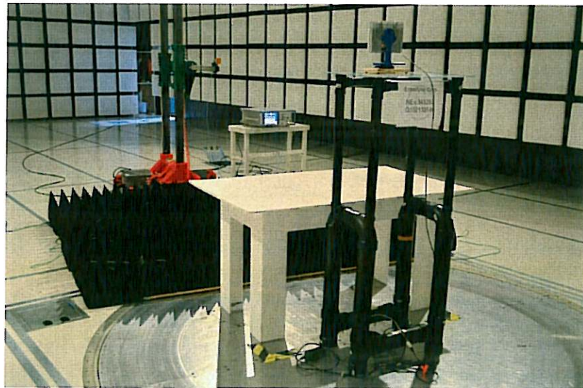
Figure 3.6-6: Radiated Emissions Test Setup – 18-40 GHz (Back)
