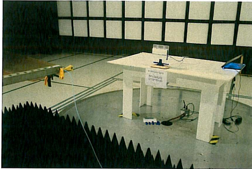
Figure 3.6-7: Radiated Emissions Test Setup – 40-75 GHz (Front)
