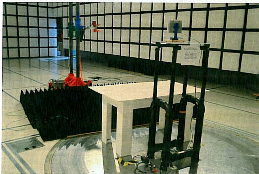
Figure 3.6-4: Radiated Emissions Test Setup – 1-18 GHz (Back)
