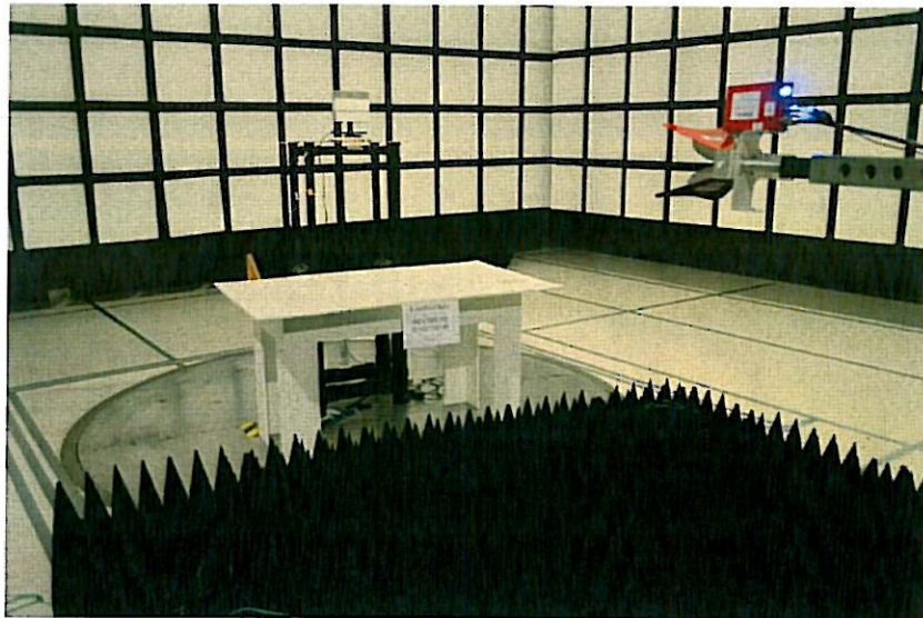
Figure 3.6-3: Radiated Emissions Test Setup – 1-18 GHz (Front)
