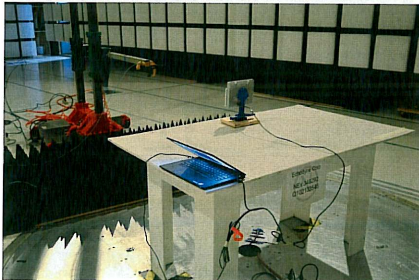
Figure 3.6-8: Radiated Emissions Test Setup – 40-75 GHz (Back)
