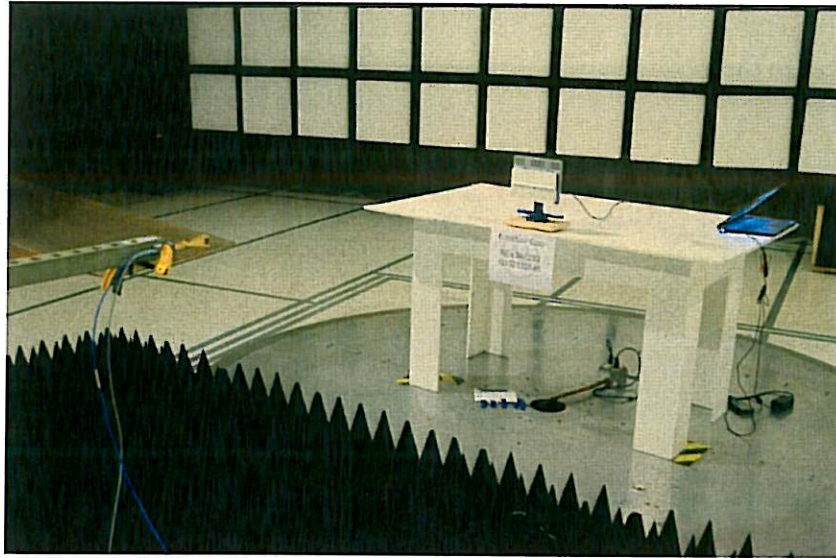
Figure 3.6-9: Radiated Emissions Test Setup – 75-110 GHz (Front)
