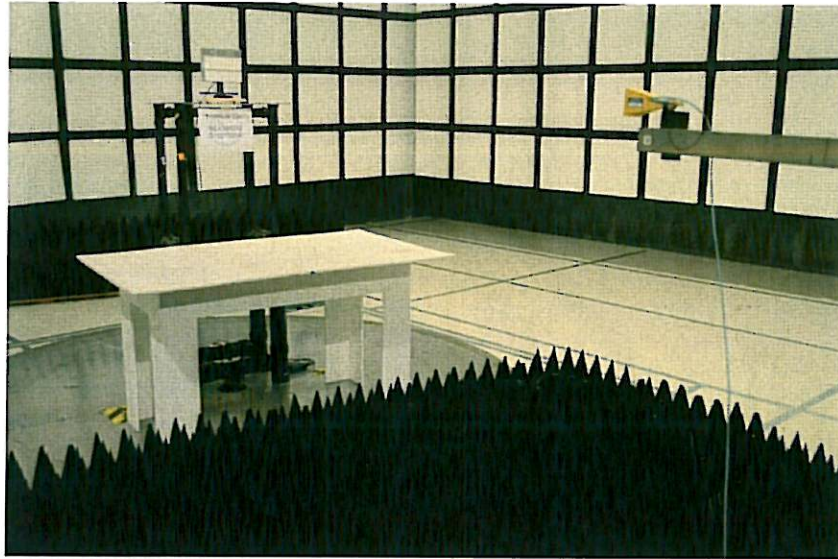
Figure 3.6-5: Radiated Emissions Test Setup – 18-40 GHz (Front)
