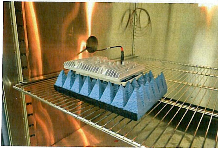
Figure 3.6-11: Frequency stability setup
