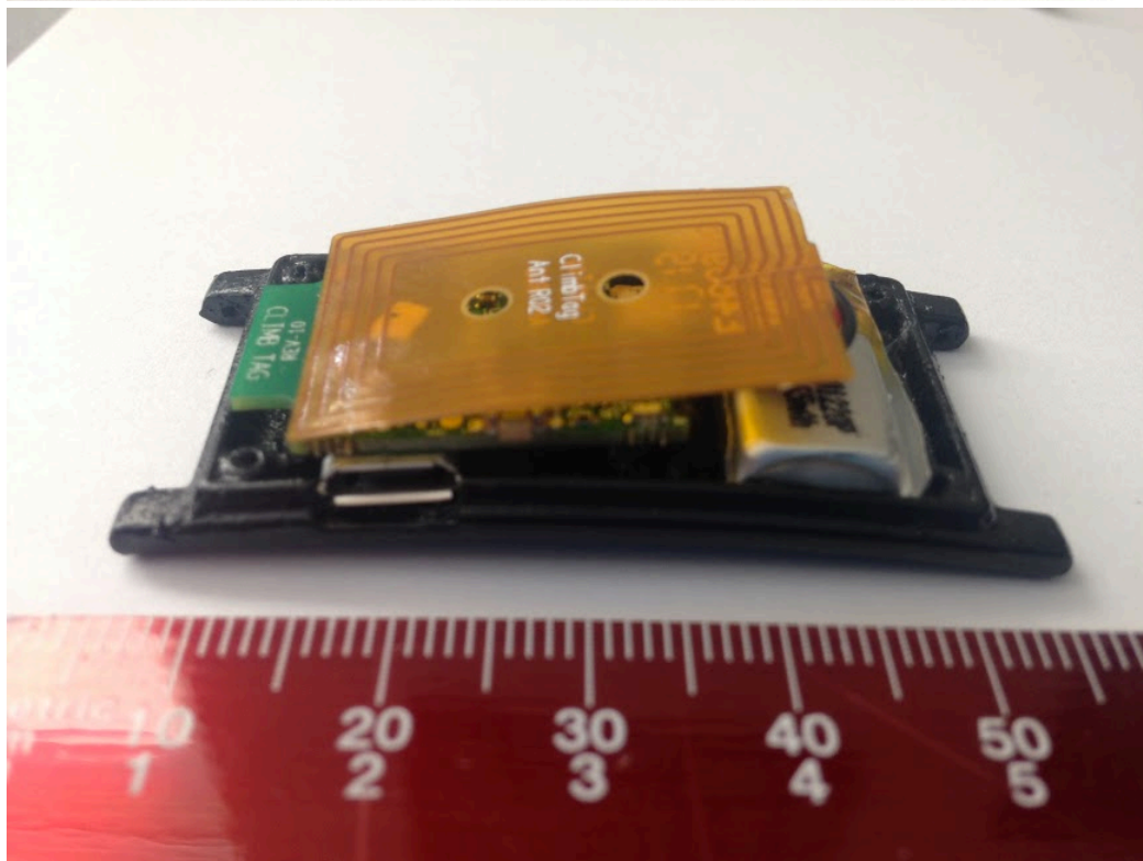
Fully assembled unit, with flexible antenna connected
