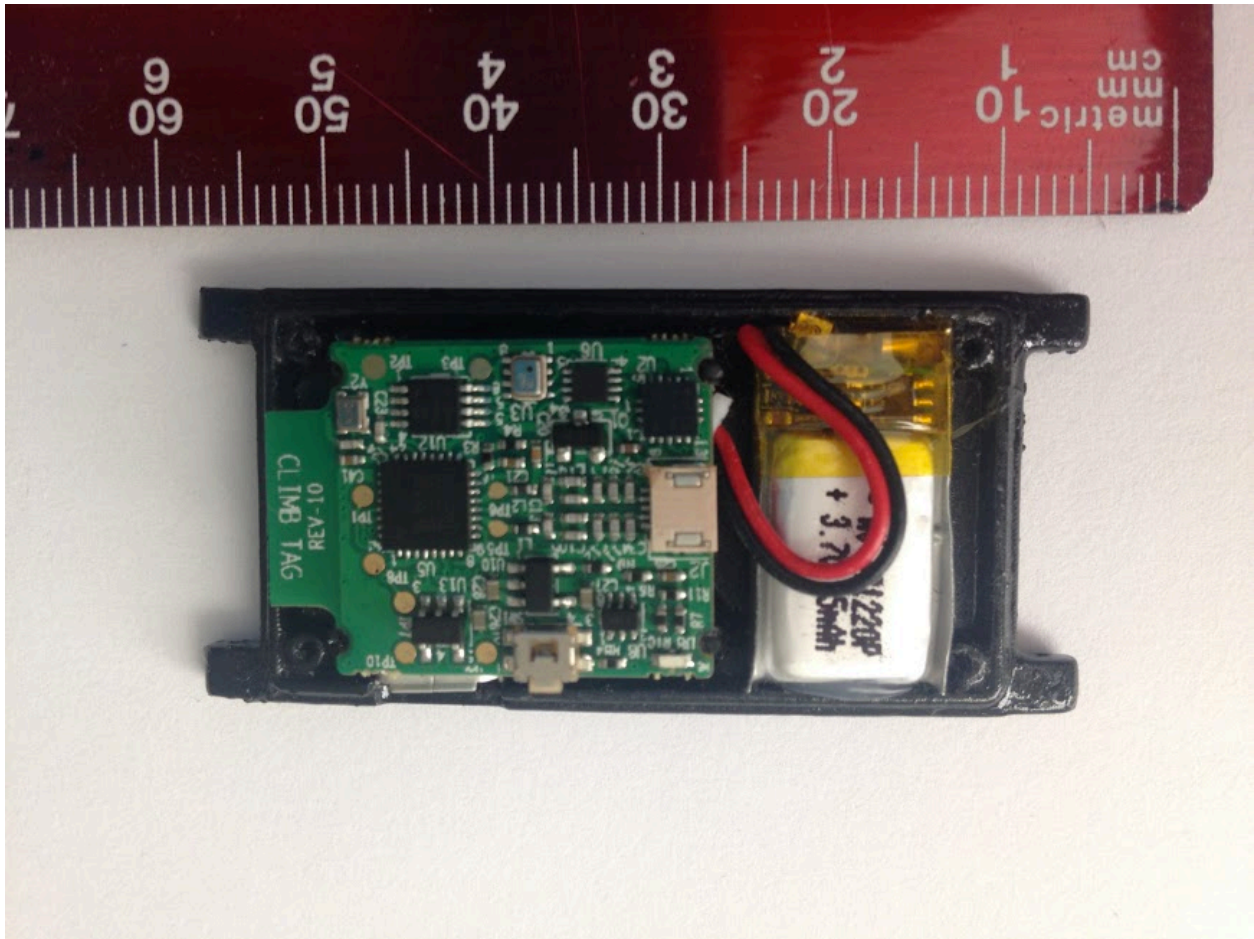
Circuit board and battery in housing
