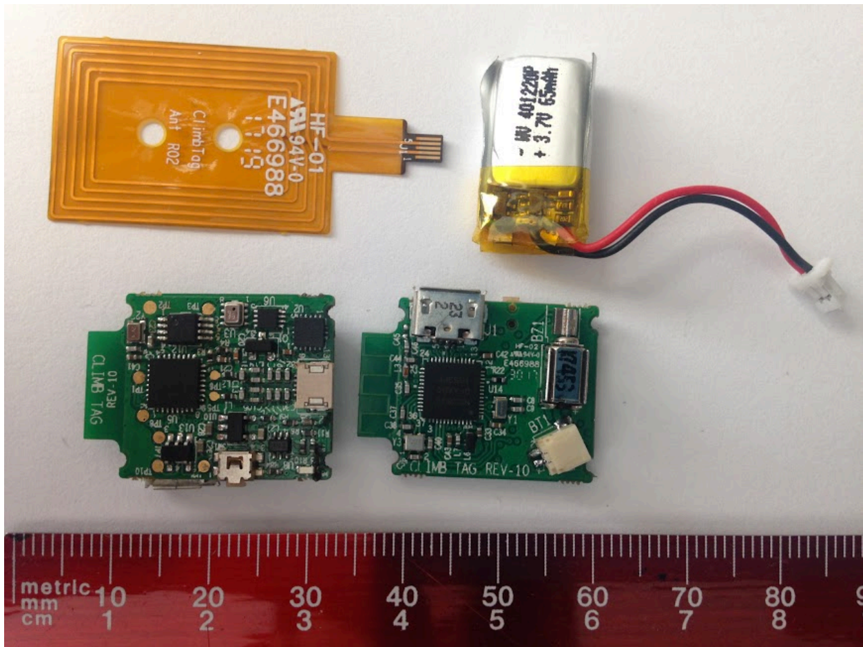
Photo showing the board from sides, the external flexible 13.56MHz antenna and battery.
