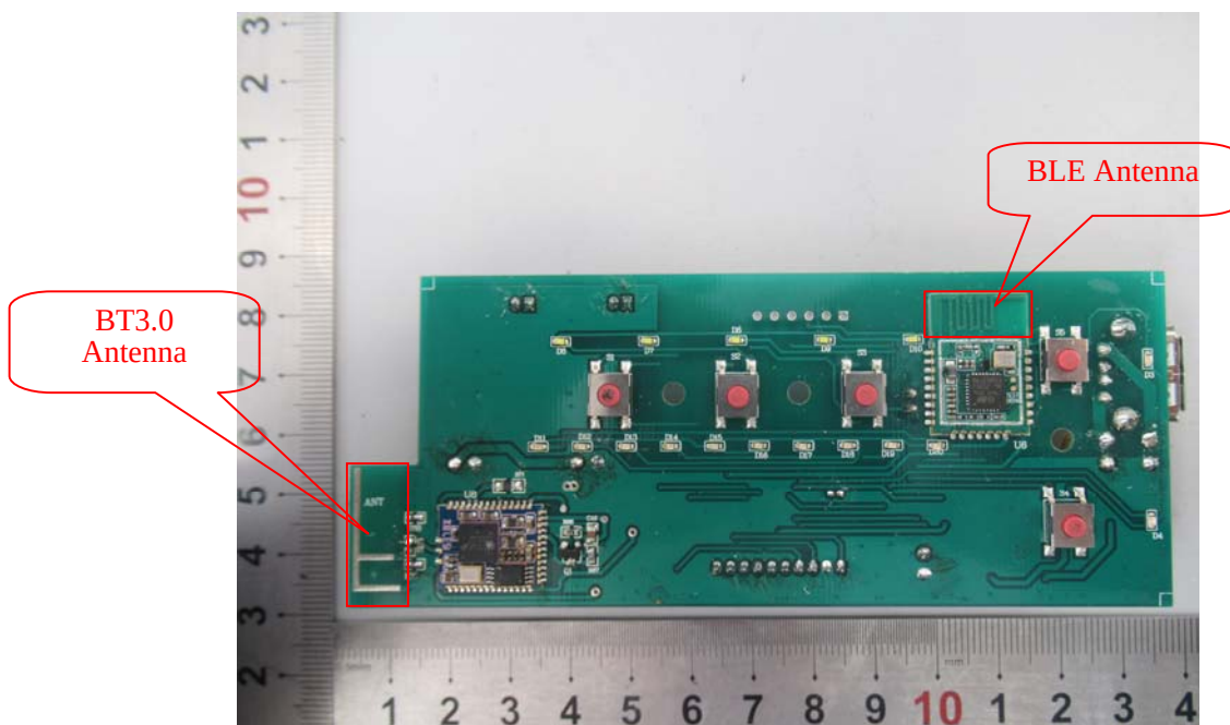
EUT – PCB-1 Bottom Shielding off View
