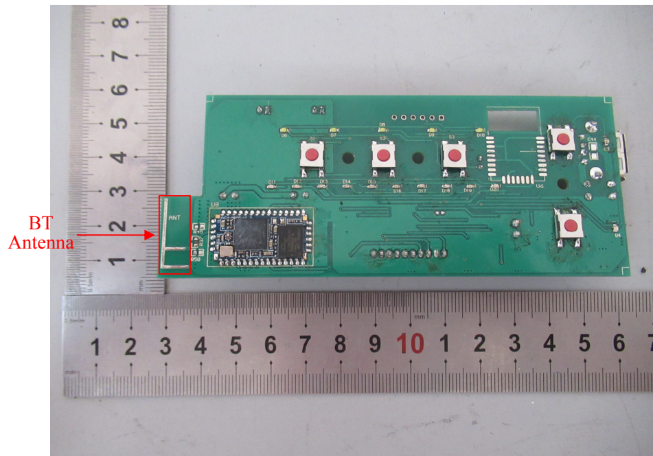
EUT – PCB-1 Bottom Chip View
