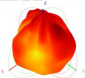
5750.0MHz H+V, Eff: 40.5%
