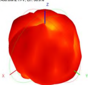
2450.0MHz H+V, Eff: 50.0%
