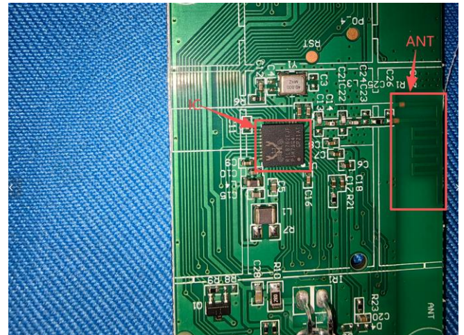
IC and Antenna
