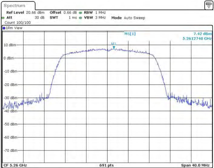
11AC20SISO_Ant2_5260
