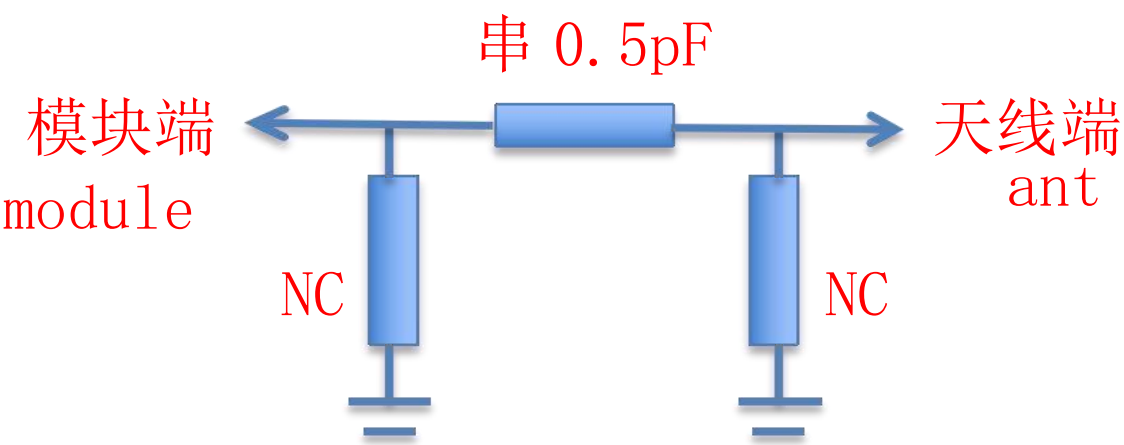
5: Antenna Matching Circuit Diagram
